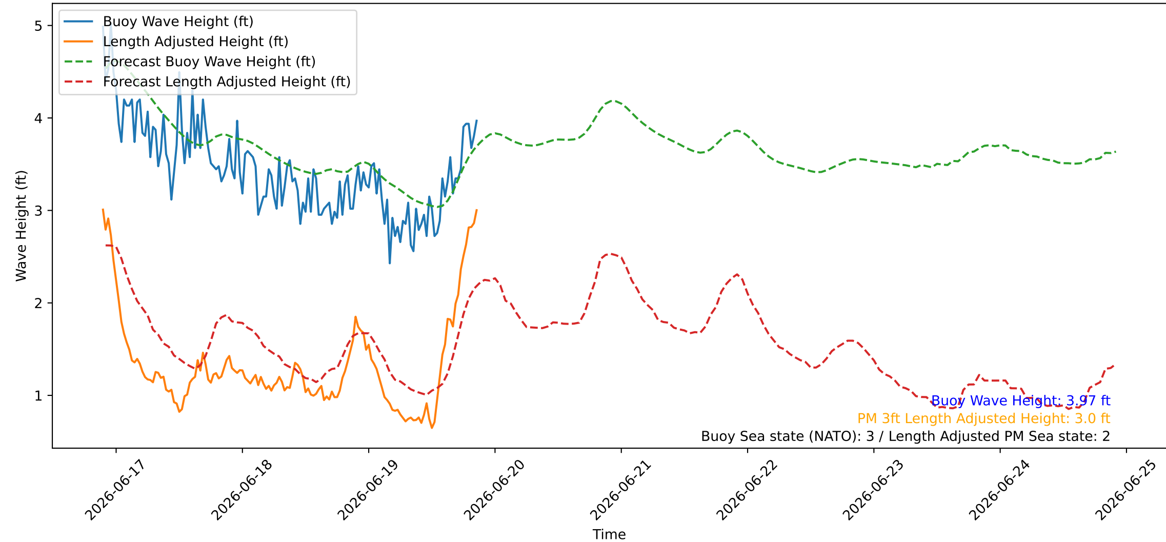
Wave Heights over Time for Green Beach at 2026-06-19 21:31:07
