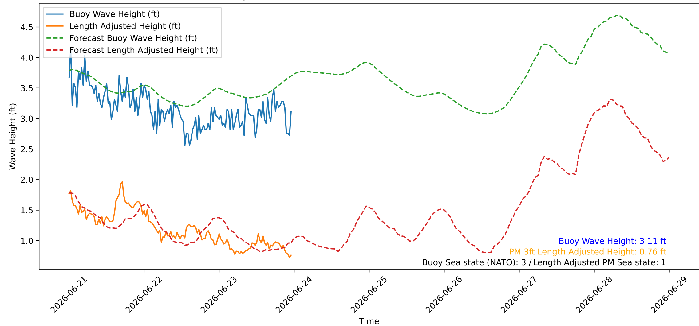
Wave Heights over Time for Oceanside Harbor at 2026-06-24 00:00:26
