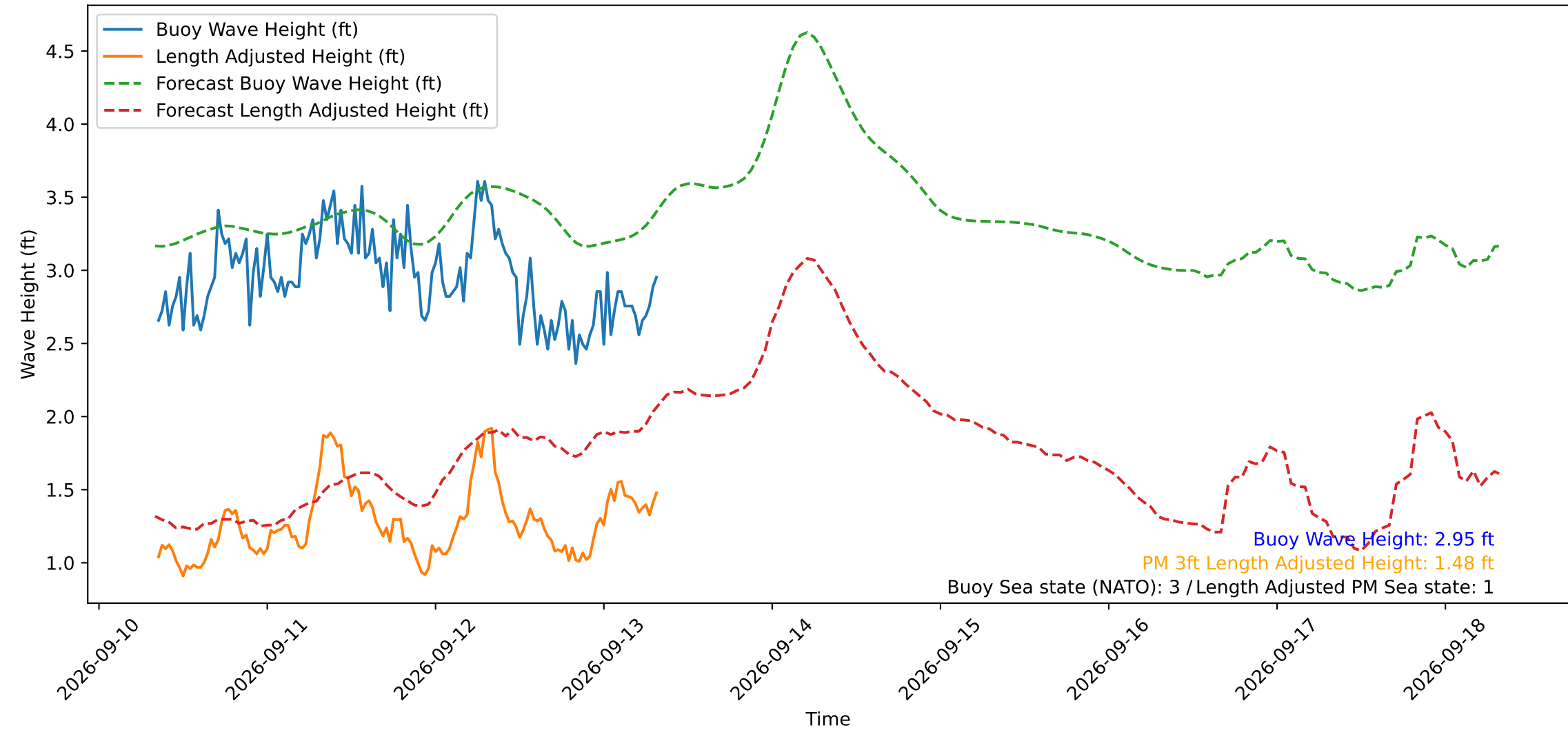
Wave Heights over Time for Green Beach at 2026-09-13 08:11:11
