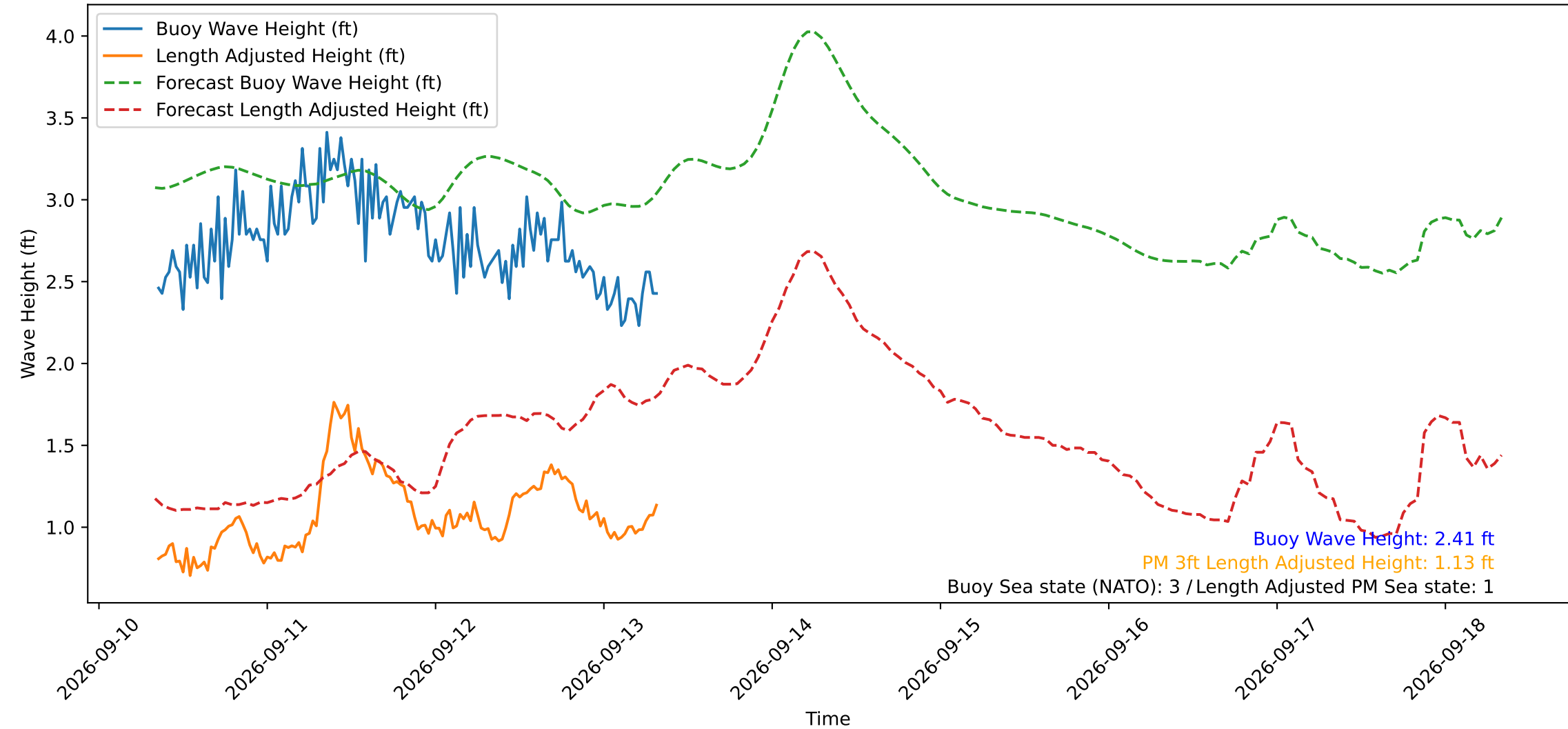
Wave Heights over Time for Red Beach at 2026-09-13 08:10:49
