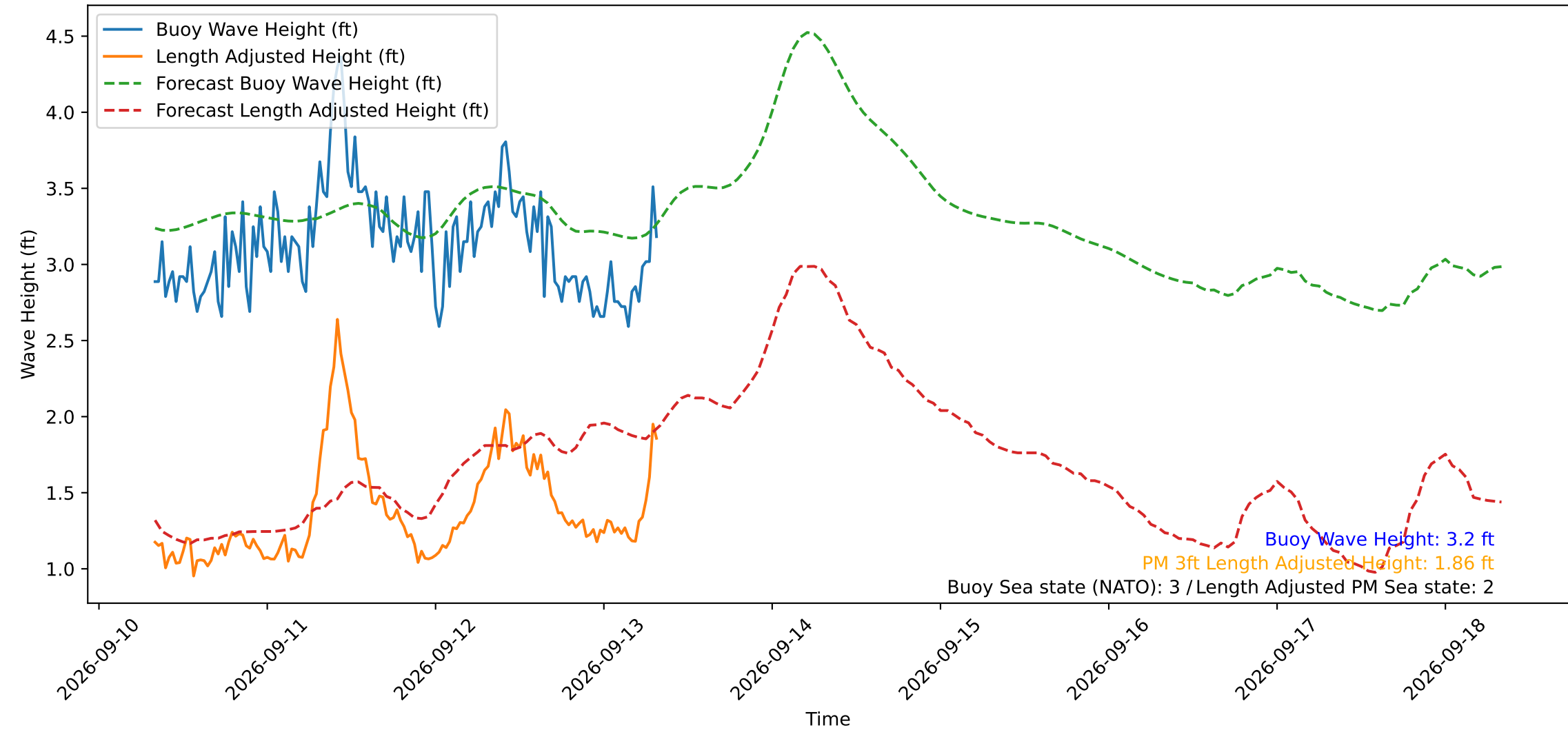
Wave Heights over Time for Oceanside Harbor at 2026-09-13 08:10:30
