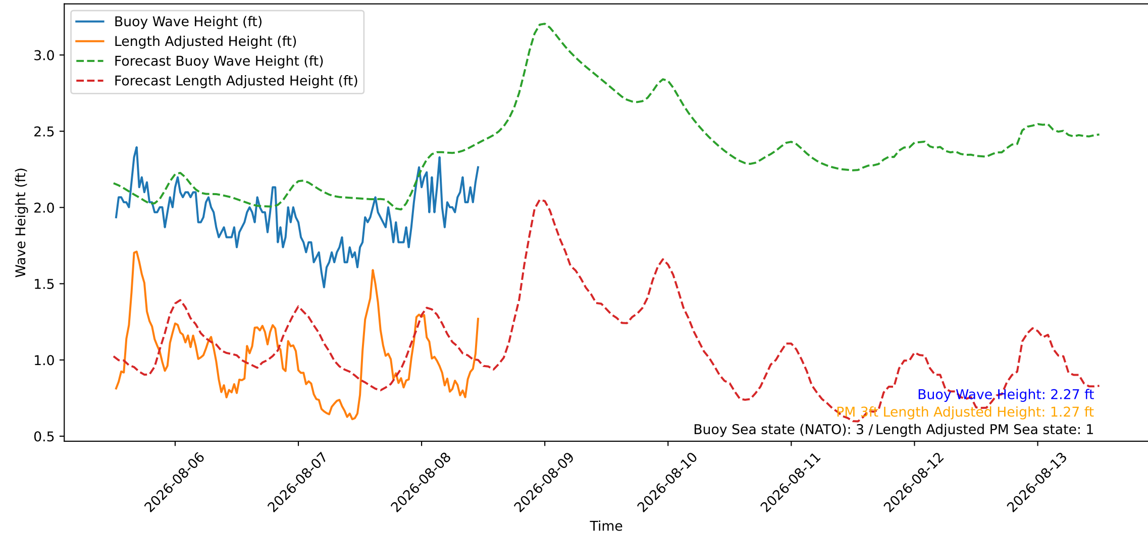
Wave Heights over Time for Red Beach at 2026-08-08 12:00:46
