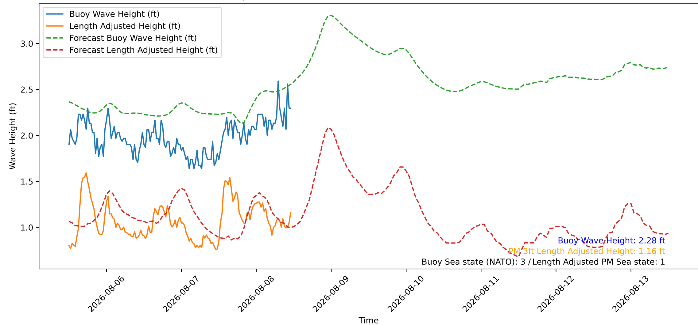
Wave Heights over Time for Oceanside Harbor at 2026-08-08 12:00:26
