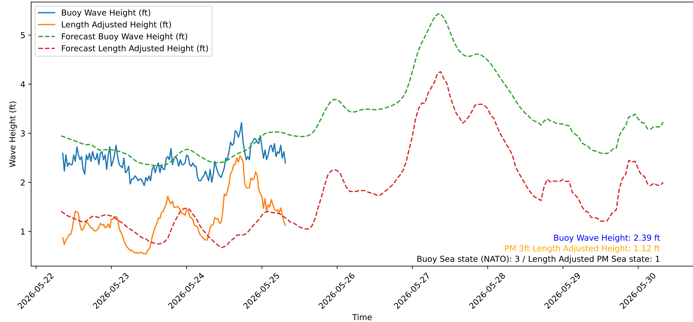
Wave Heights over Time for Red Beach at 2026-05-25 08:20:52
