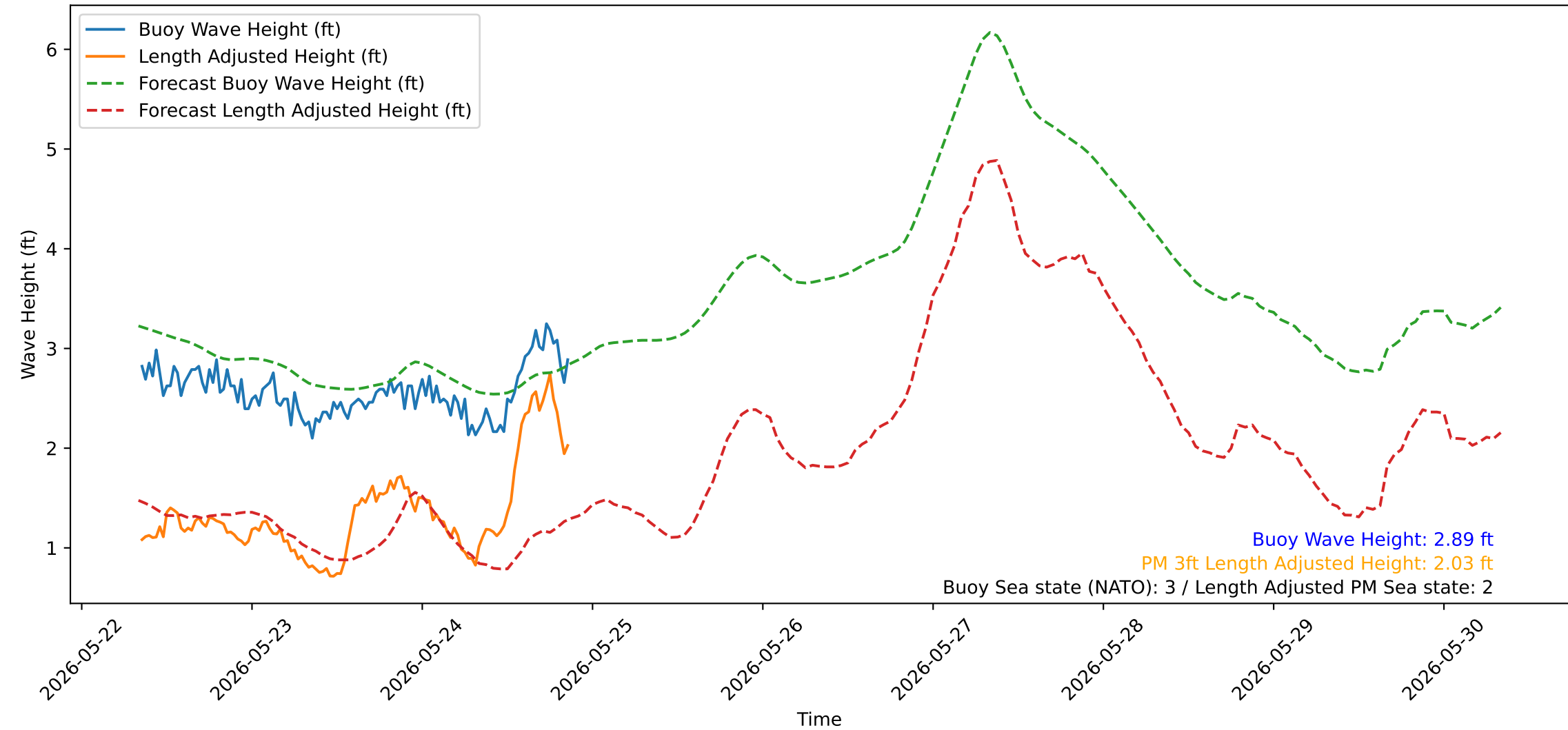
Wave Heights over Time for Oceanside Harbor at 2026-05-25 08:20:31
