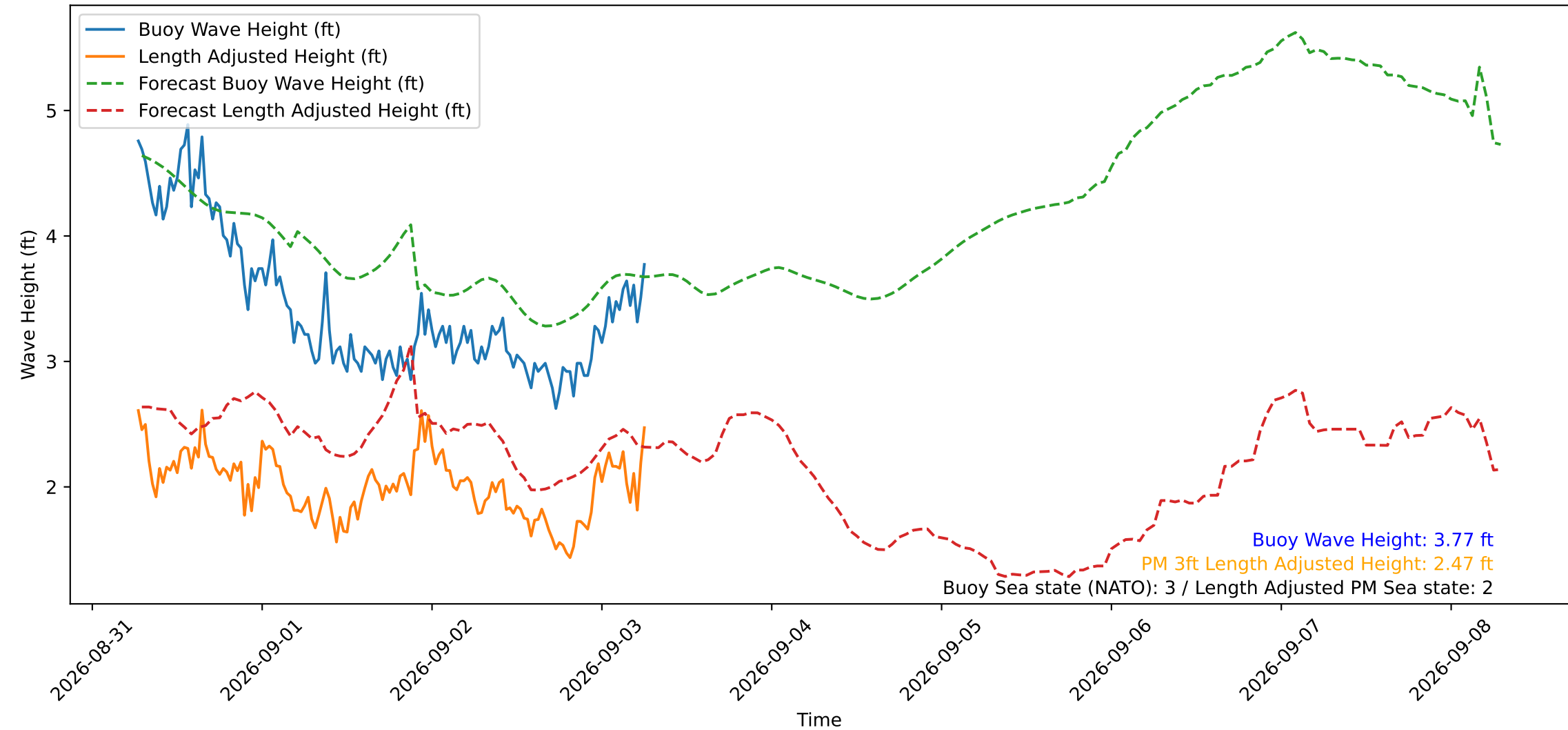
Wave Heights over Time for Oceanside Harbor at 2026-09-03 06:40:29
