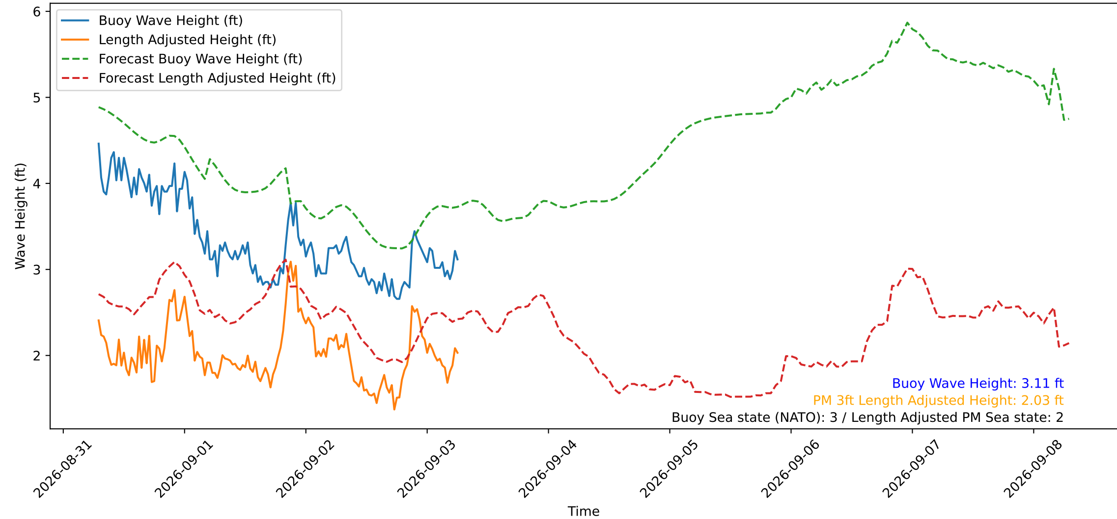
Wave Heights over Time for Green Beach at 2026-09-03 06:41:12
