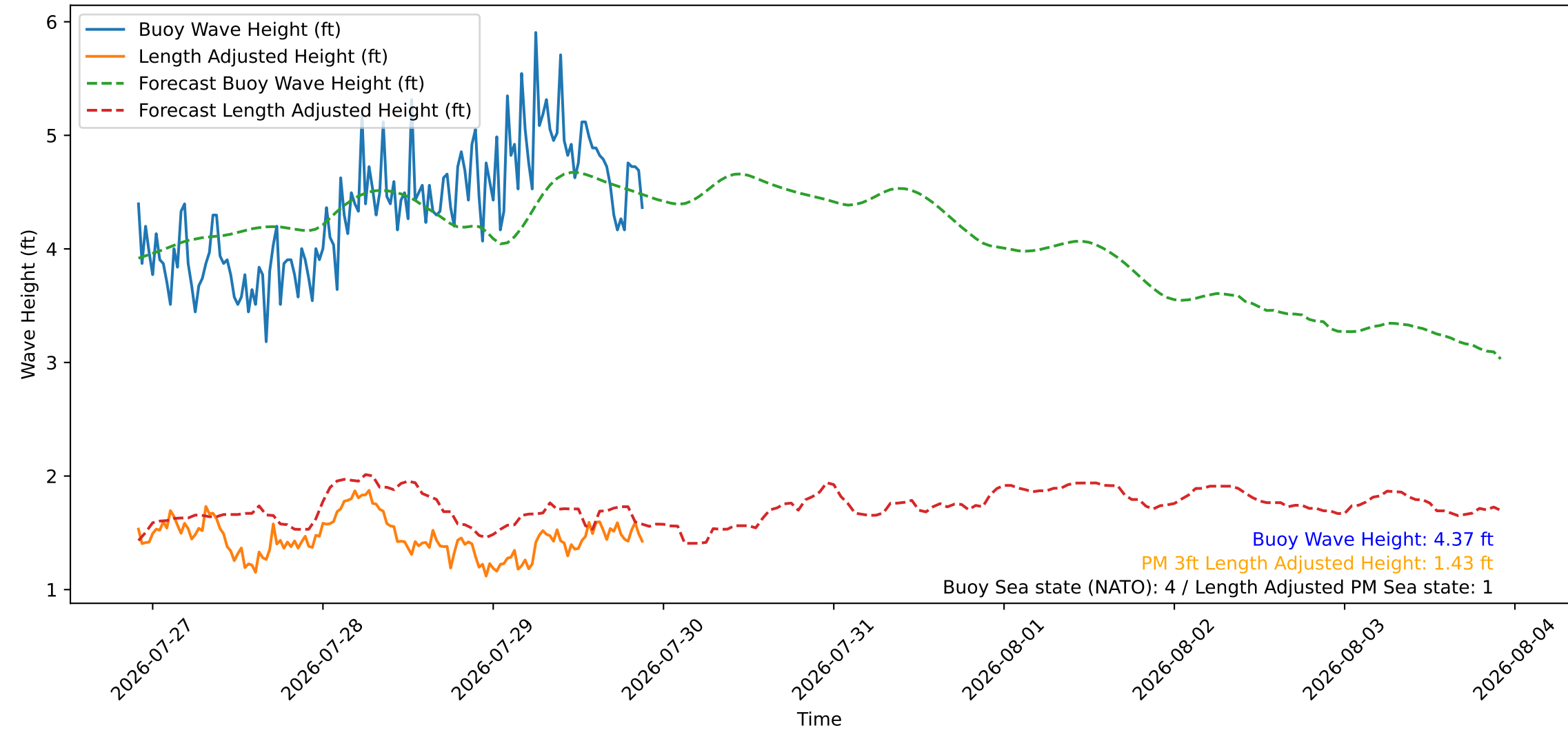
Wave Heights over Time for Oceanside Harbor at 2026-07-29 21:50:27
