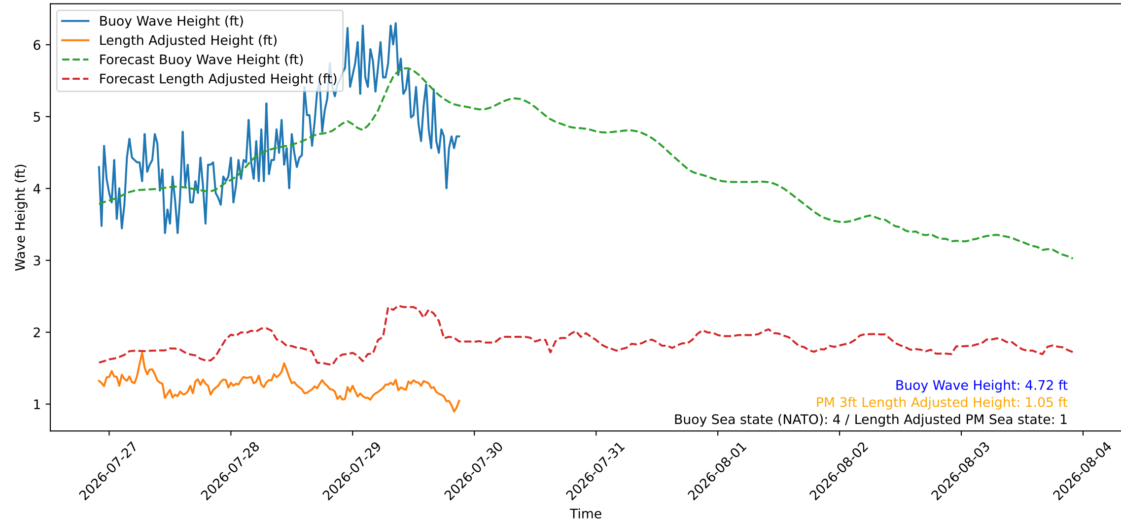
Wave Heights over Time for Green Beach at 2026-07-29 21:51:10
