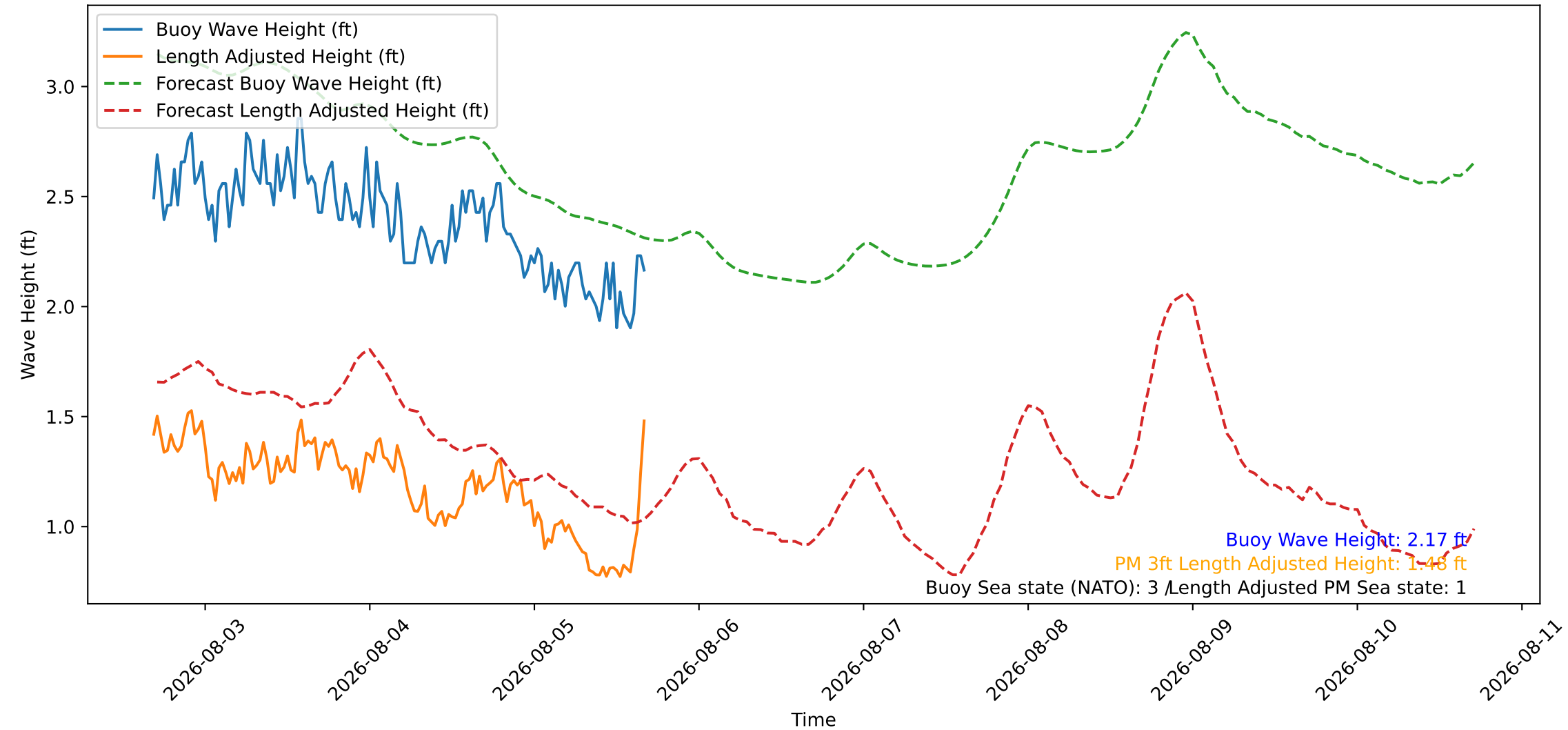
Wave Heights over Time for Oceanside Harbor at 2026-08-05 16:40:26
