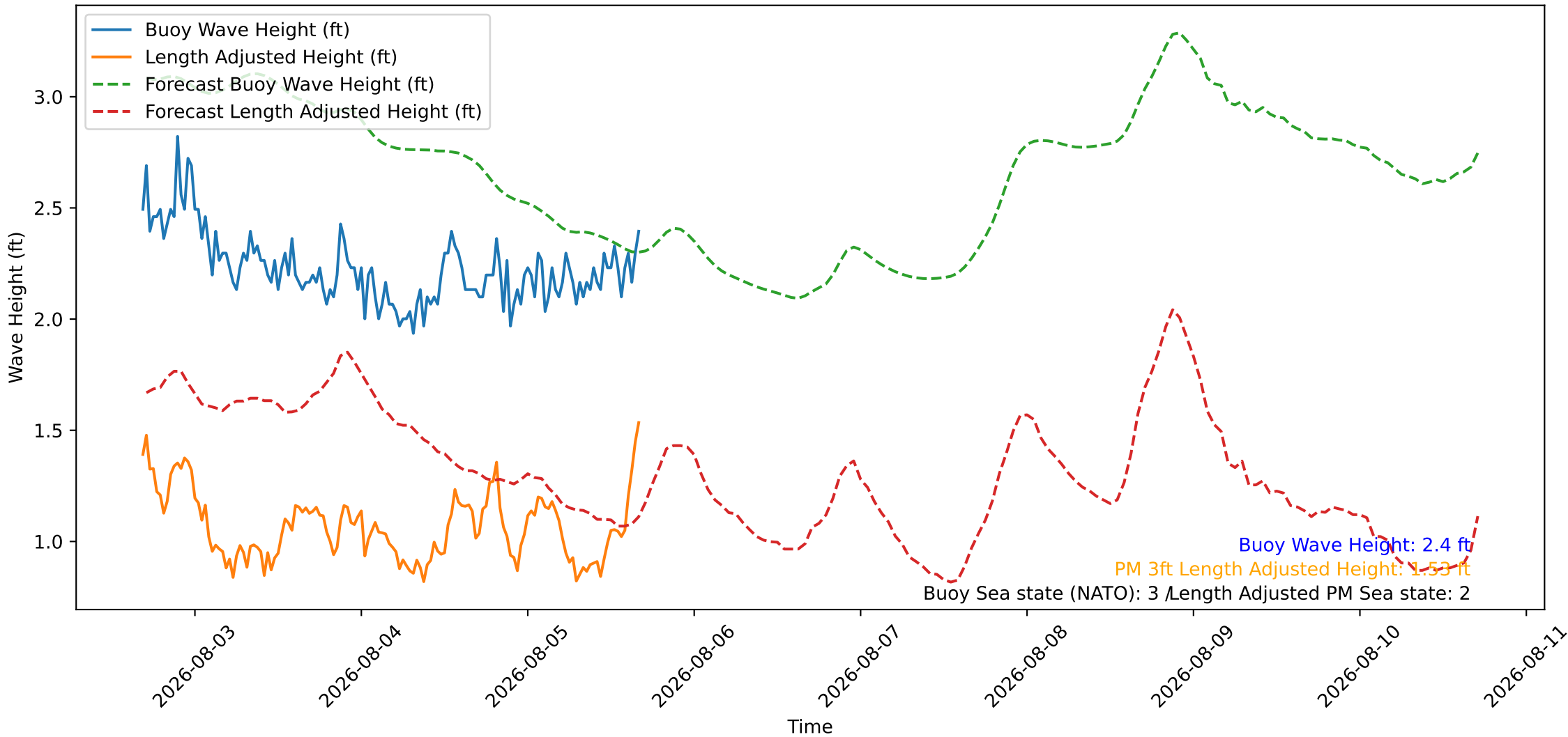
Wave Heights over Time for Green Beach at 2026-08-05 16:41:09
