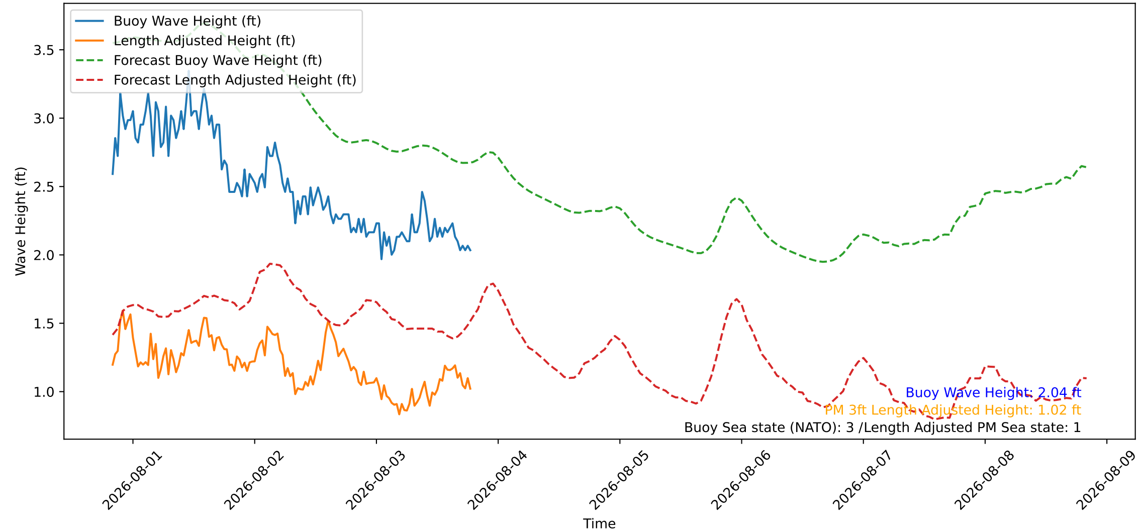
Wave Heights over Time for Red Beach at 2026-08-03 19:30:46
