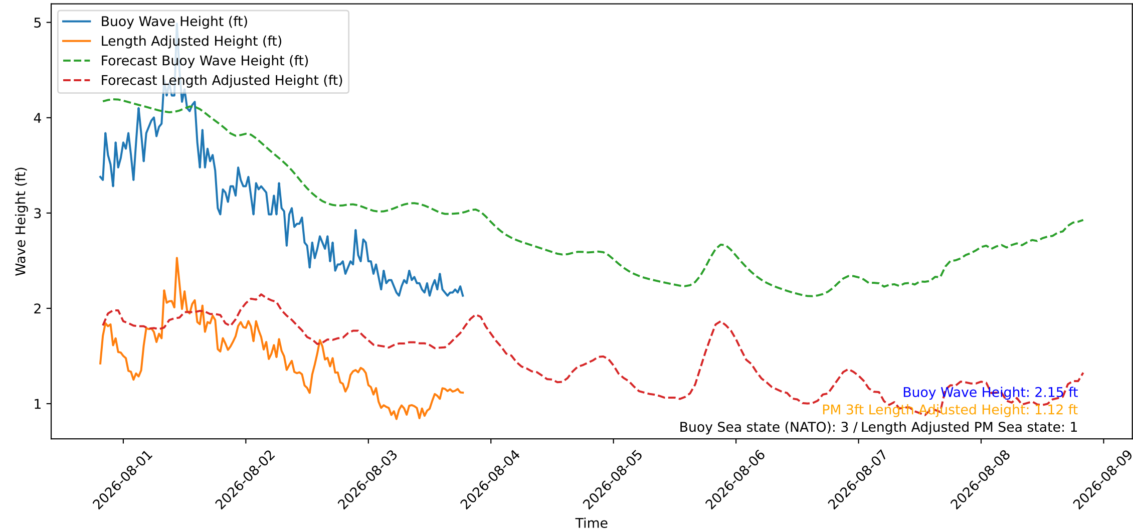
Wave Heights over Time for Green Beach at 2026-08-03 19:31:08
