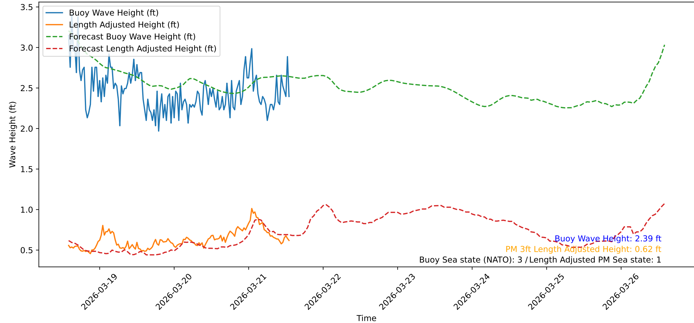
Wave Heights over Time for Oceanside Harbor at 2026-03-21 13:50:31
