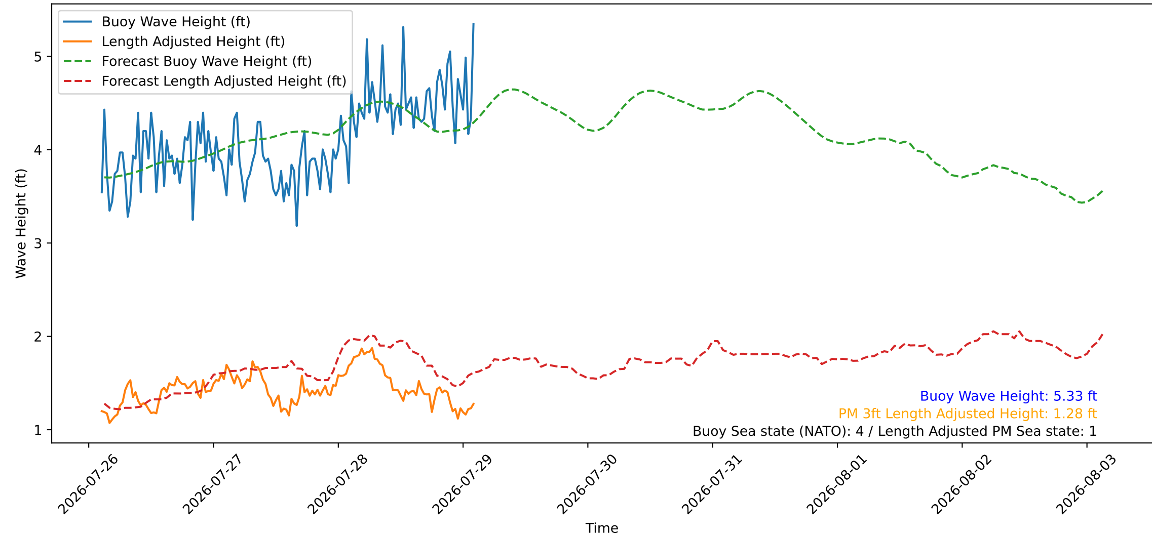
Wave Heights over Time for Oceanside Harbor at 2026-07-29 02:40:27
