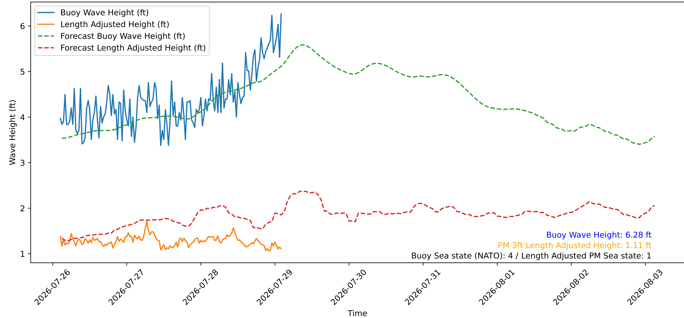
Wave Heights over Time for Green Beach at 2026-07-29 02:41:10
