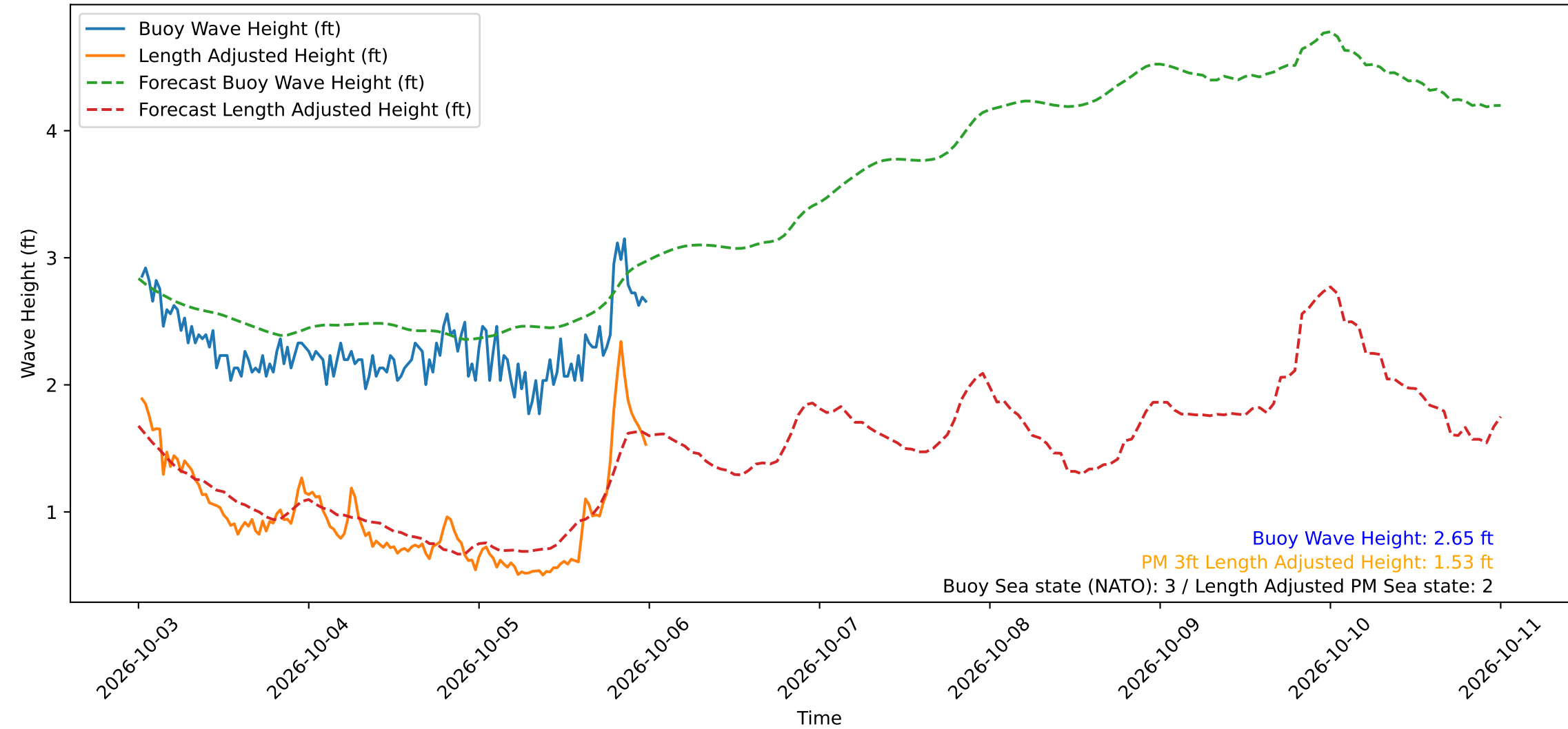
Wave Heights over Time for Green Beach at 2026-10-06 00:21:14
