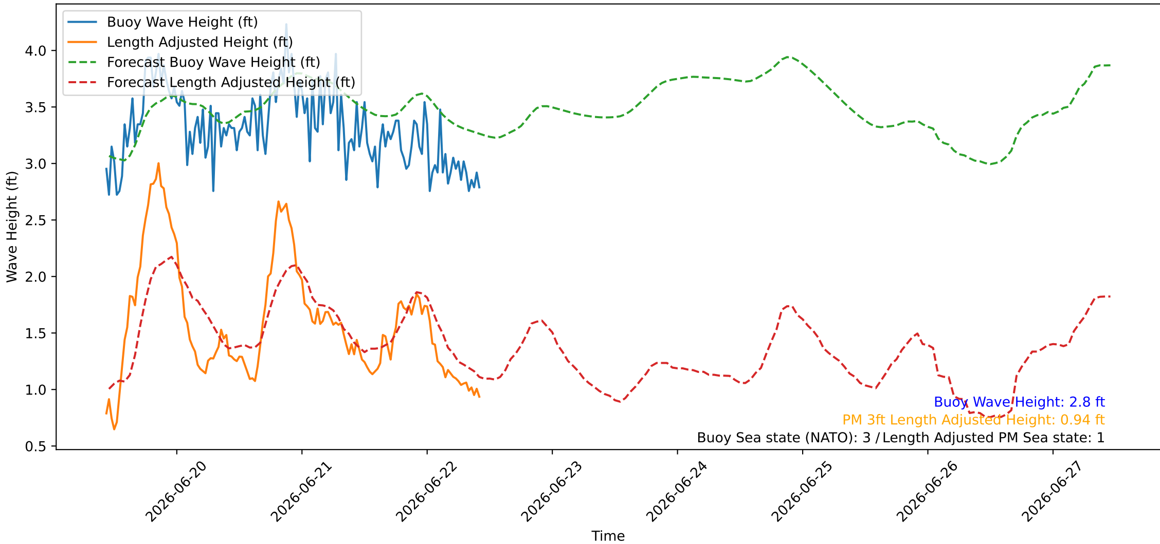
Wave Heights over Time for Green Beach at 2026-06-22 10:41:08
