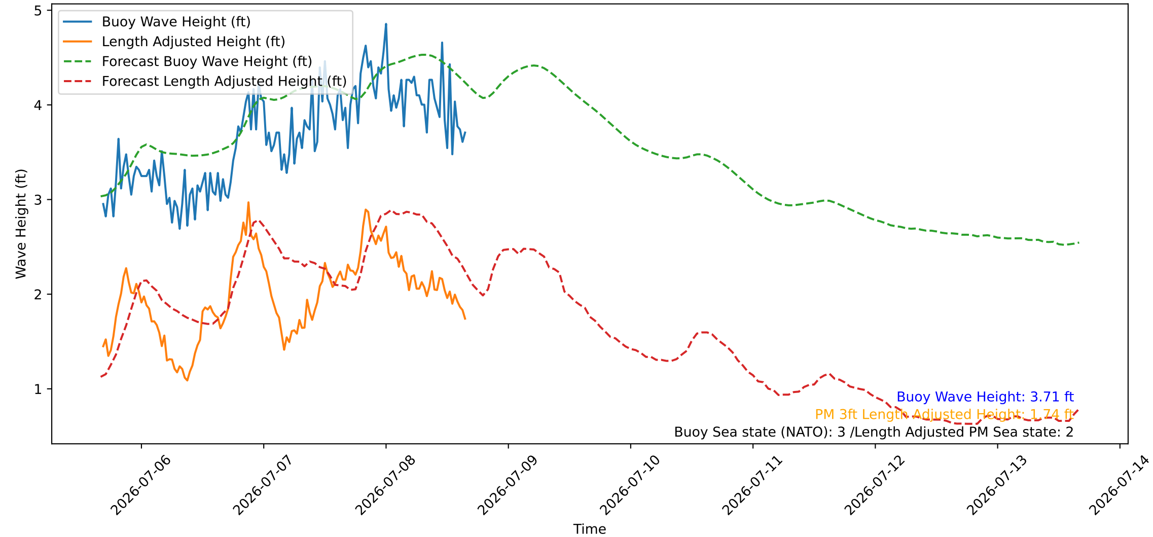
Wave Heights over Time for Red Beach at 2026-07-08 16:20:47
