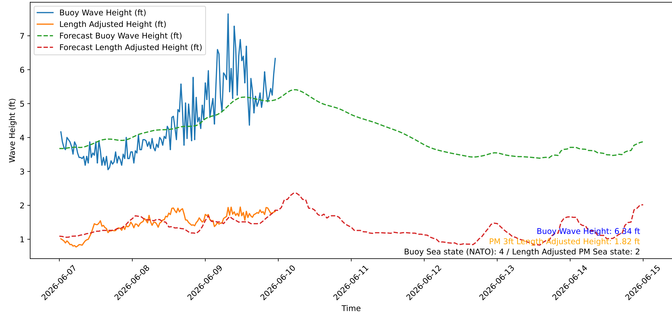
Wave Heights over Time for Red Beach at 2026-06-10 00:00:47
