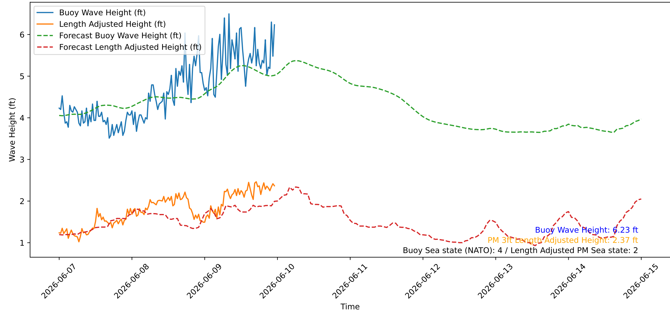
Wave Heights over Time for Oceanside Harbor at 2026-06-10 00:00:27
