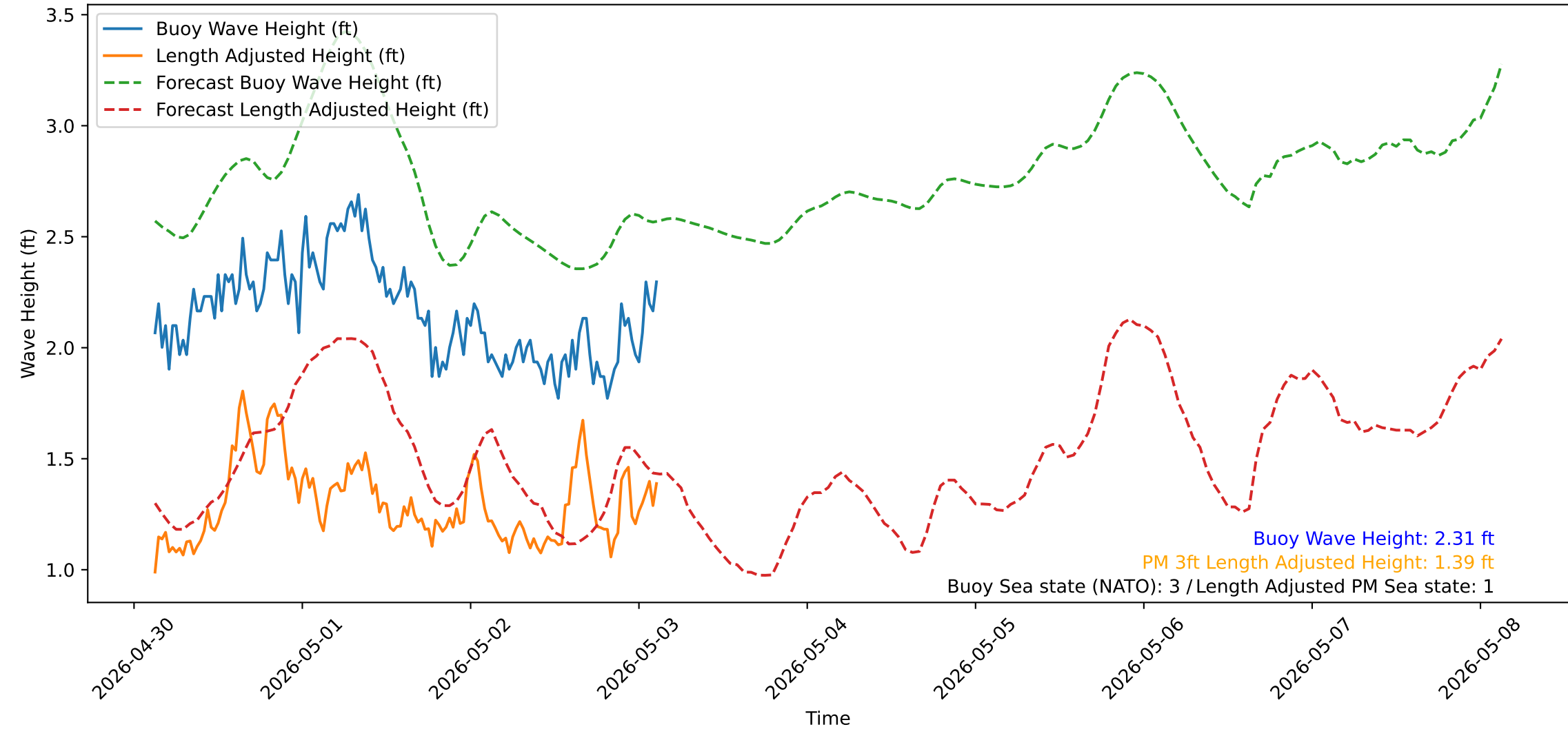
Wave Heights over Time for Oceanside Harbor at 2026-05-03 03:10:31
