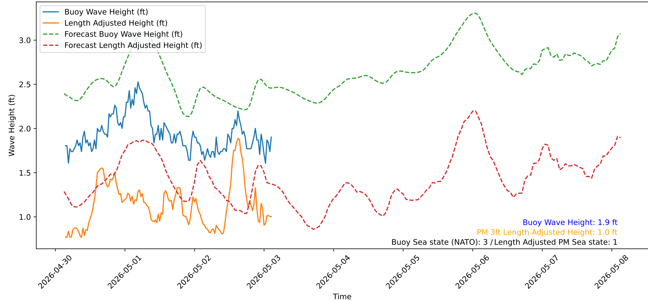
Wave Heights over Time for Red Beach at 2026-05-03 03:10:50
