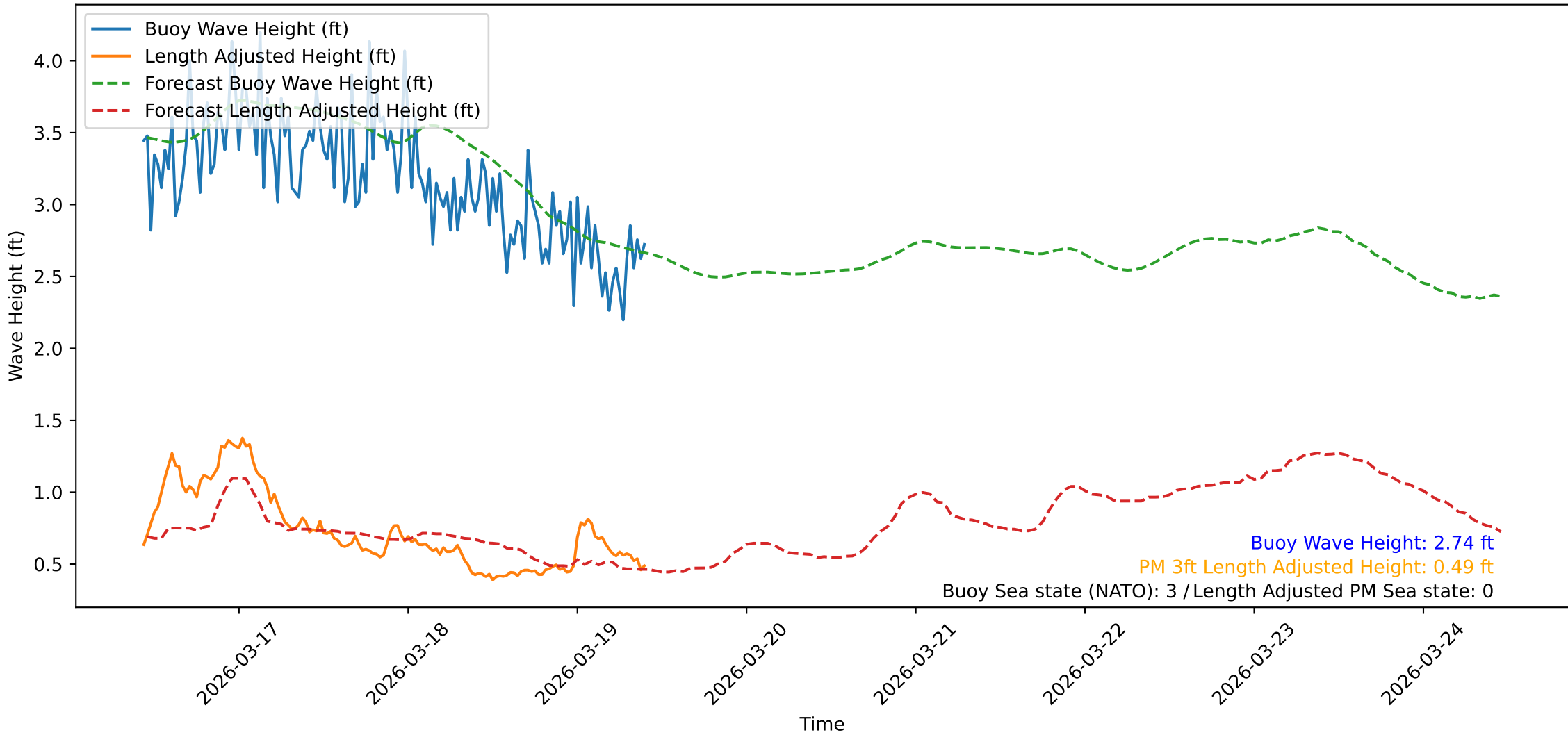
Wave Heights over Time for Green Beach at 2026-03-19 10:31:10
