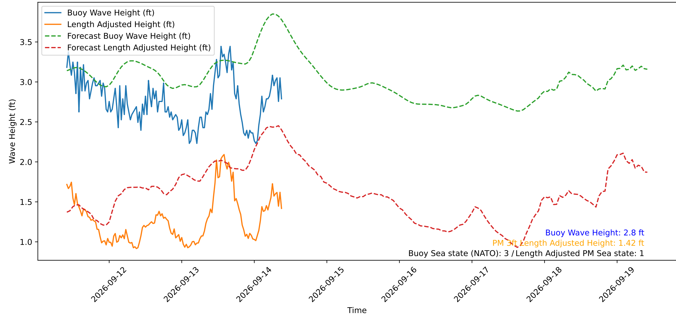
Wave Heights over Time for Red Beach at 2026-09-14 09:50:50
