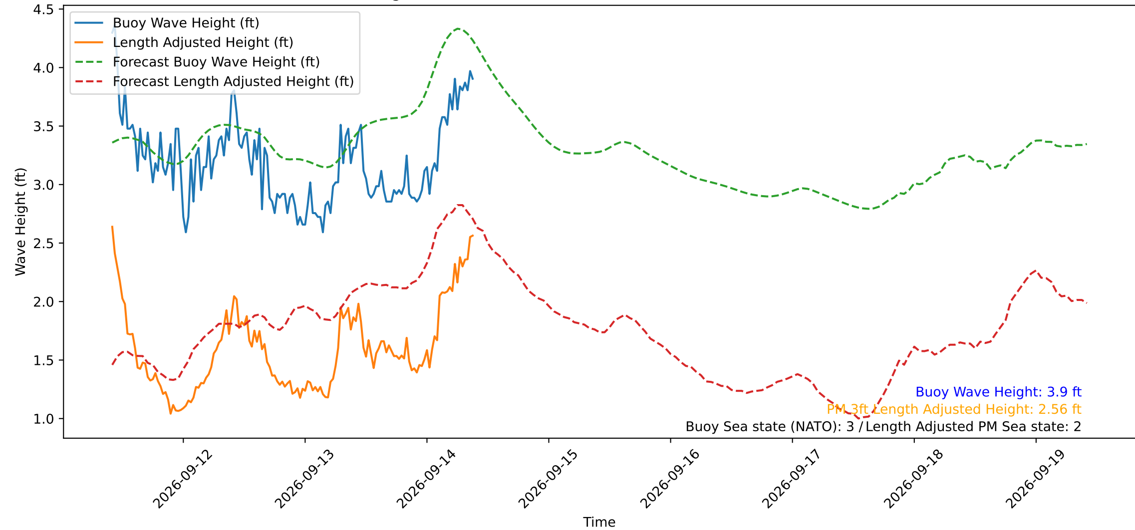
Wave Heights over Time for Oceanside Harbor at 2026-09-14 09:50:29
