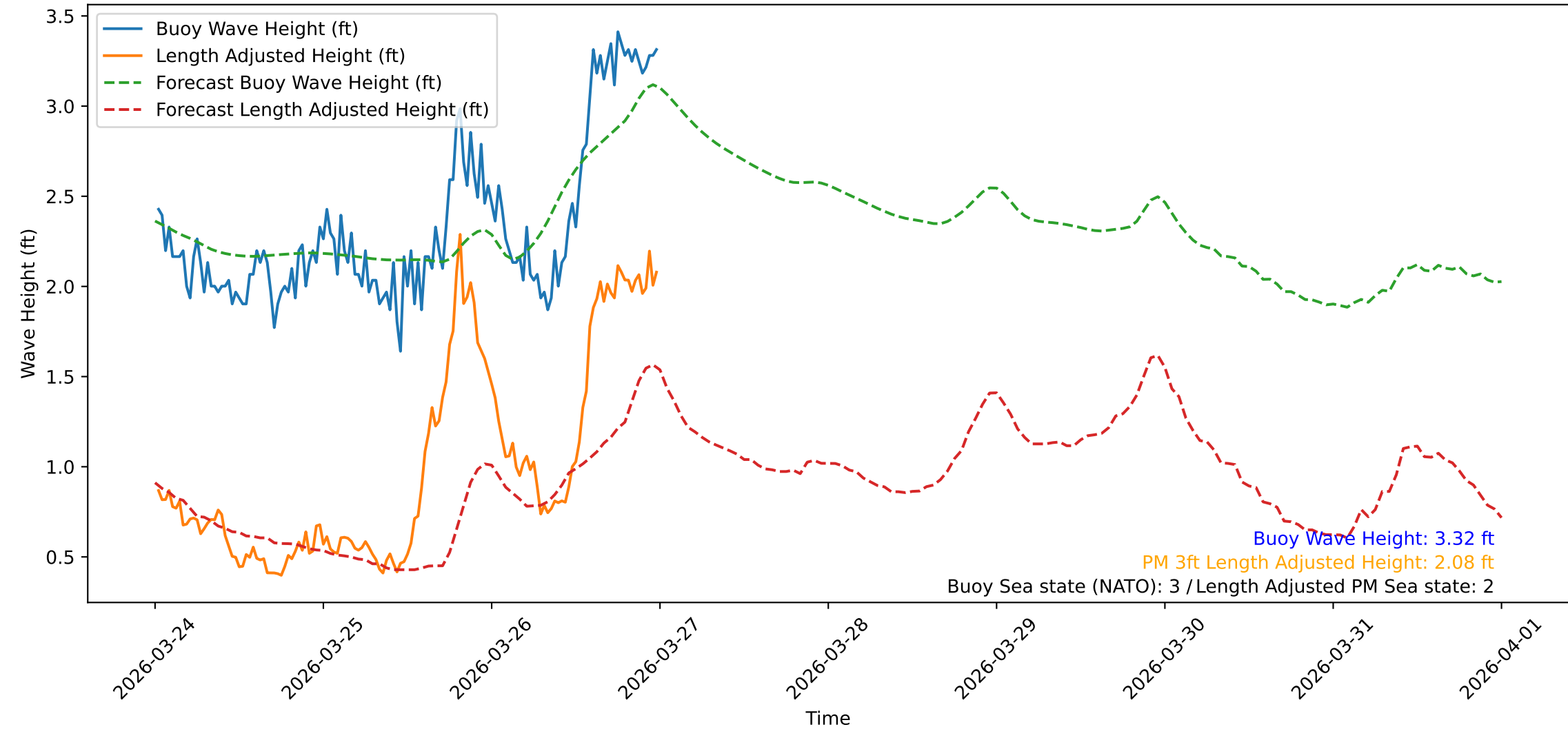
Wave Heights over Time for Green Beach at 2026-03-27 00:21:09
