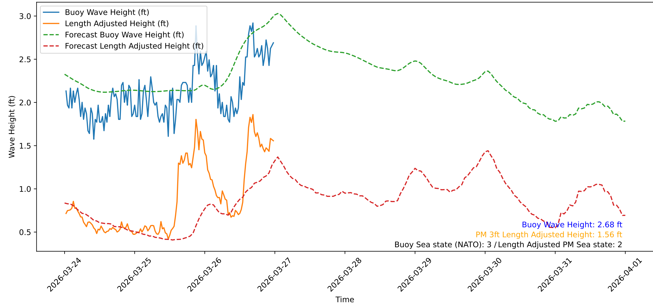
Wave Heights over Time for Oceanside Harbor at 2026-03-27 00:20:31
