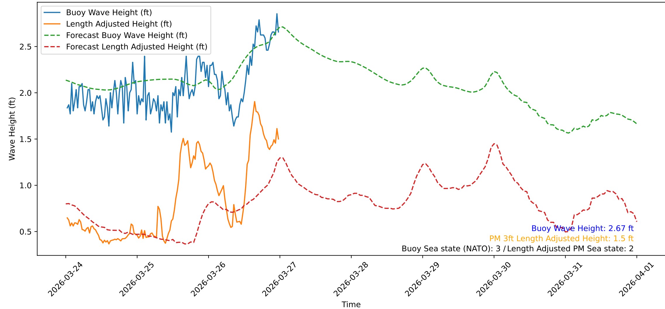
Wave Heights over Time for Red Beach at 2026-03-27 00:20:47
