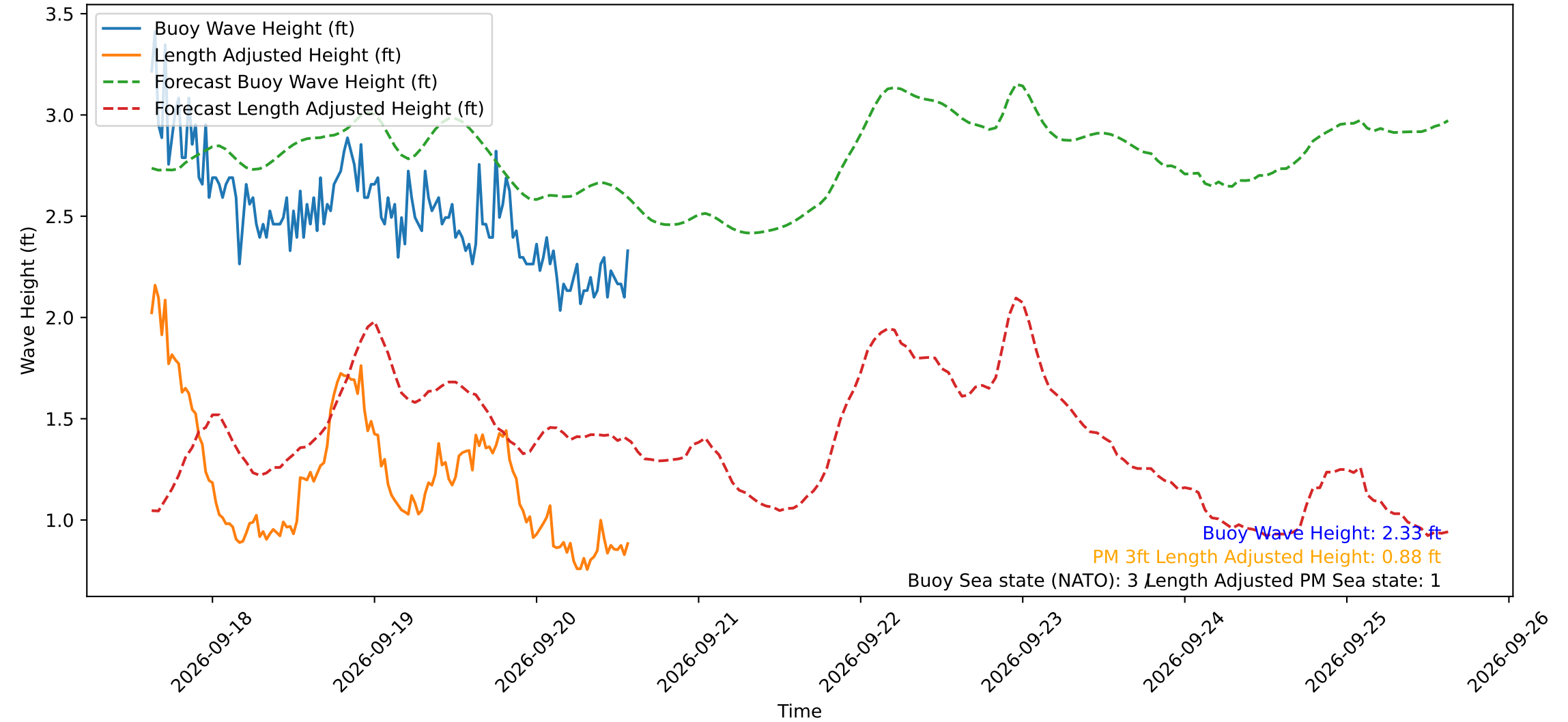
Wave Heights over Time for Red Beach at 2026-09-20 14:40:49
