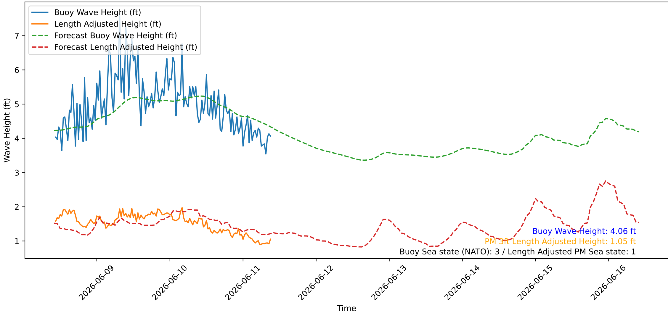
Wave Heights over Time for Red Beach at 2026-06-11 10:00:46
