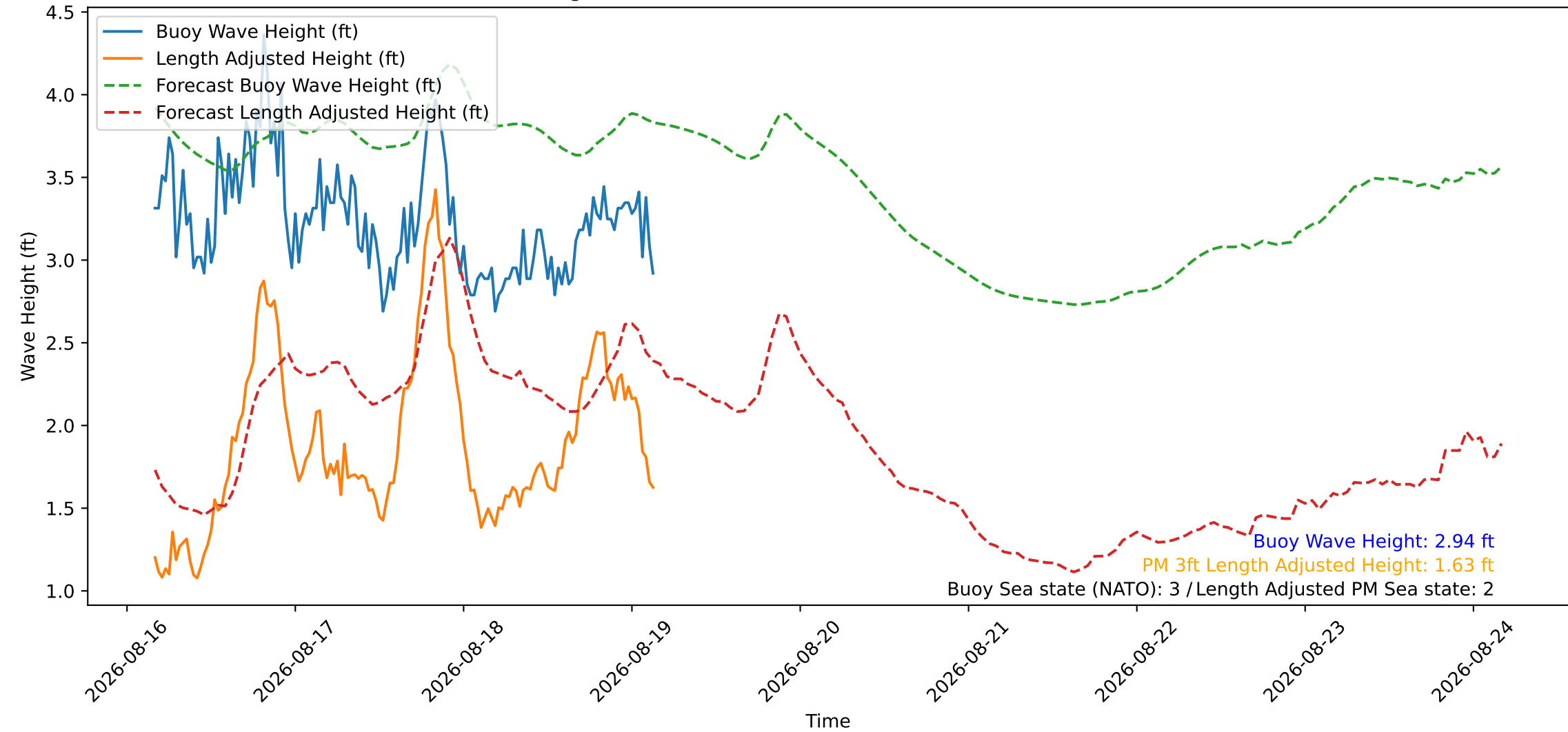
Wave Heights over Time for Green Beach at 2026-08-19 03:51:10
