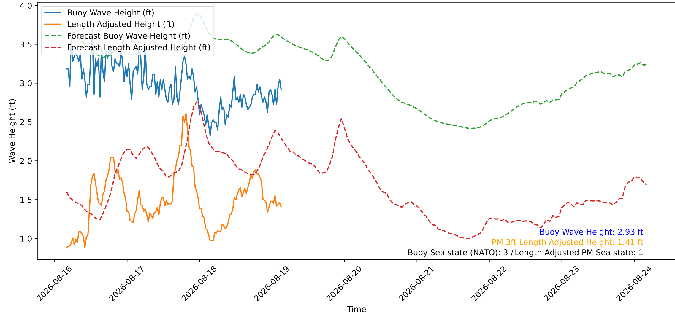
Wave Heights over Time for Red Beach at 2026-08-19 03:50:47
