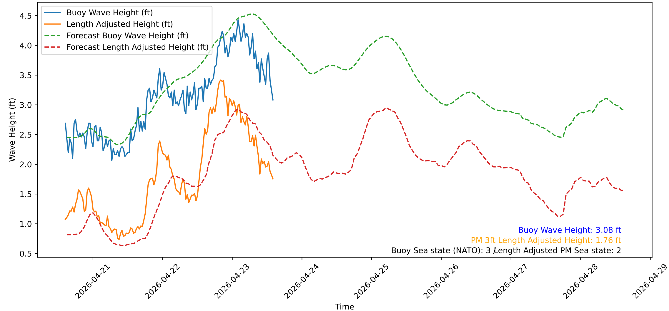
Wave Heights over Time for Oceanside Harbor at 2026-04-23 14:30:31
