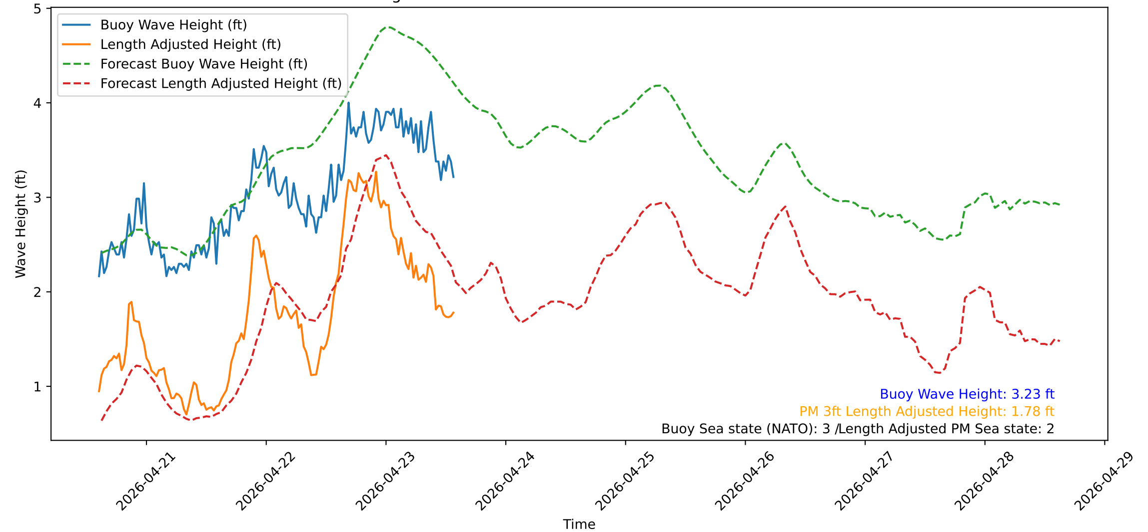
Wave Heights over Time for Green Beach at 2026-04-23 14:31:13
