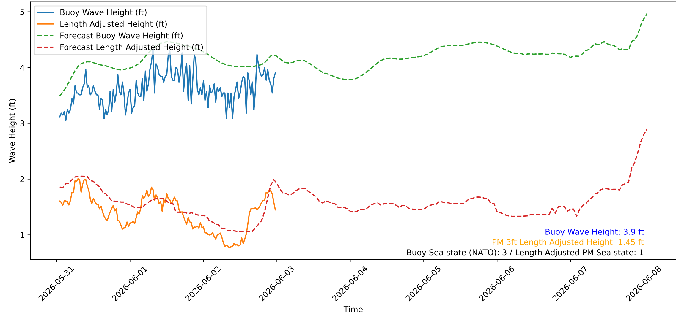
Wave Heights over Time for Green Beach at 2026-06-03 01:01:08
