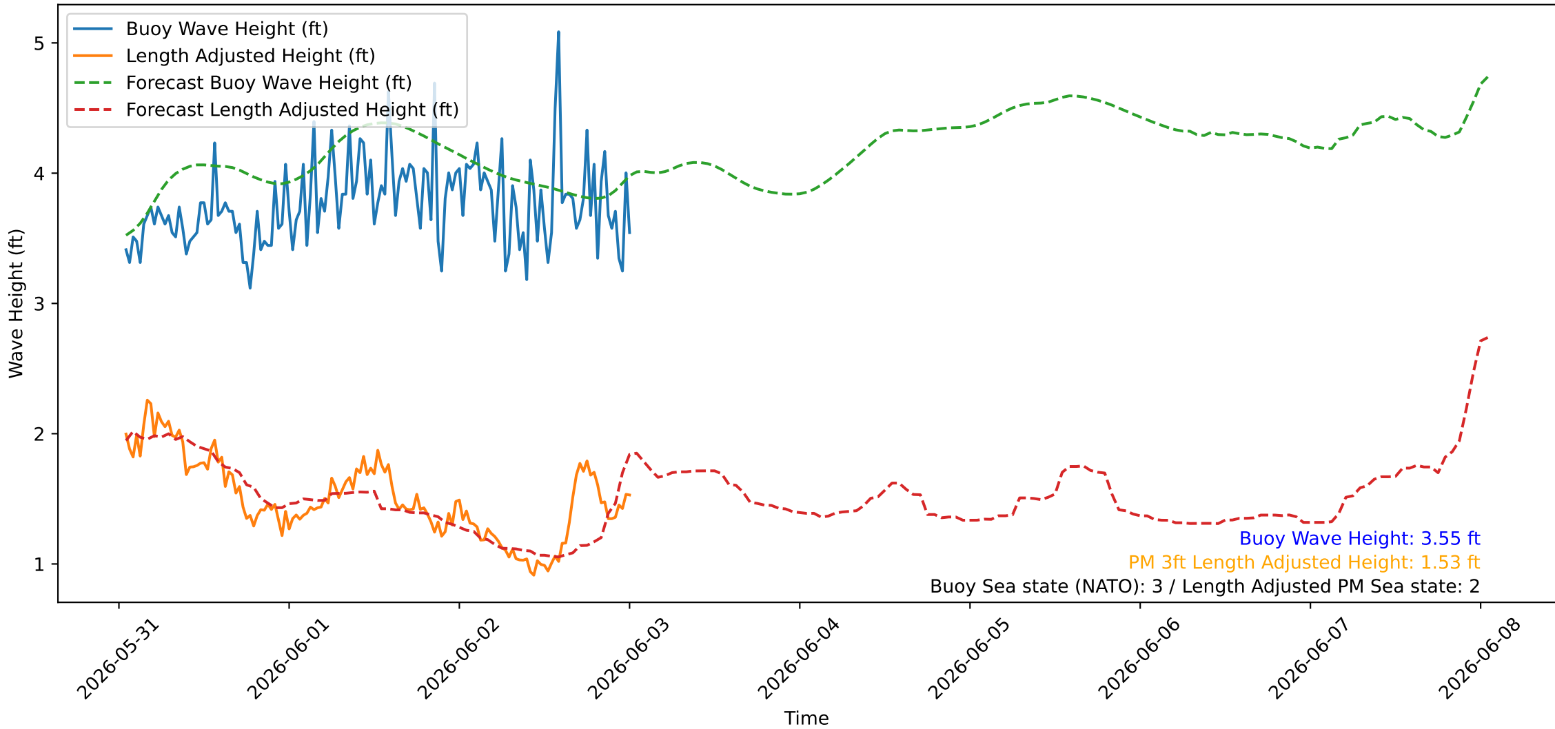
Wave Heights over Time for Oceanside Harbor at 2026-06-03 01:00:26
