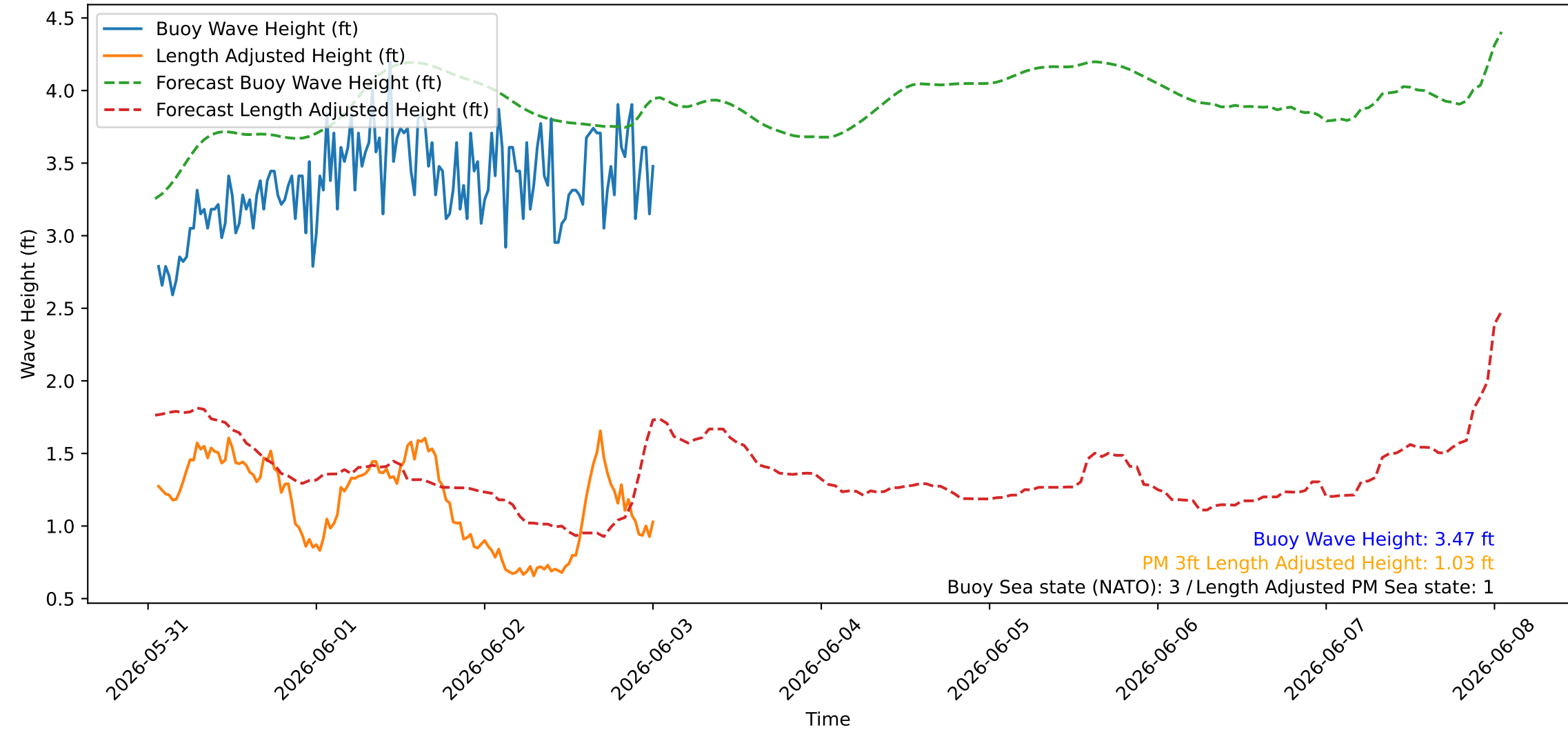
Wave Heights over Time for Red Beach at 2026-06-03 01:00:45
