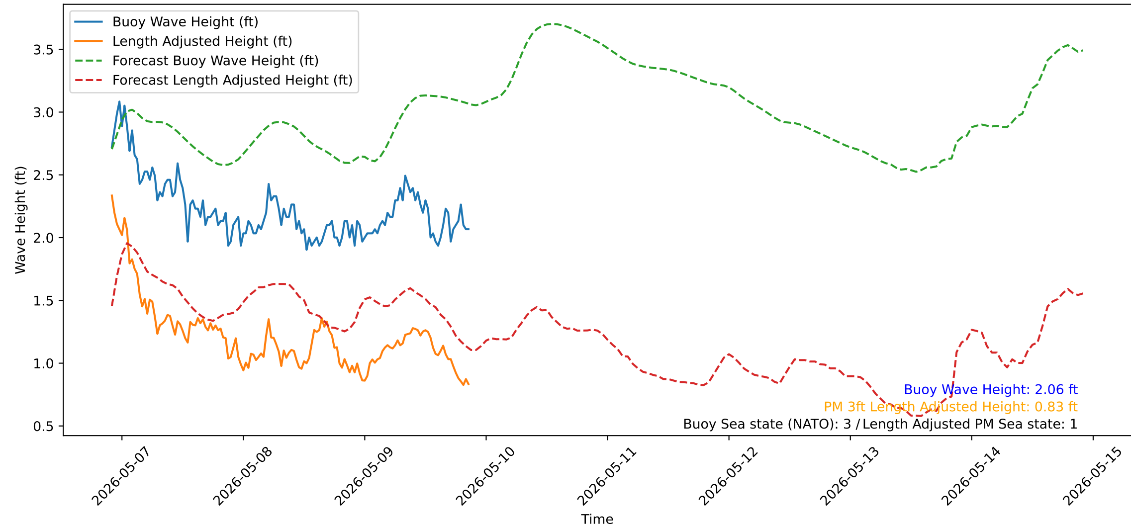
Wave Heights over Time for Red Beach at 2026-05-09 21:30:51
