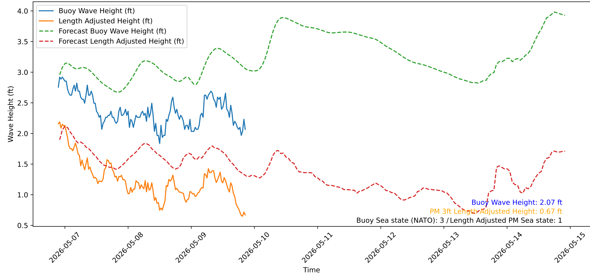
Wave Heights over Time for Green Beach at 2026-05-09 21:31:14
