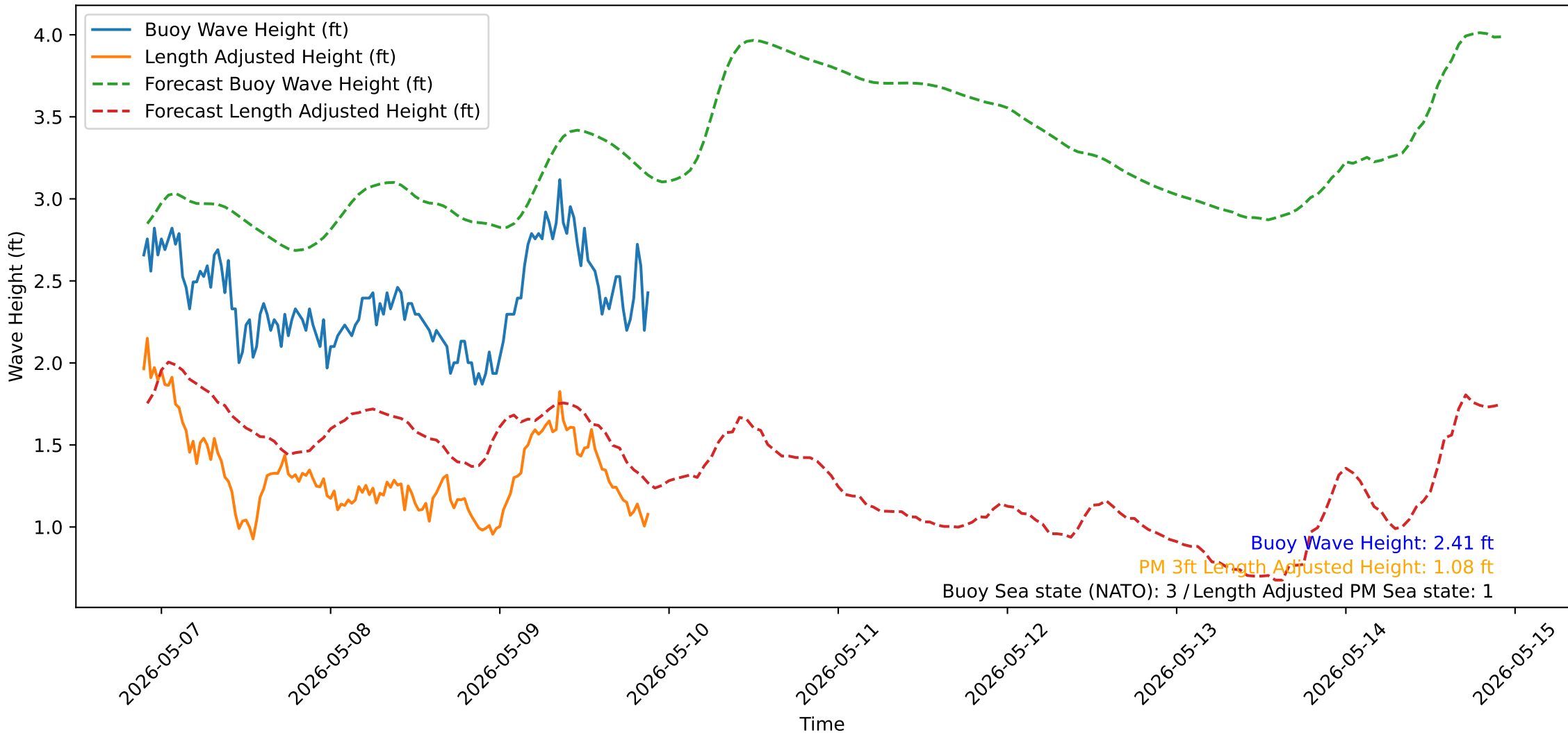
Wave Heights over Time for Oceanside Harbor at 2026-05-09 21:30:31
