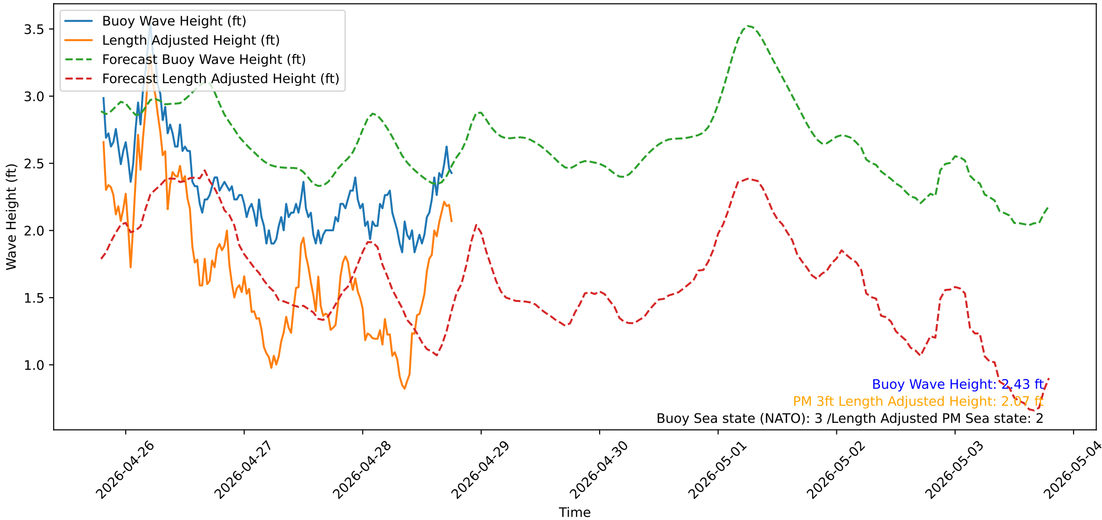
Wave Heights over Time for Red Beach at 2026-04-28 19:10:51
