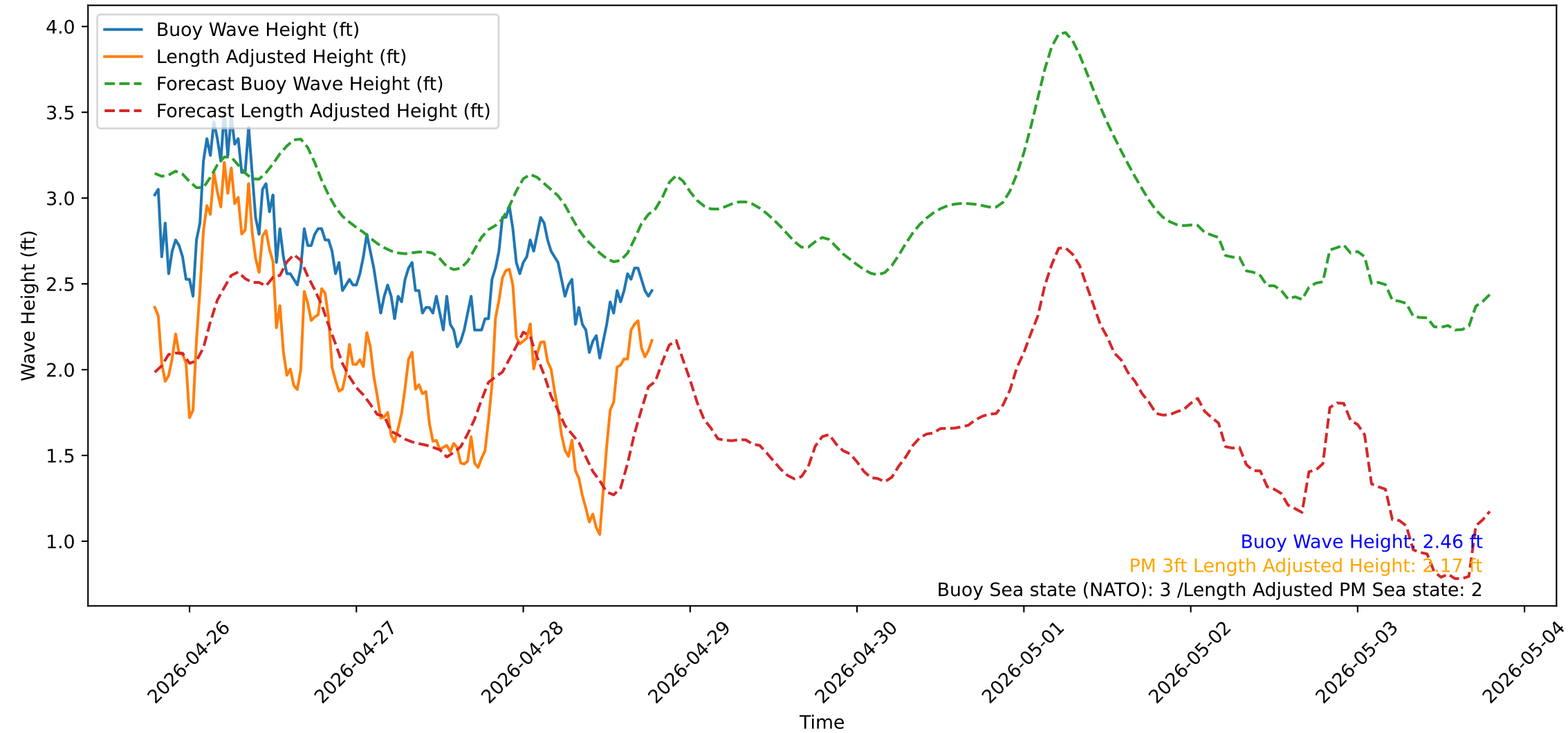
Wave Heights over Time for Green Beach at 2026-04-28 19:11:13
