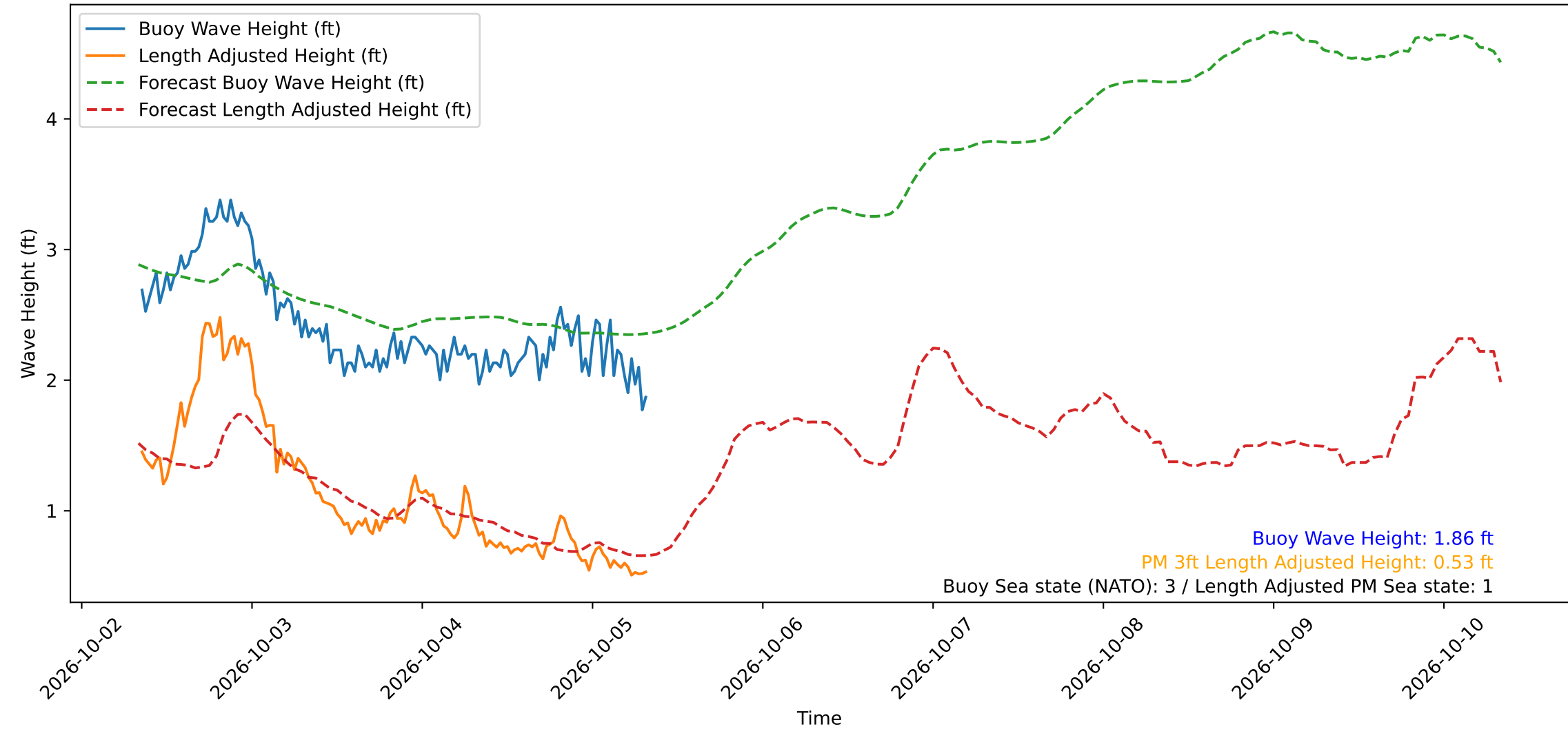
Wave Heights over Time for Green Beach at 2026-10-05 08:21:14
