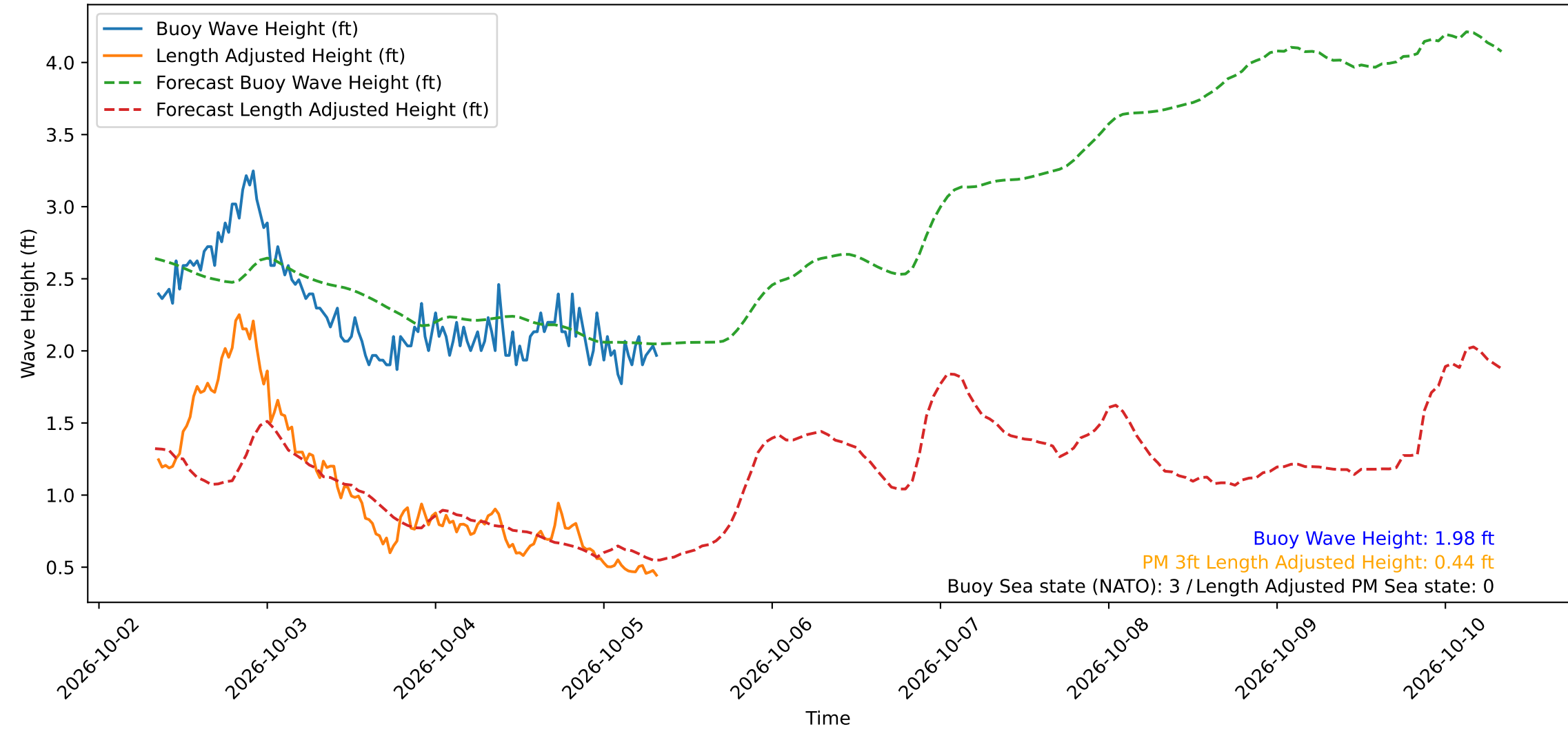
Wave Heights over Time for Red Beach at 2026-10-05 08:20:51
