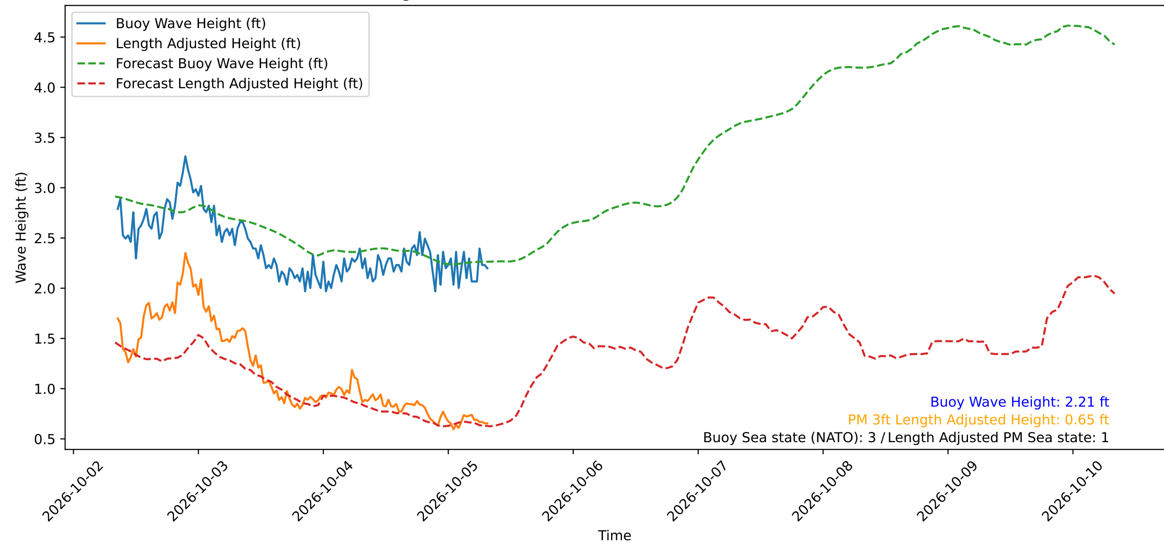
Wave Heights over Time for Oceanside Harbor at 2026-10-05 08:20:30
