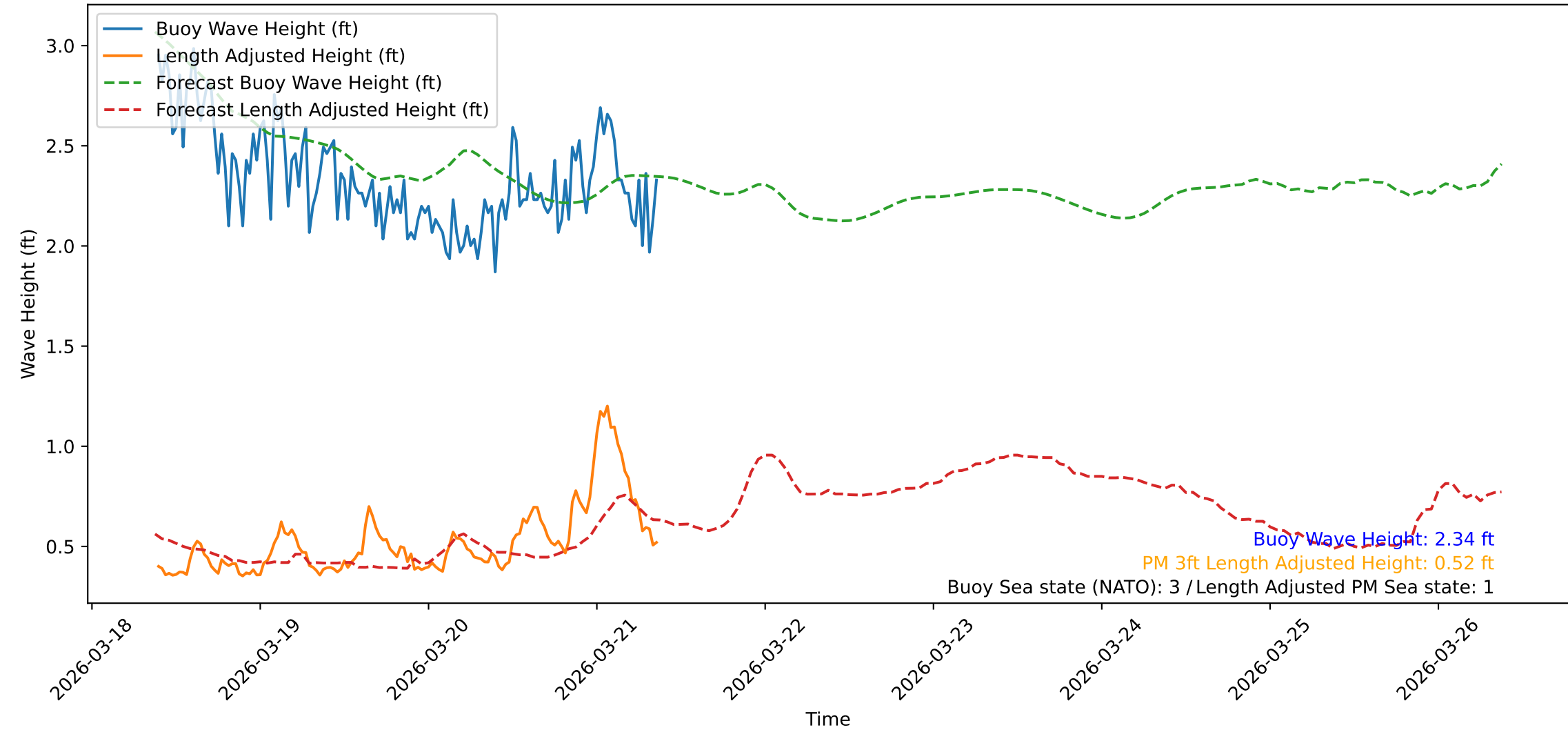
Wave Heights over Time for Red Beach at 2026-03-21 09:20:48
