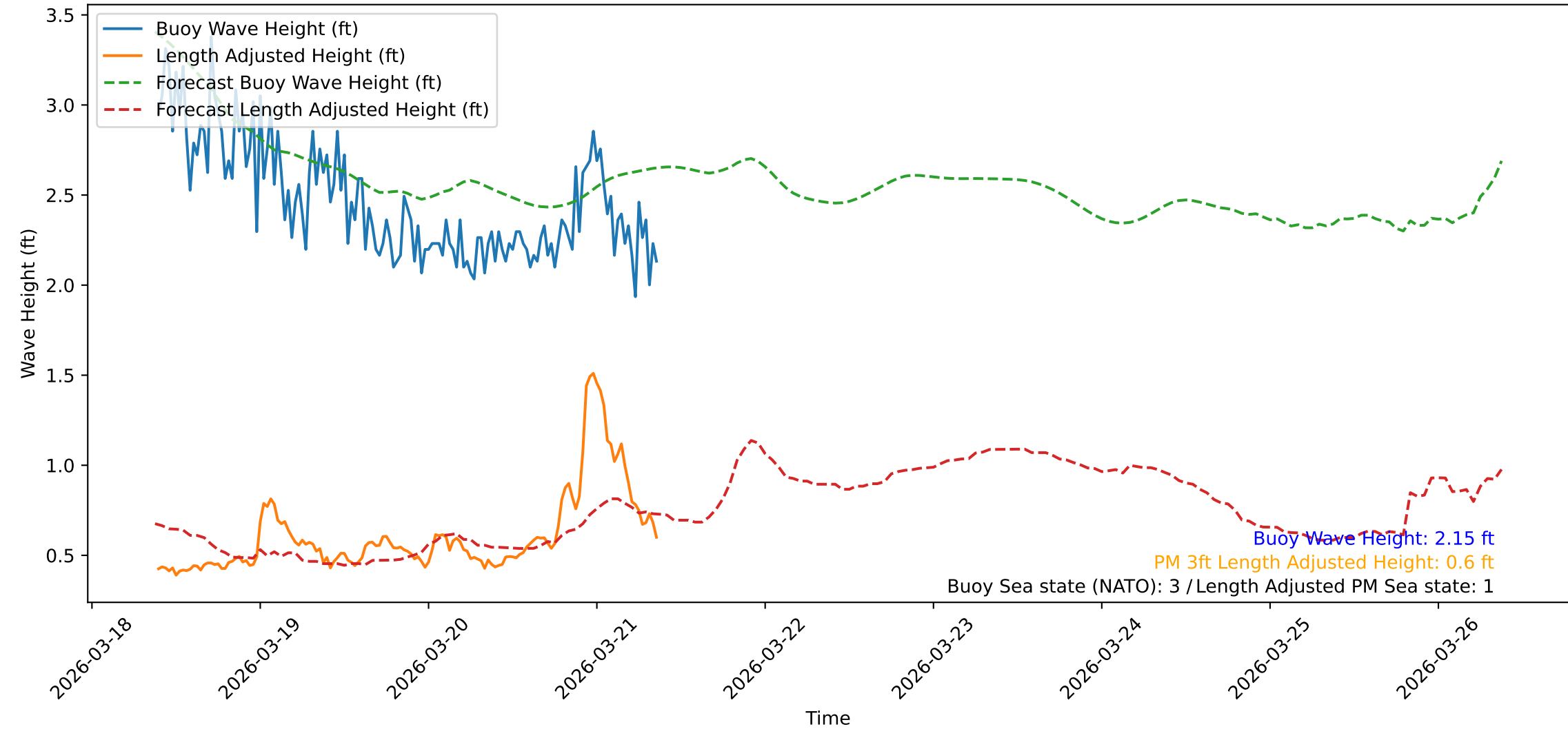
Wave Heights over Time for Green Beach at 2026-03-21 09:21:11
