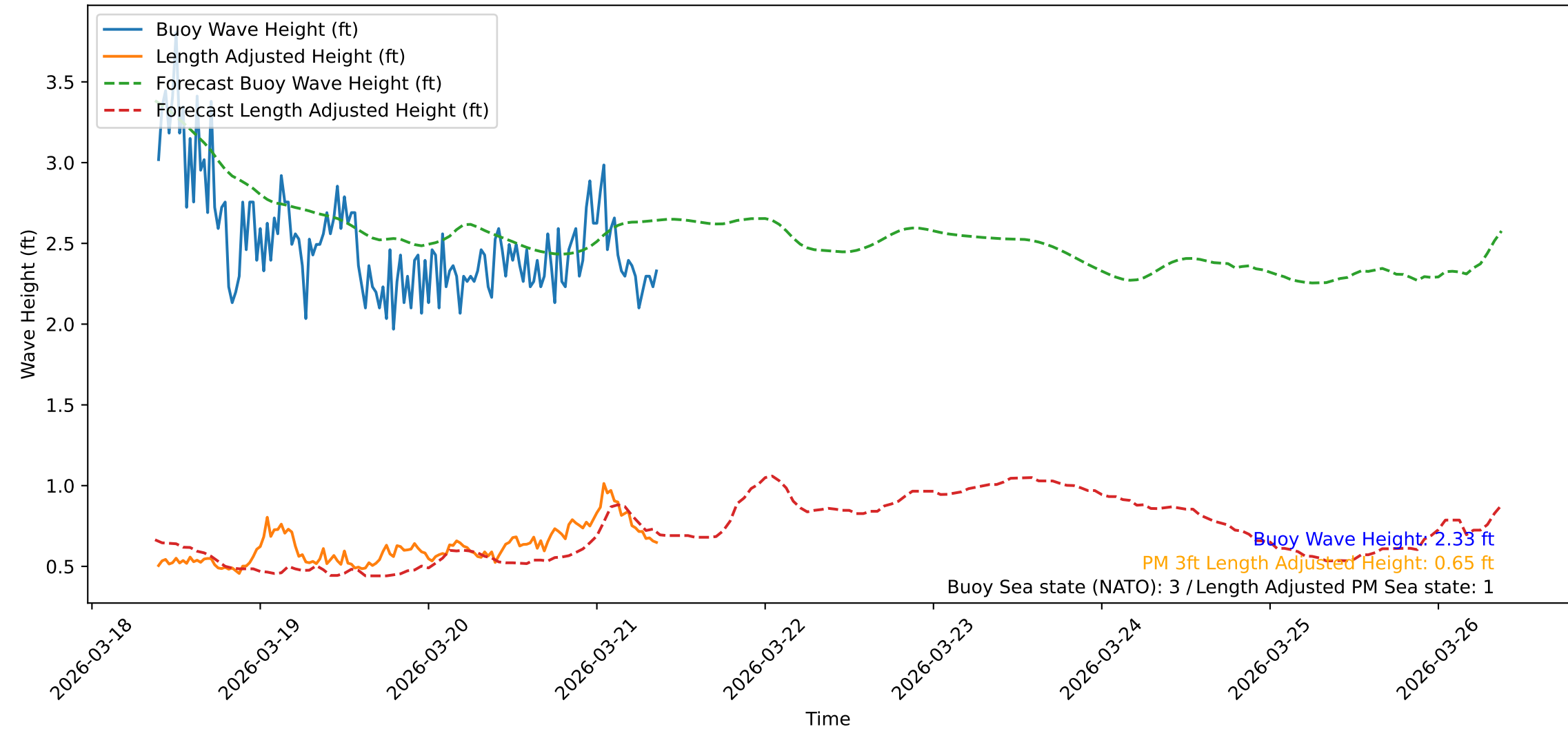
Wave Heights over Time for Oceanside Harbor at 2026-03-21 09:20:32
