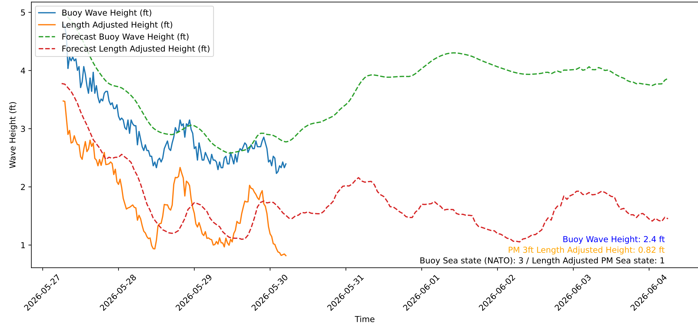
Wave Heights over Time for Red Beach at 2026-05-30 06:00:42
