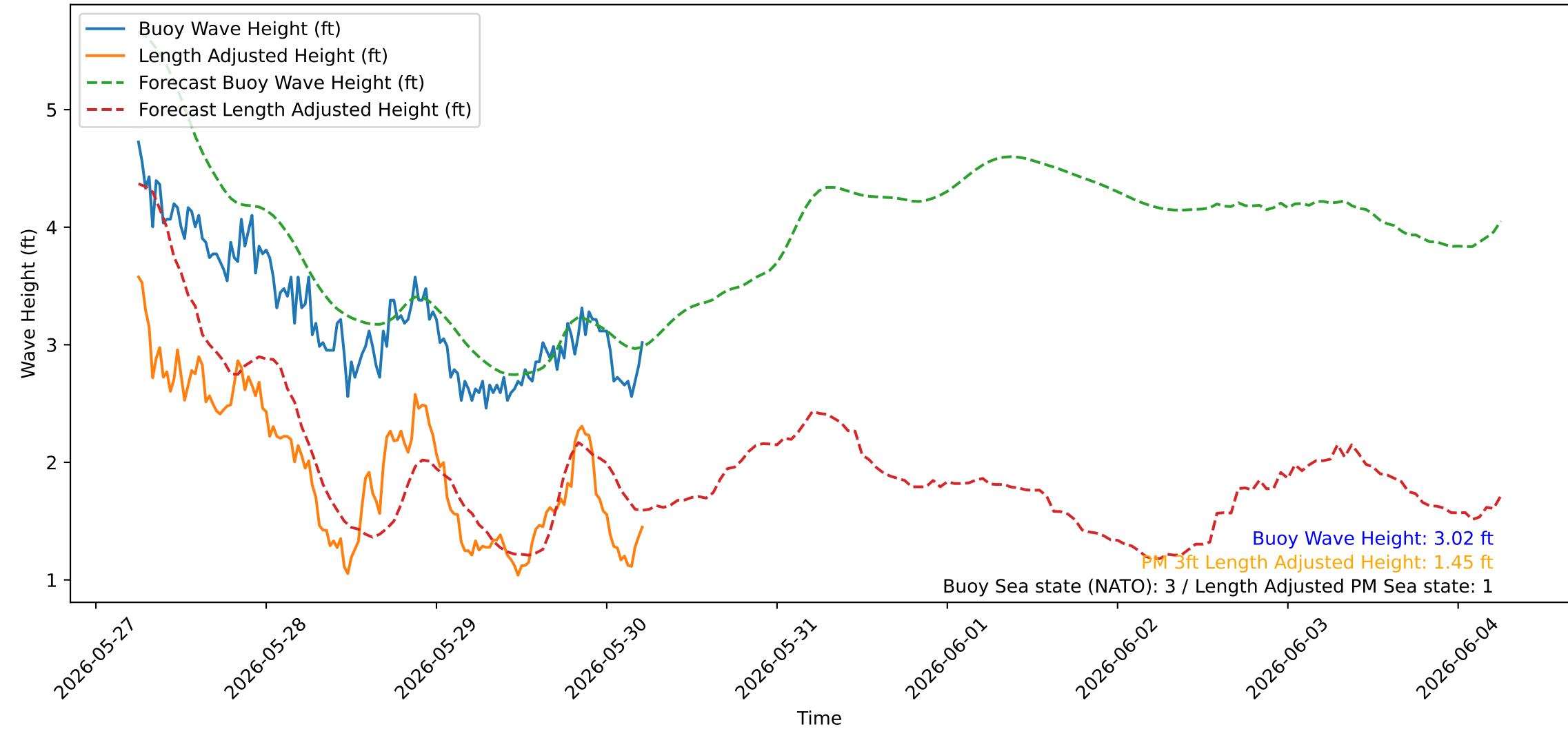
Wave Heights over Time for Green Beach at 2026-05-30 06:01:05
