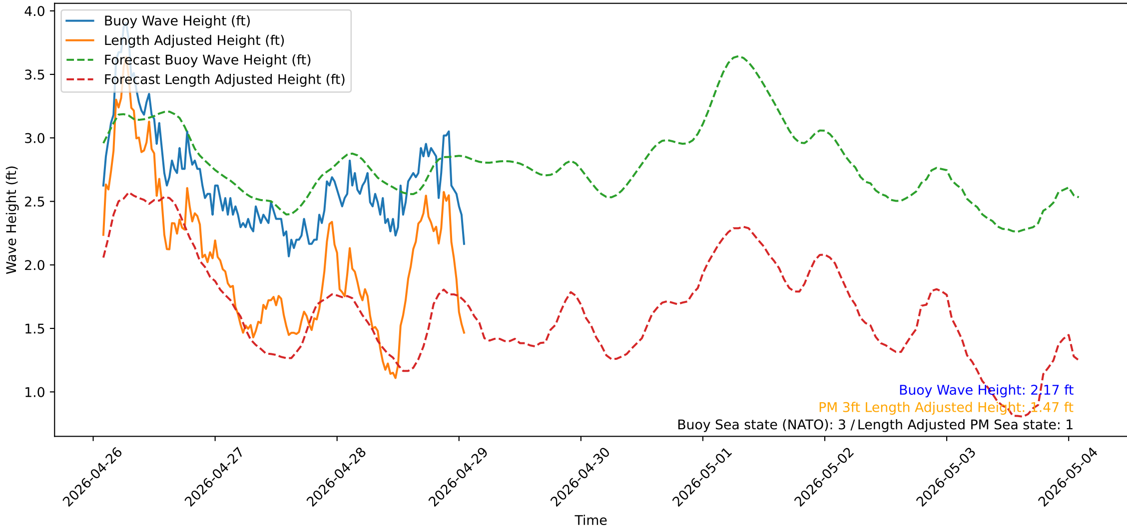
Wave Heights over Time for Oceanside Harbor at 2026-04-29 01:50:31
