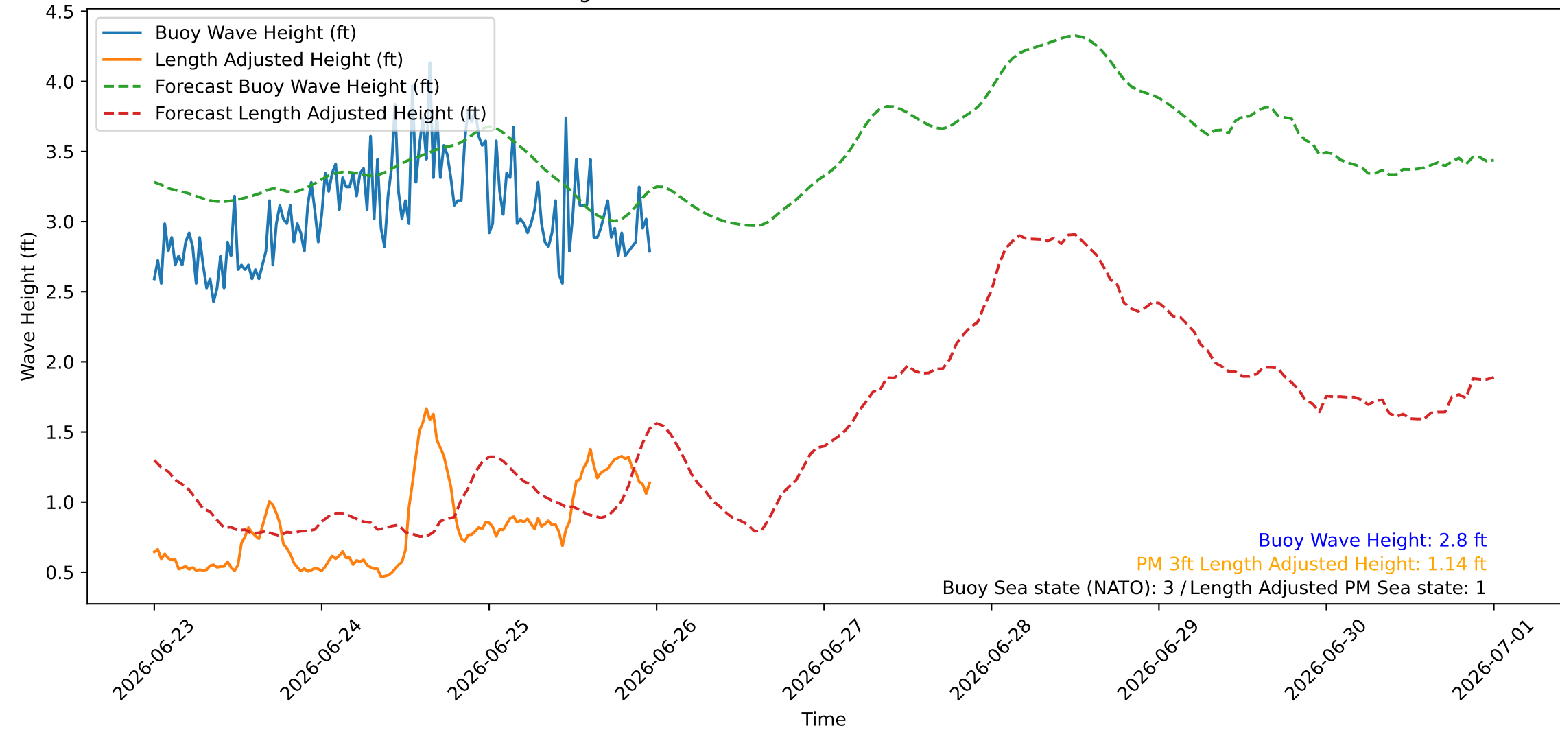
Wave Heights over Time for Red Beach at 2026-06-25 23:50:46
