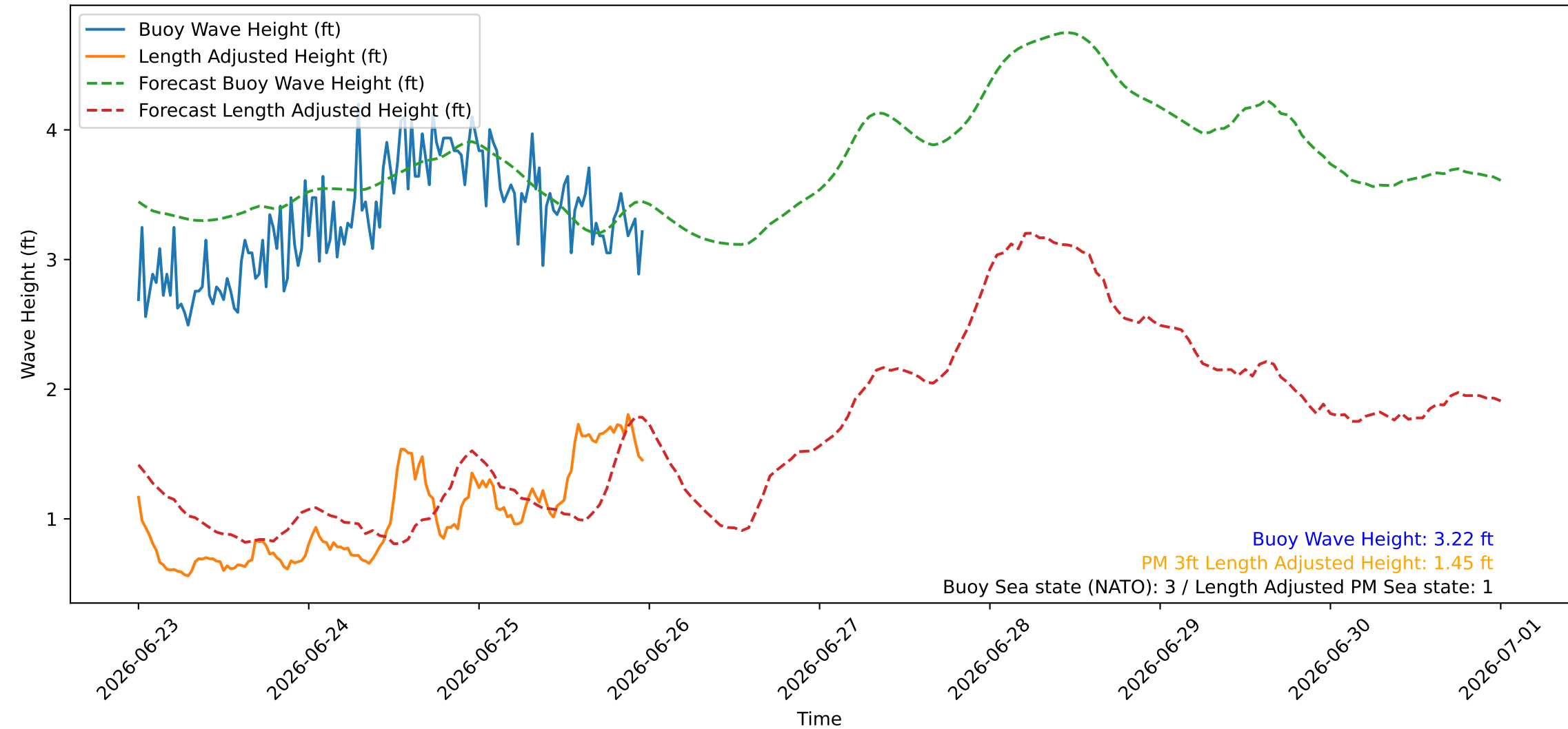
Wave Heights over Time for Green Beach at 2026-06-25 23:51:09
