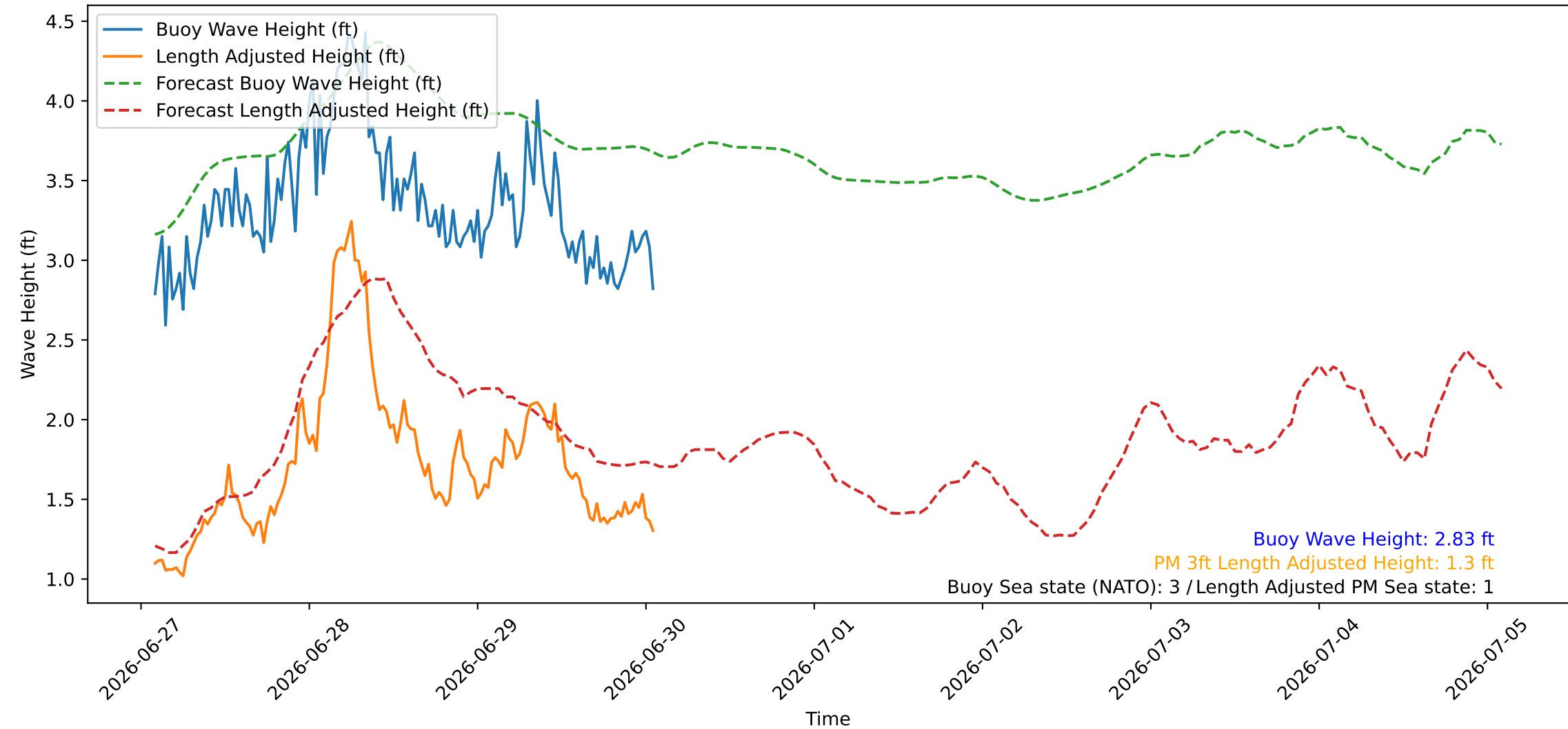
Wave Heights over Time for Oceanside Harbor at 2026-06-30 02:10:26
