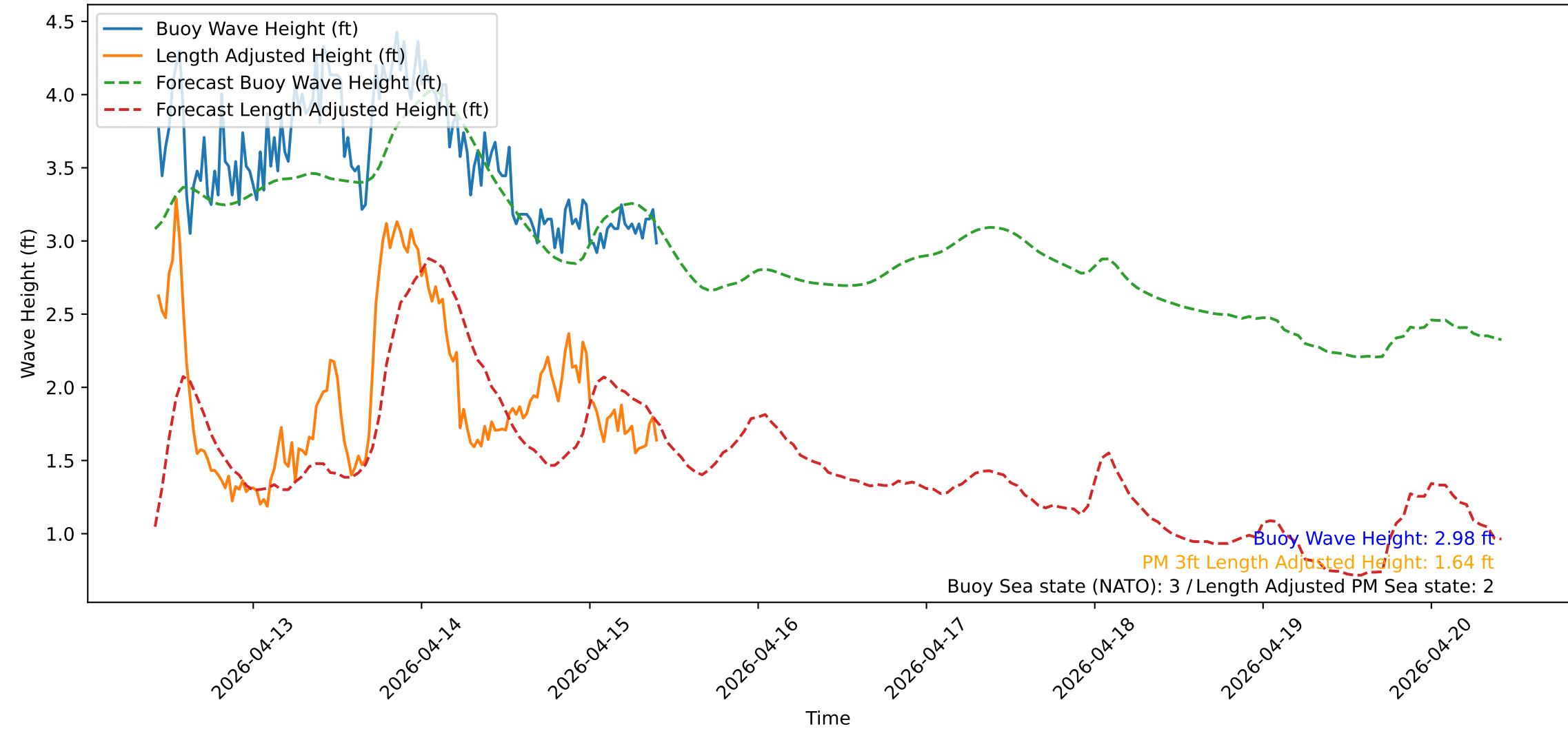
Wave Heights over Time for Red Beach at 2026-04-15 10:10:51
