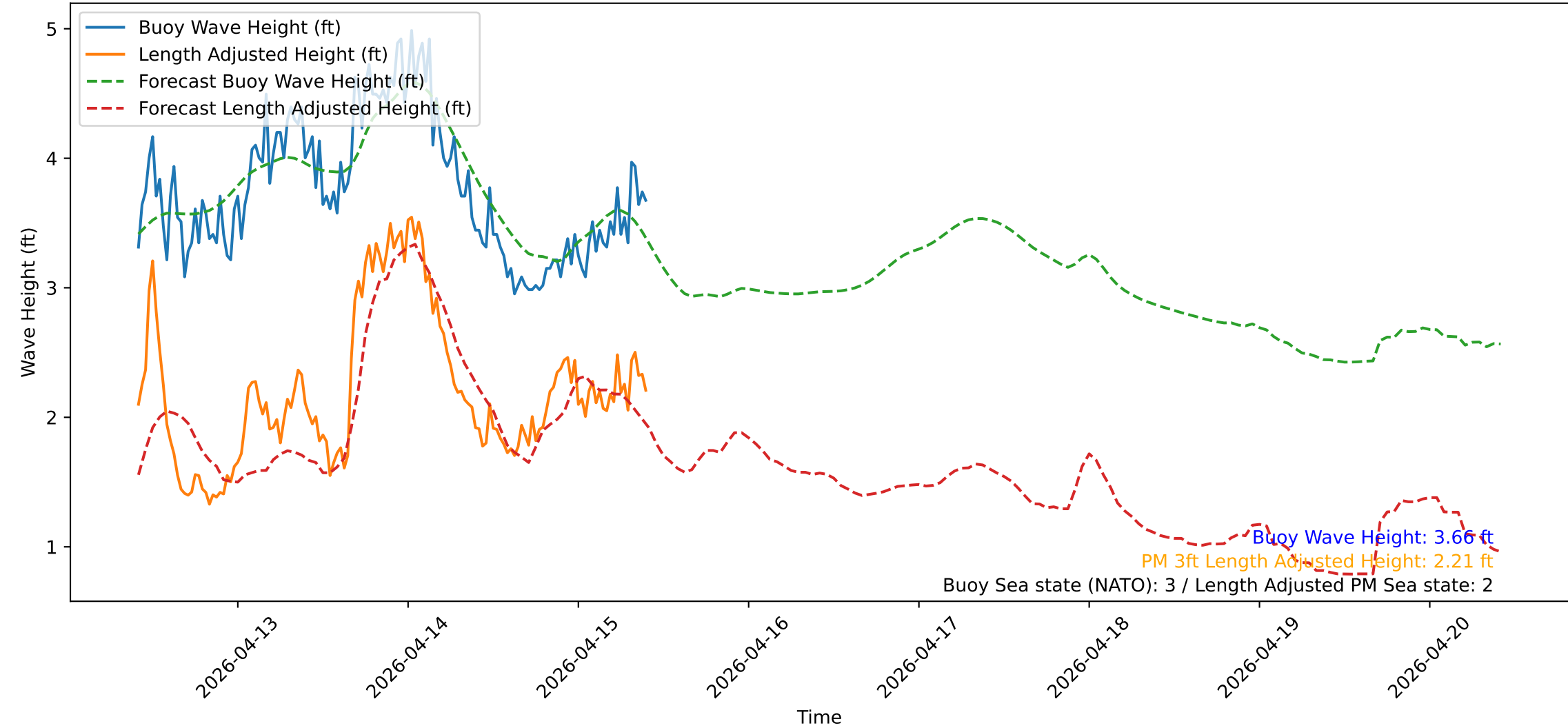
Wave Heights over Time for Green Beach at 2026-04-15 10:11:14
