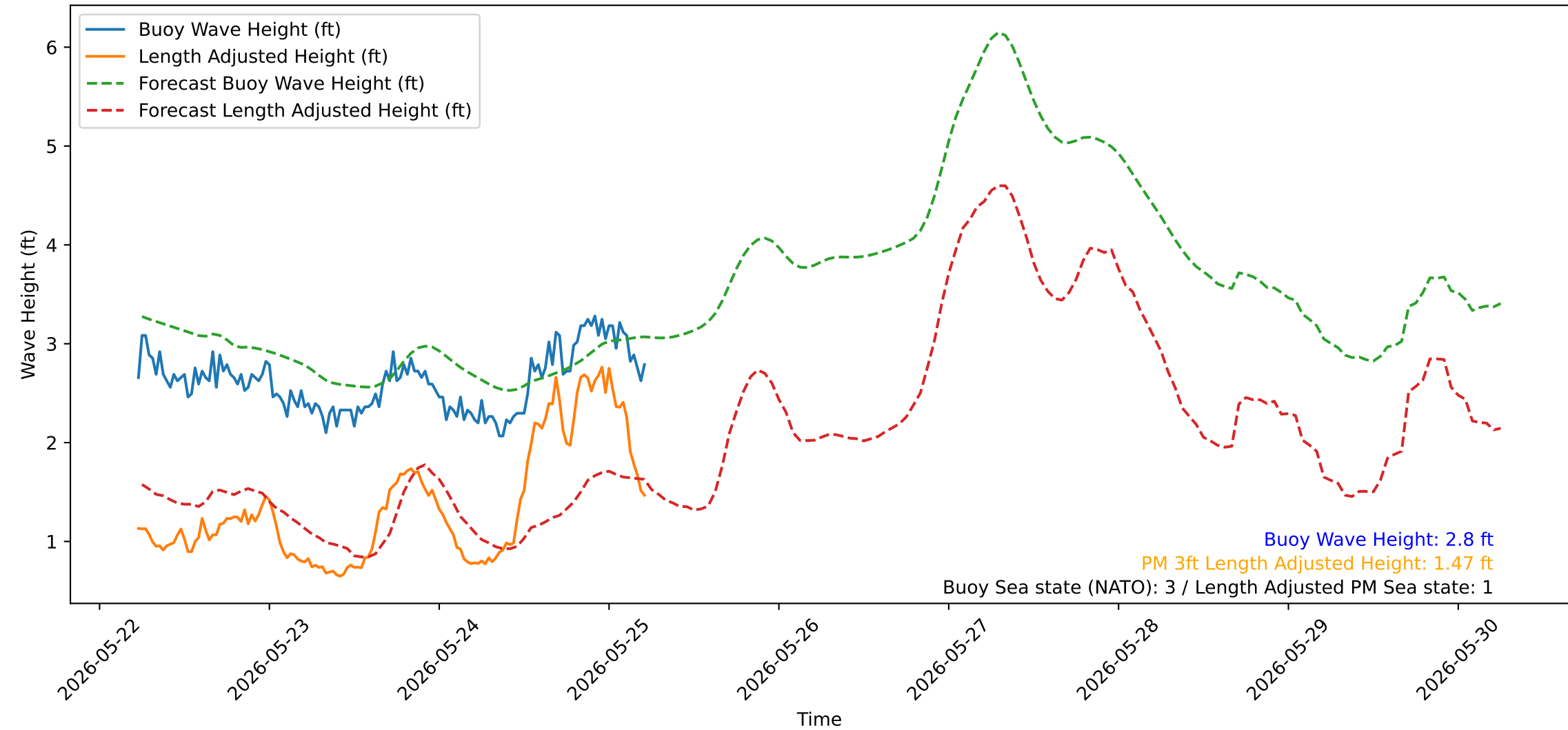
Wave Heights over Time for Green Beach at 2026-05-25 05:41:12
