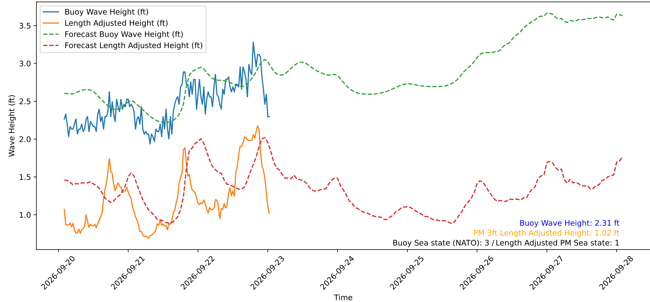
Wave Heights over Time for Red Beach at 2026-09-23 01:30:49
