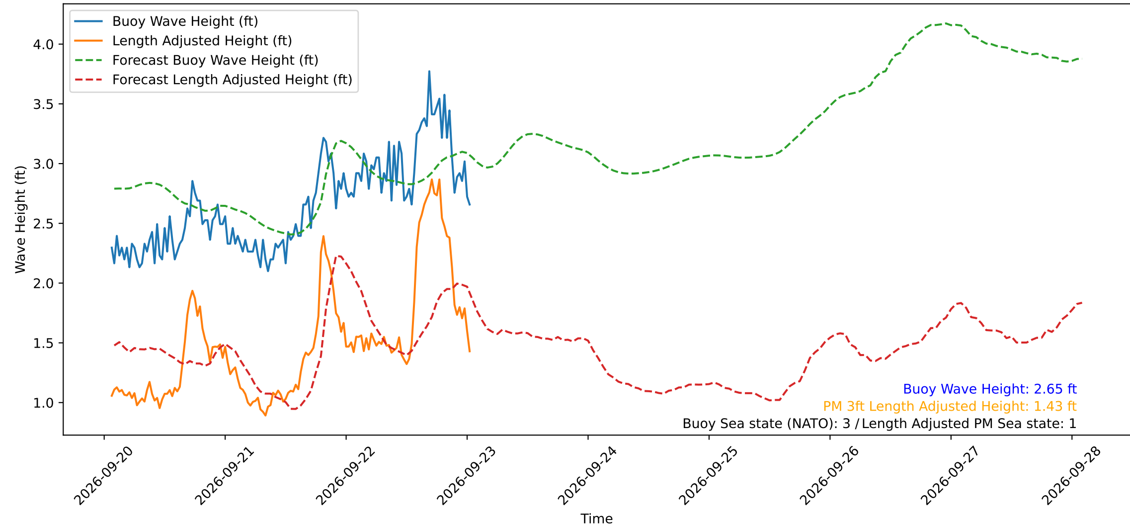
Wave Heights over Time for Oceanside Harbor at 2026-09-23 01:30:30
