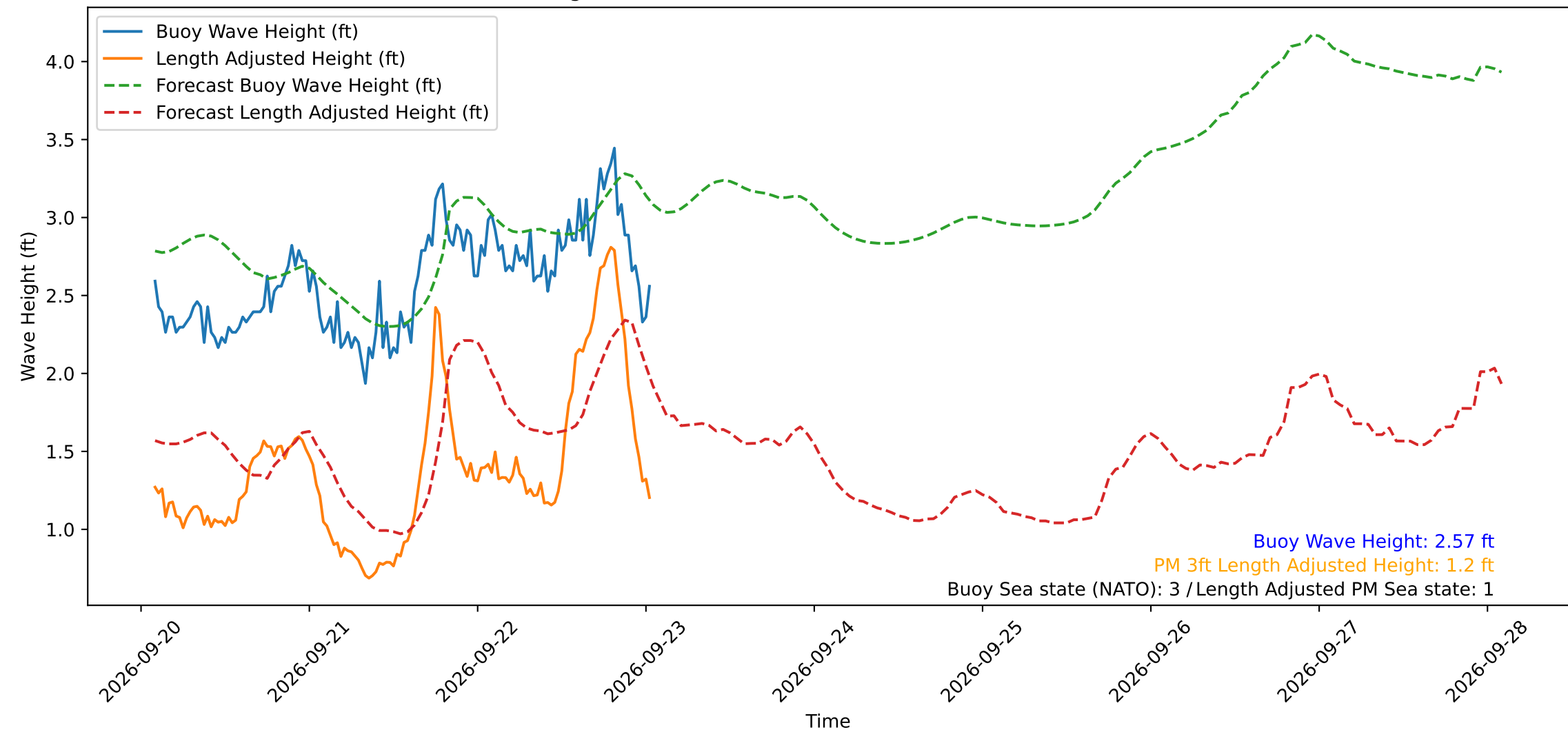
Wave Heights over Time for Green Beach at 2026-09-23 01:31:12
