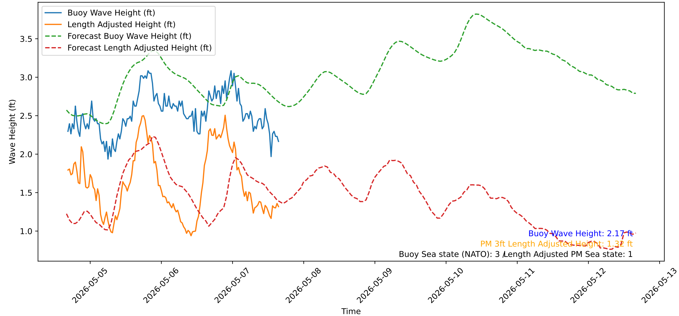
Wave Heights over Time for Red Beach at 2026-05-07 16:20:51
