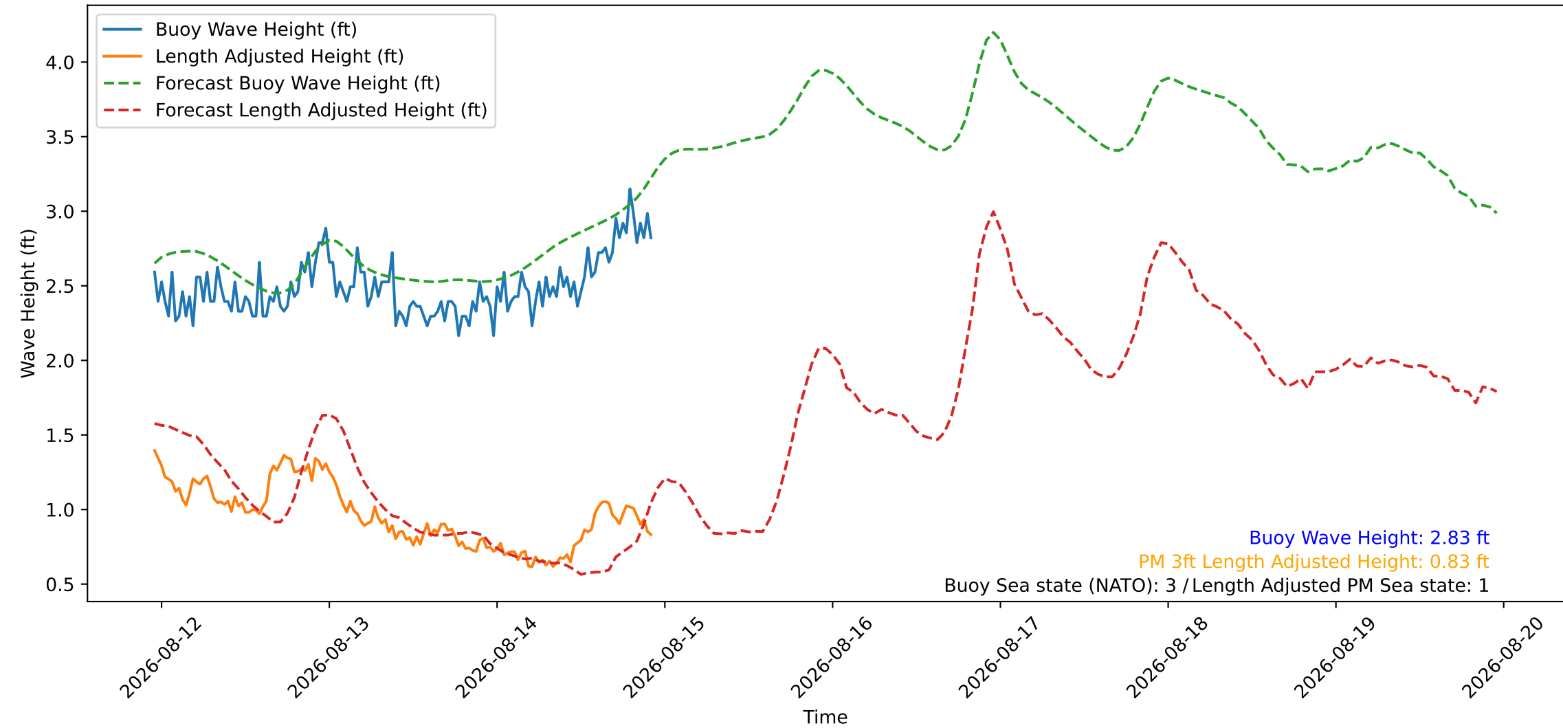
Wave Heights over Time for Red Beach at 2026-08-14 22:50:47
