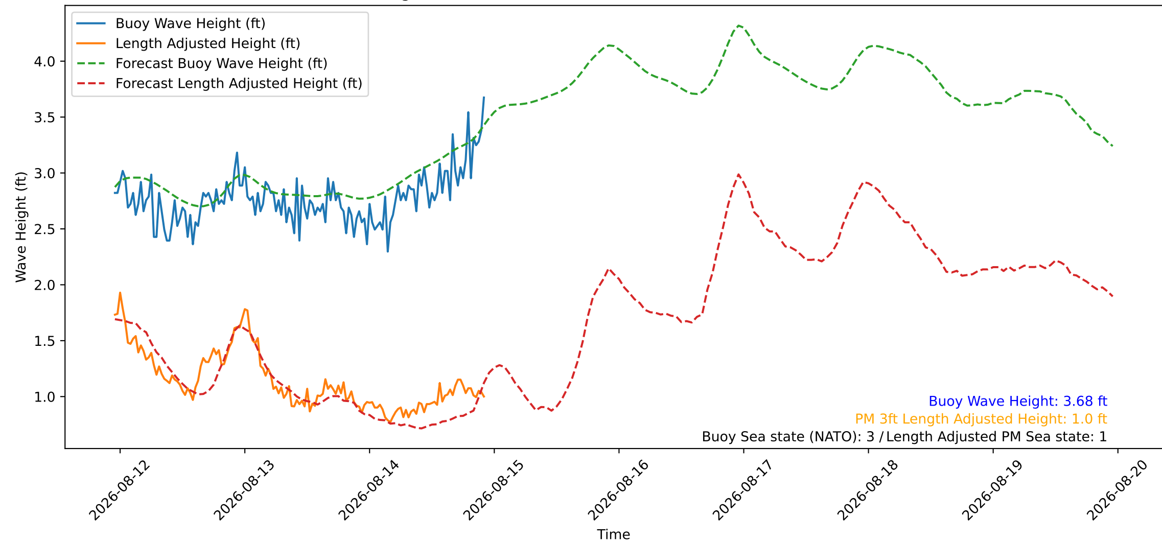
Wave Heights over Time for Oceanside Harbor at 2026-08-14 22:50:26
