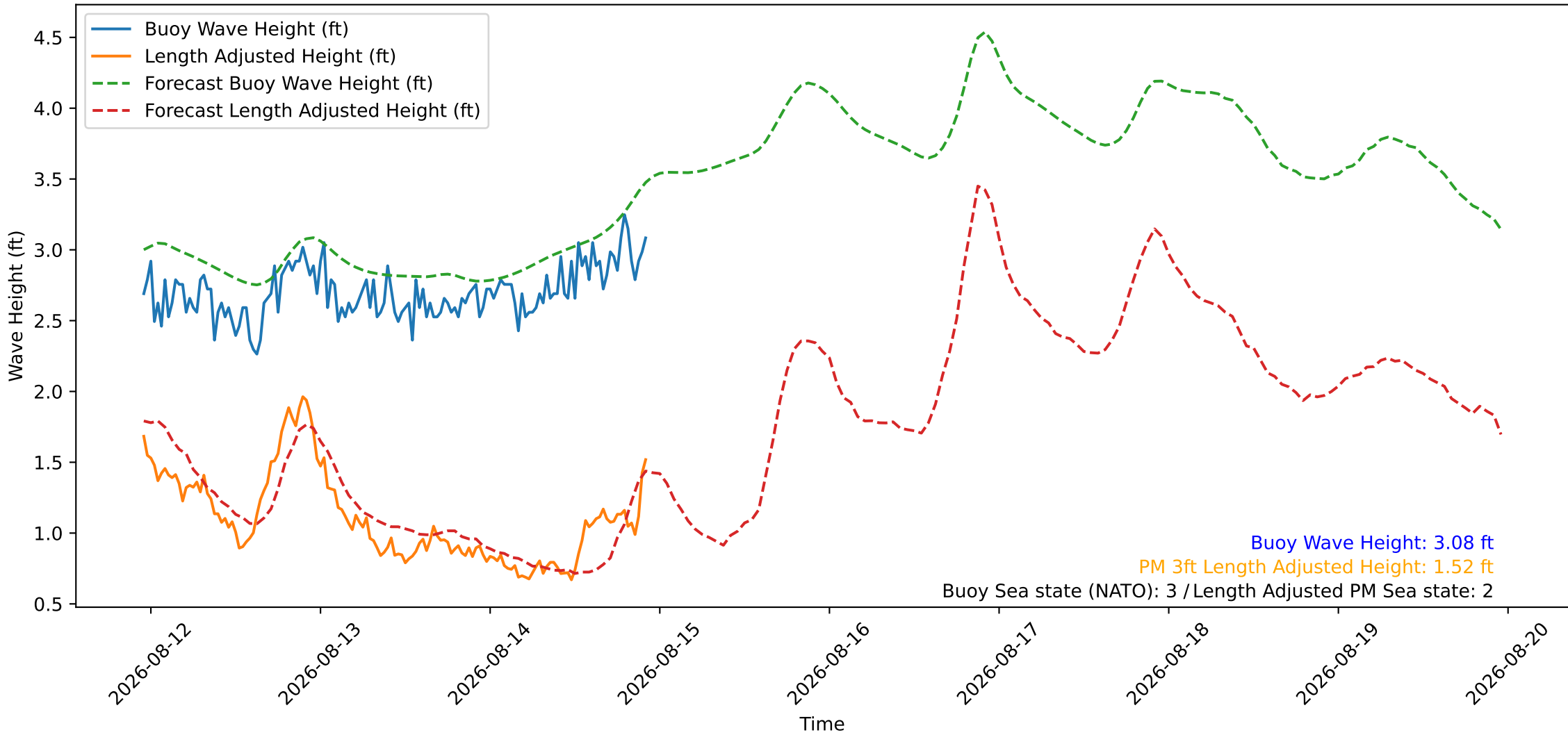
Wave Heights over Time for Green Beach at 2026-08-14 22:51:09
