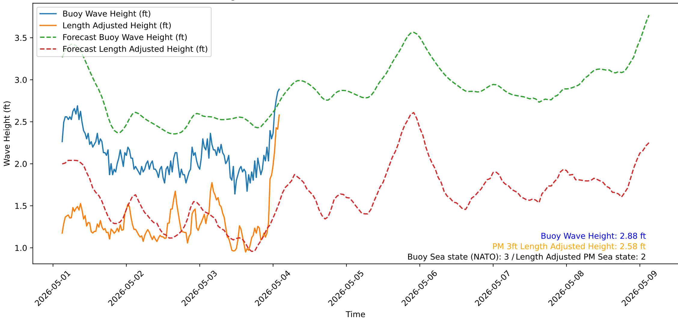
Wave Heights over Time for Oceanside Harbor at 2026-05-04 02:50:31
