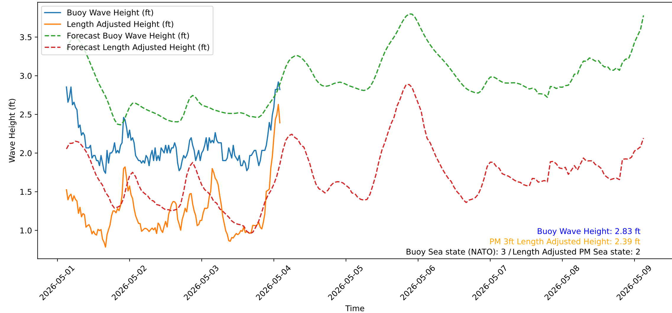
Wave Heights over Time for Green Beach at 2026-05-04 02:51:13
