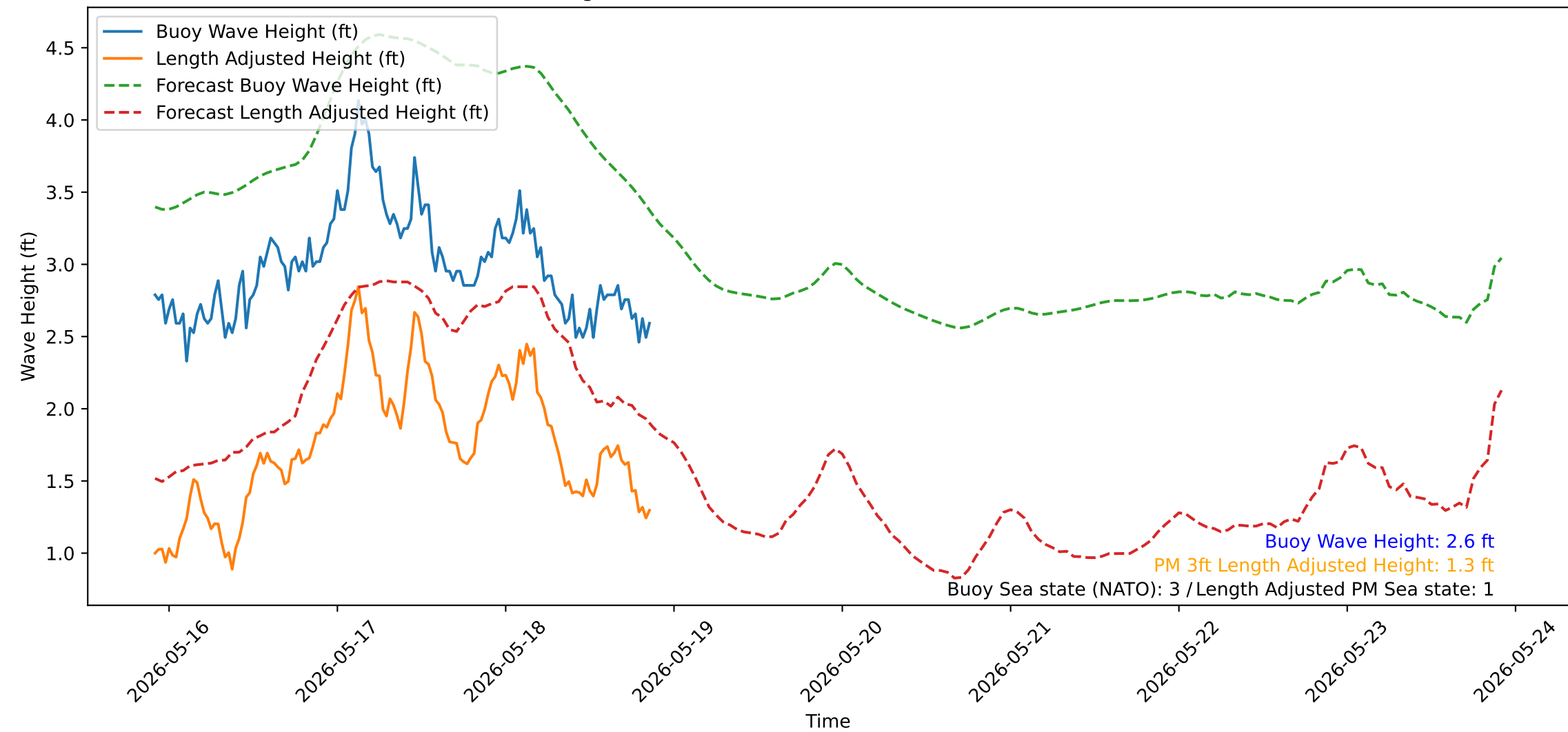
Wave Heights over Time for Red Beach at 2026-05-18 21:30:52
