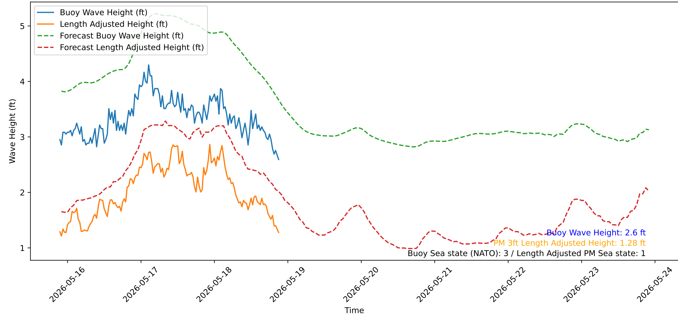
Wave Heights over Time for Oceanside Harbor at 2026-05-18 21:30:32
