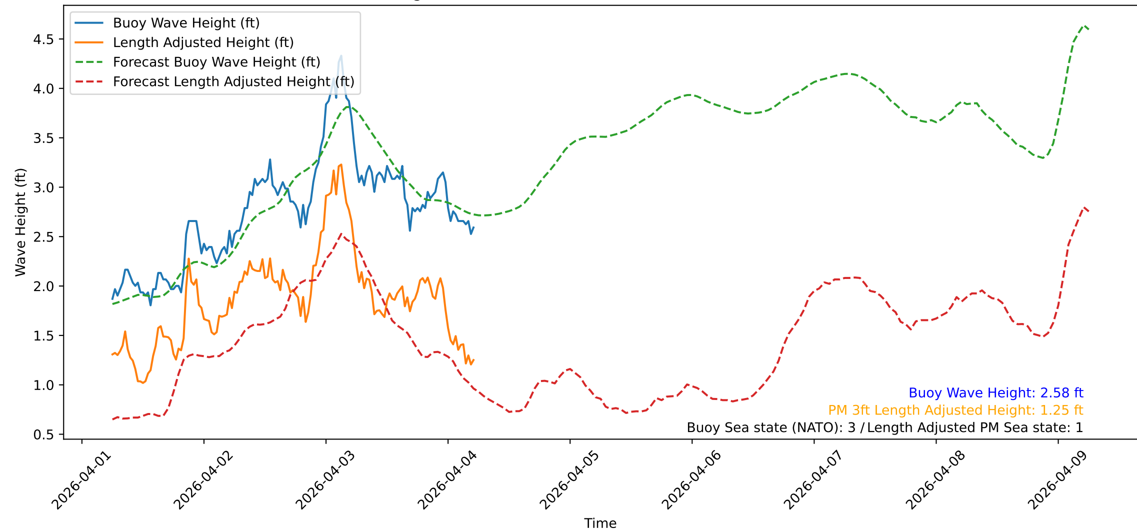
Wave Heights over Time for Green Beach at 2026-04-04 05:51:10
