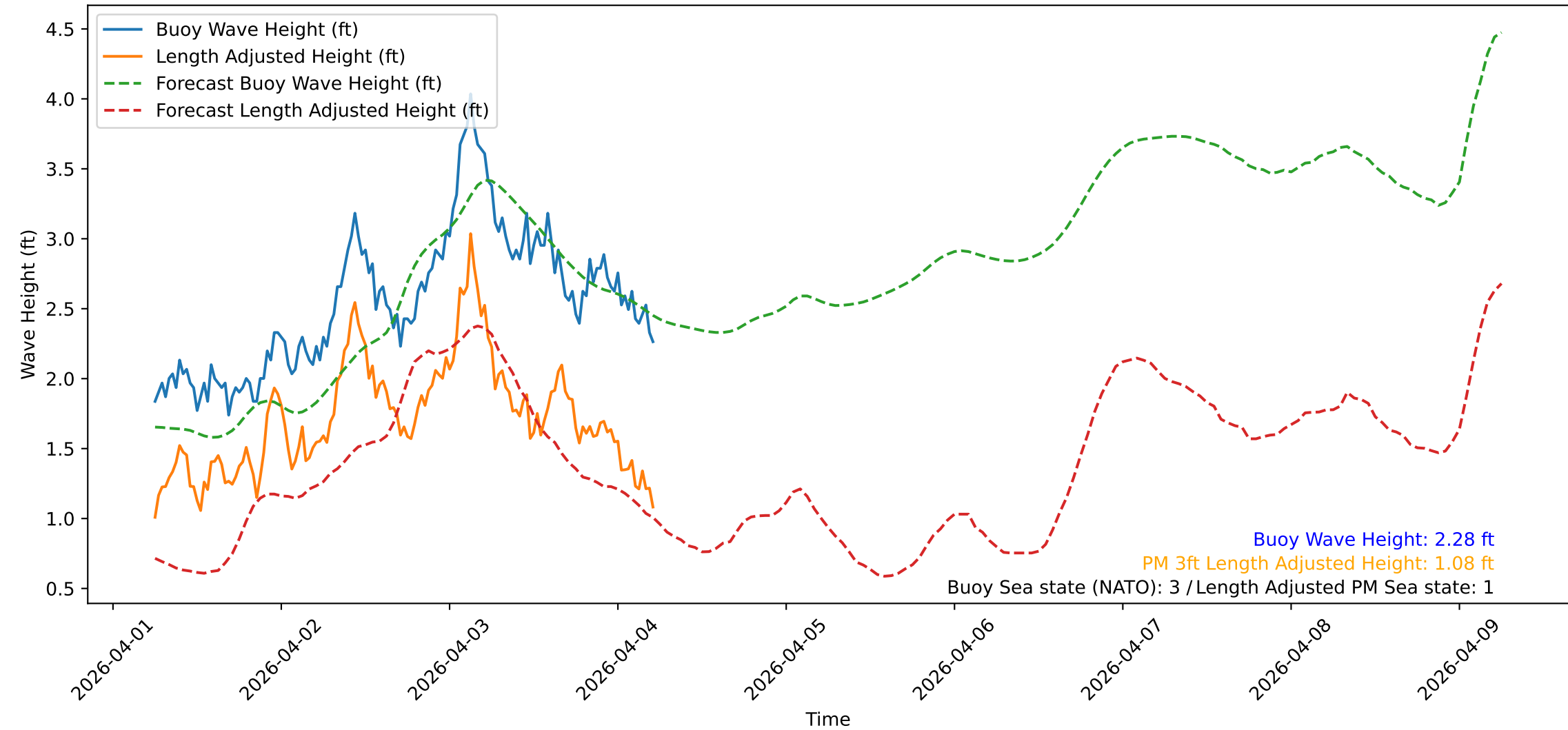
Wave Heights over Time for Oceanside Harbor at 2026-04-04 05:50:31
