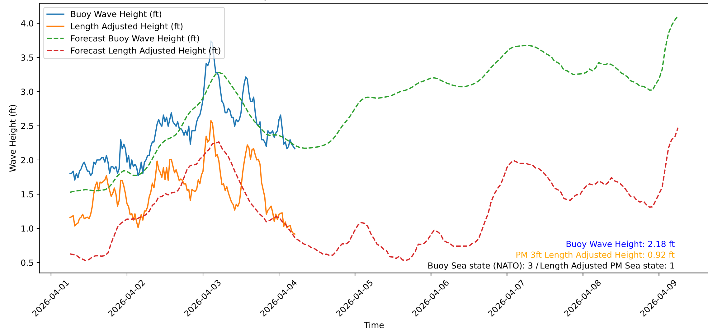
Wave Heights over Time for Red Beach at 2026-04-04 05:50:48
