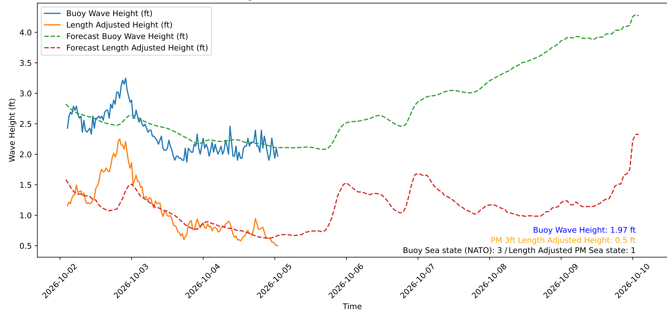
Wave Heights over Time for Red Beach at 2026-10-05 02:00:49
