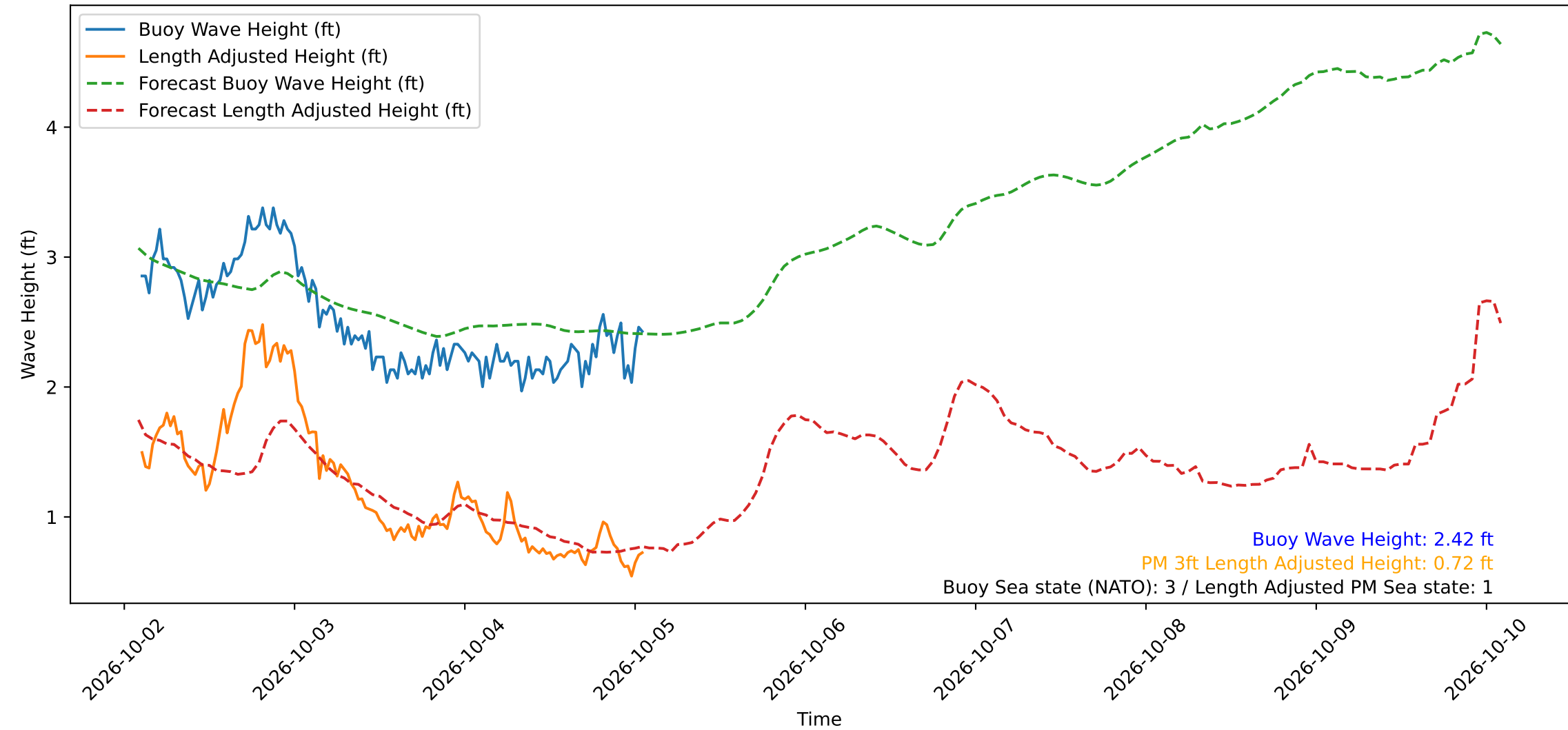
Wave Heights over Time for Green Beach at 2026-10-05 02:01:11
