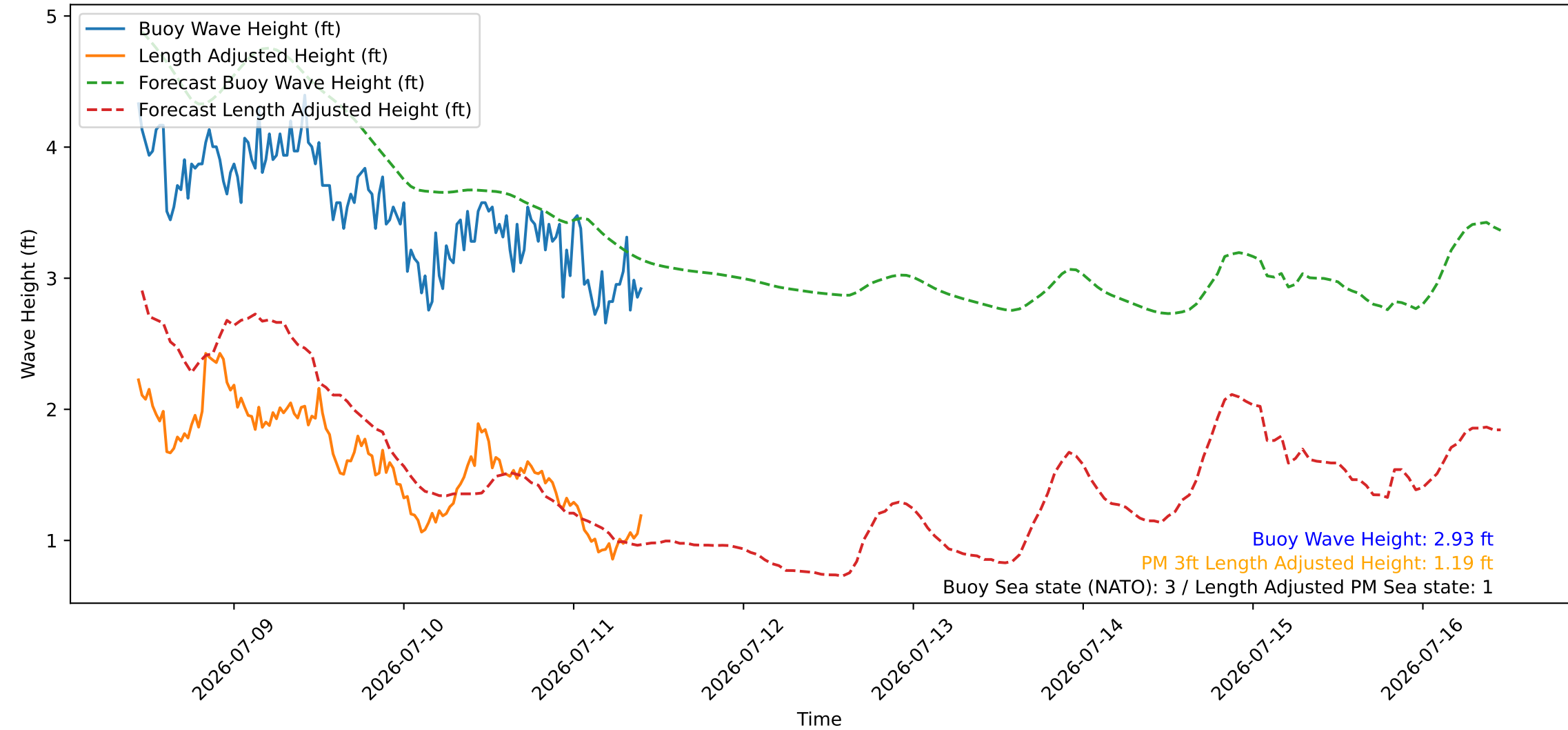
Wave Heights over Time for Green Beach at 2026-07-11 10:31:09
