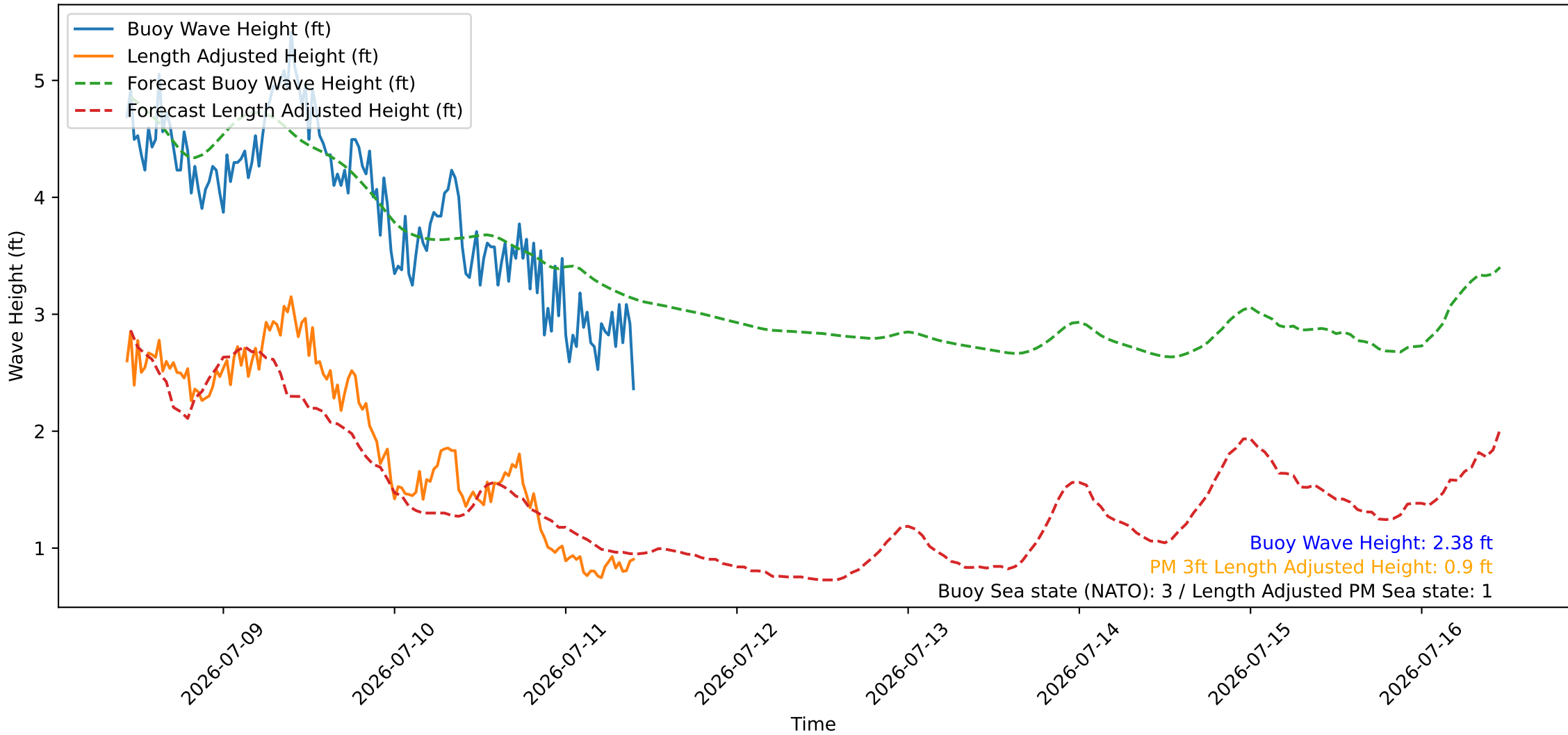
Wave Heights over Time for Oceanside Harbor at 2026-07-11 10:30:27
