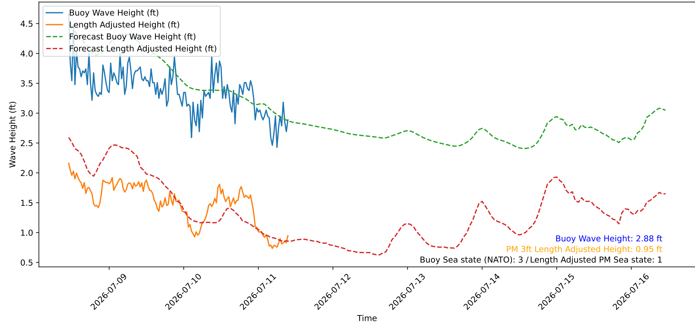
Wave Heights over Time for Red Beach at 2026-07-11 10:30:47
