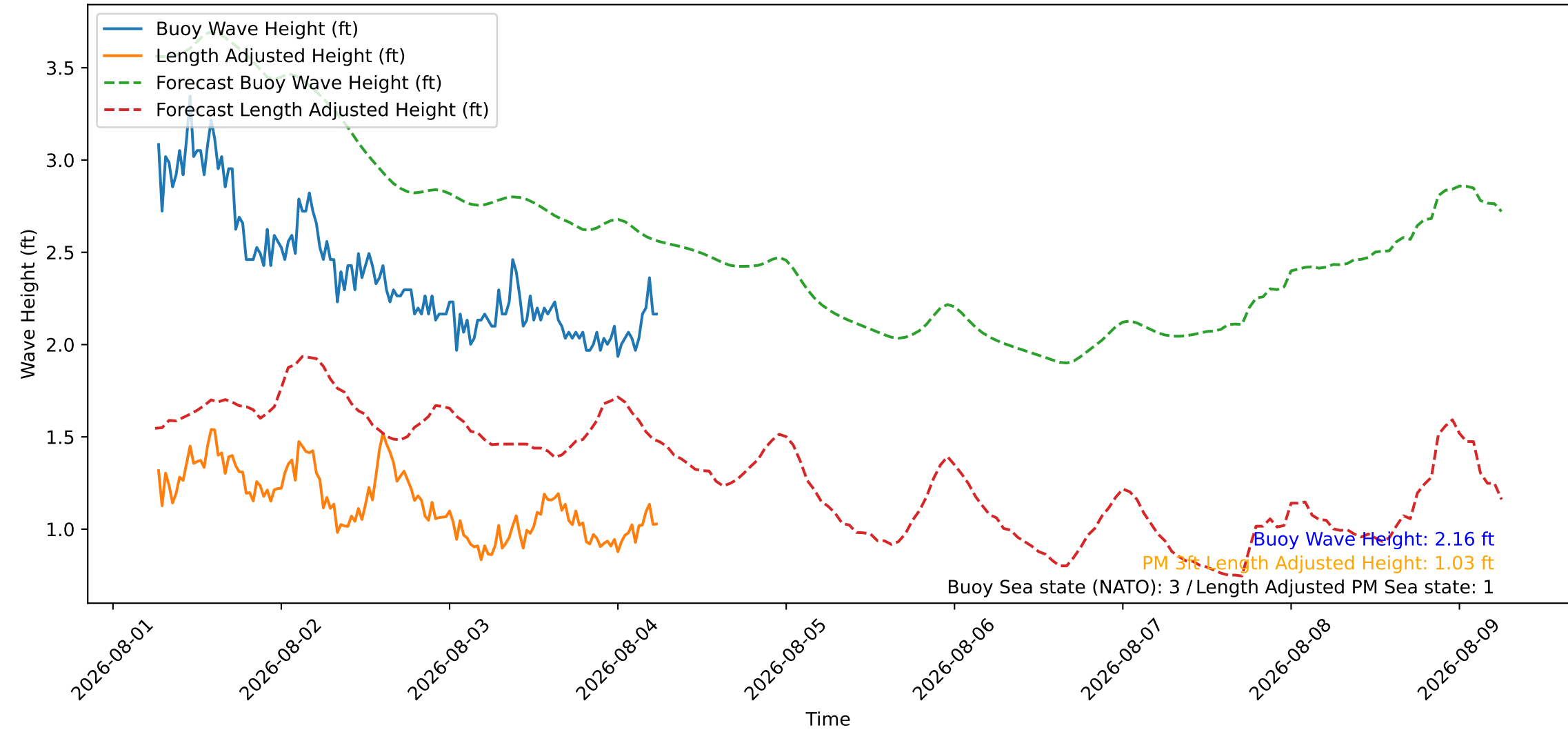
Wave Heights over Time for Red Beach at 2026-08-04 06:20:47
