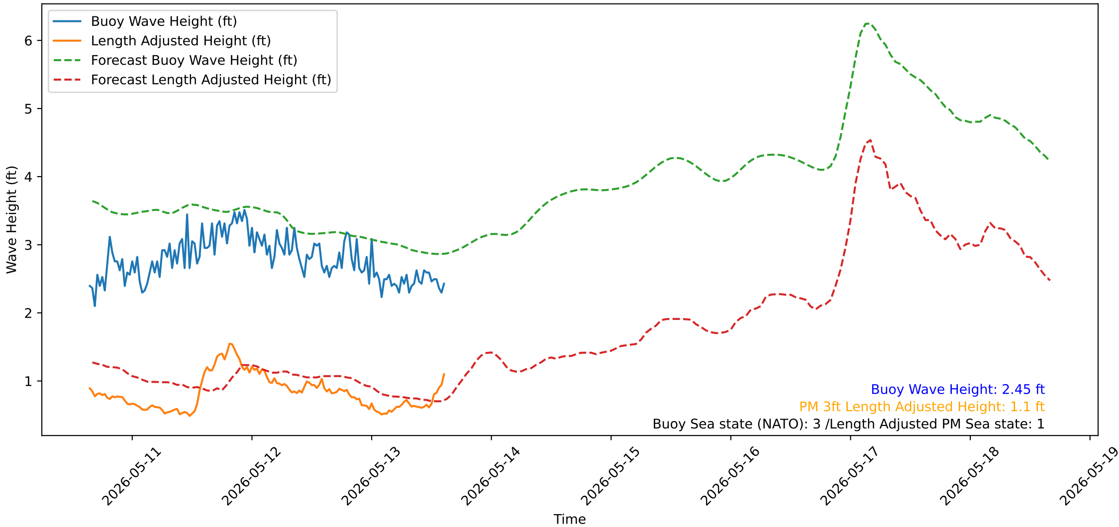
Wave Heights over Time for Green Beach at 2026-05-13 15:31:14
