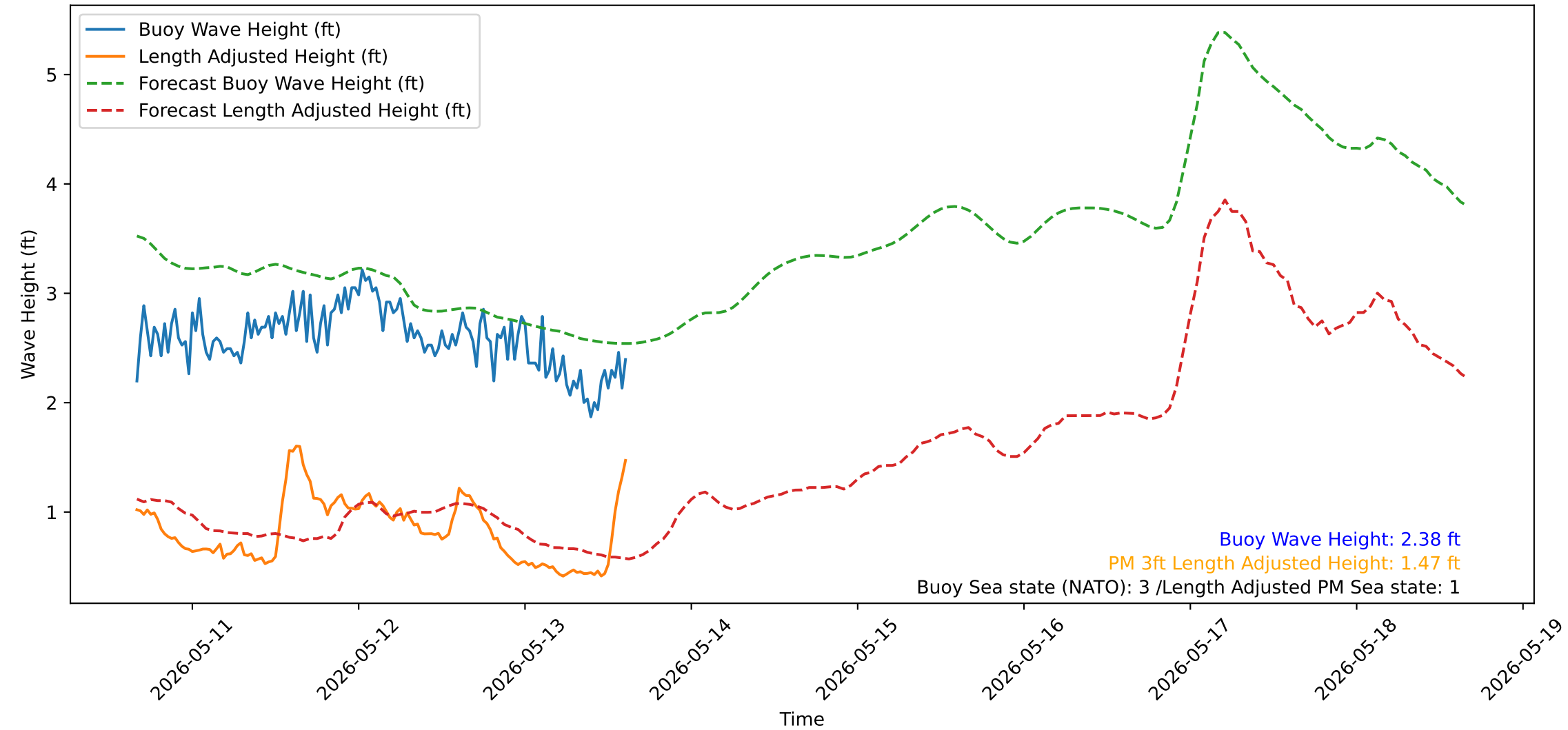
Wave Heights over Time for Red Beach at 2026-05-13 15:30:51
