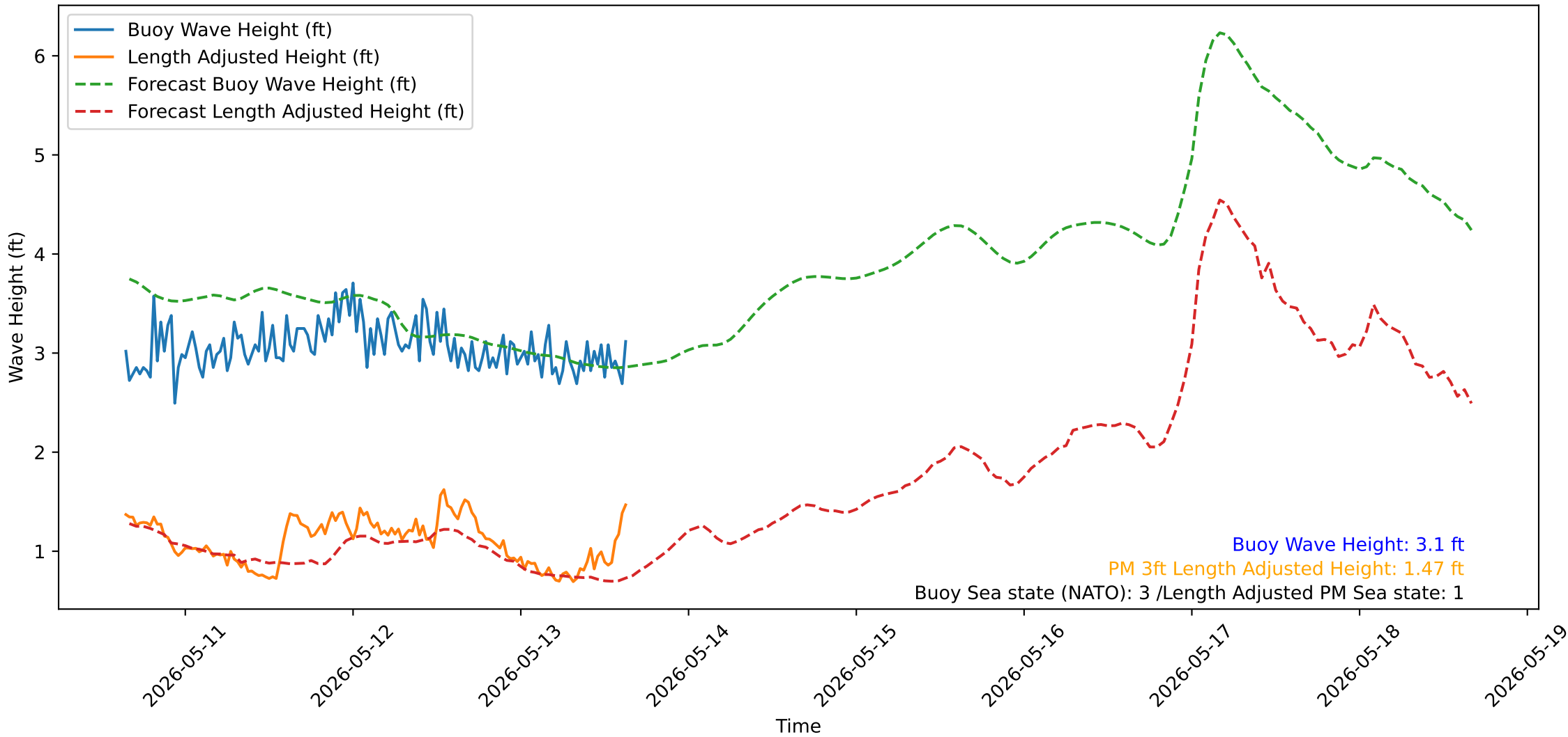
Wave Heights over Time for Oceanside Harbor at 2026-05-13 15:30:32
