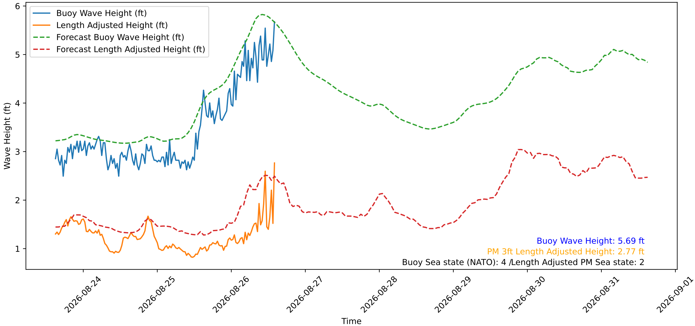
Wave Heights over Time for Green Beach at 2026-08-26 14:41:11
