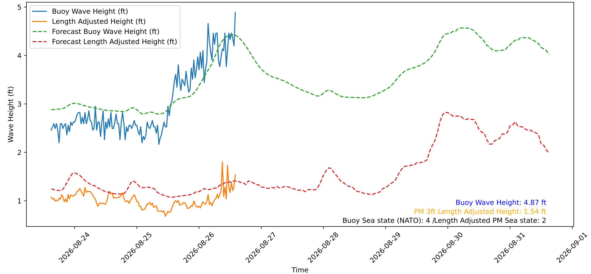
Wave Heights over Time for Red Beach at 2026-08-26 14:40:49
