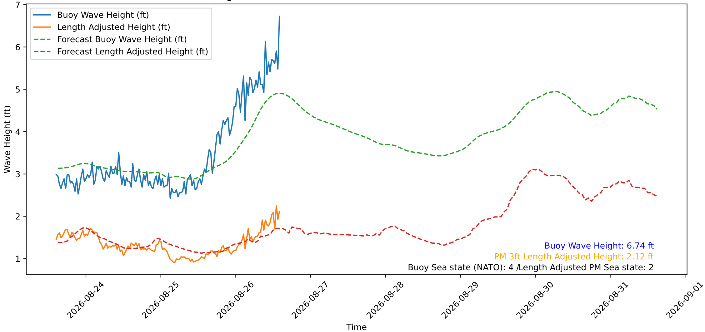
Wave Heights over Time for Oceanside Harbor at 2026-08-26 14:40:29
