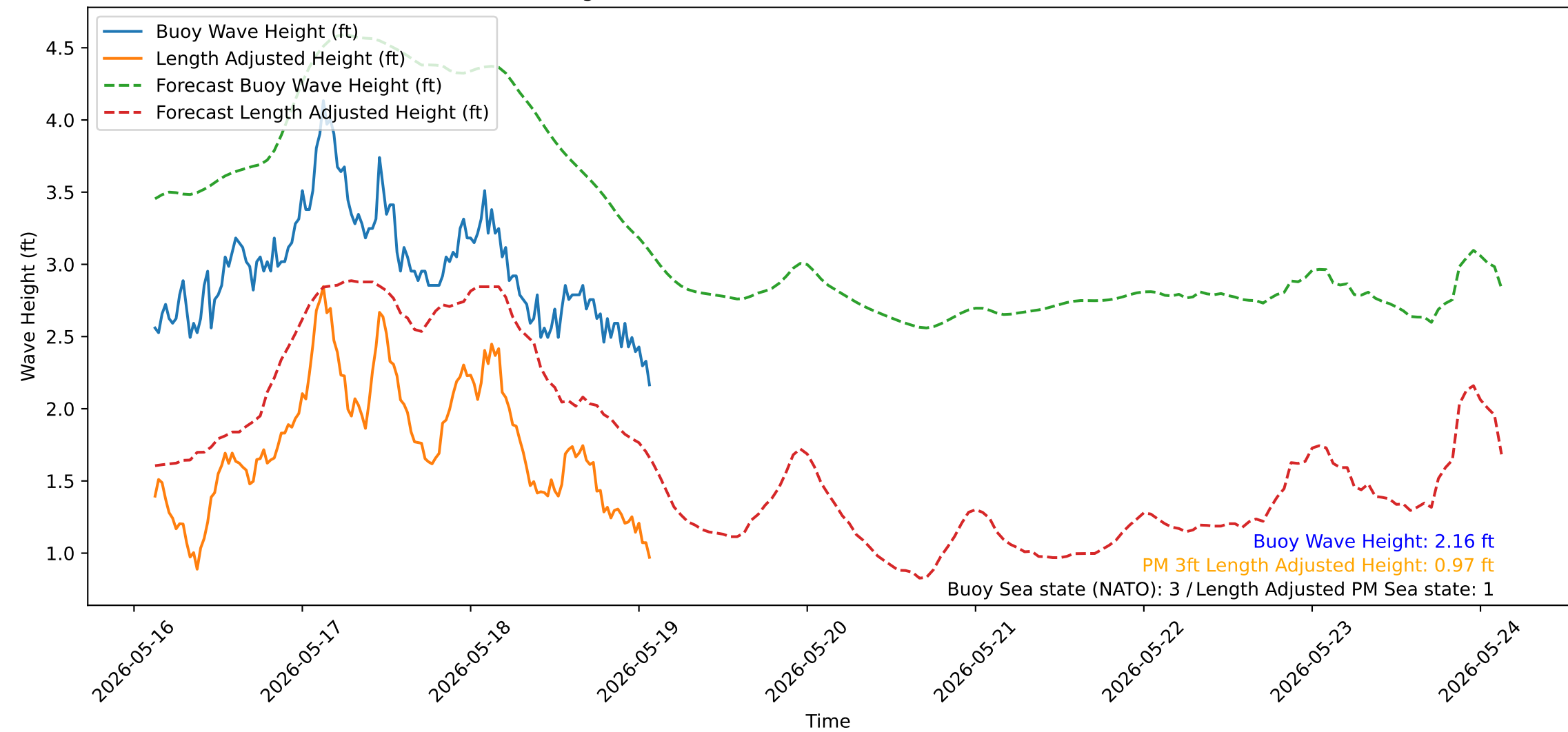
Wave Heights over Time for Red Beach at 2026-05-19 02:30:51
