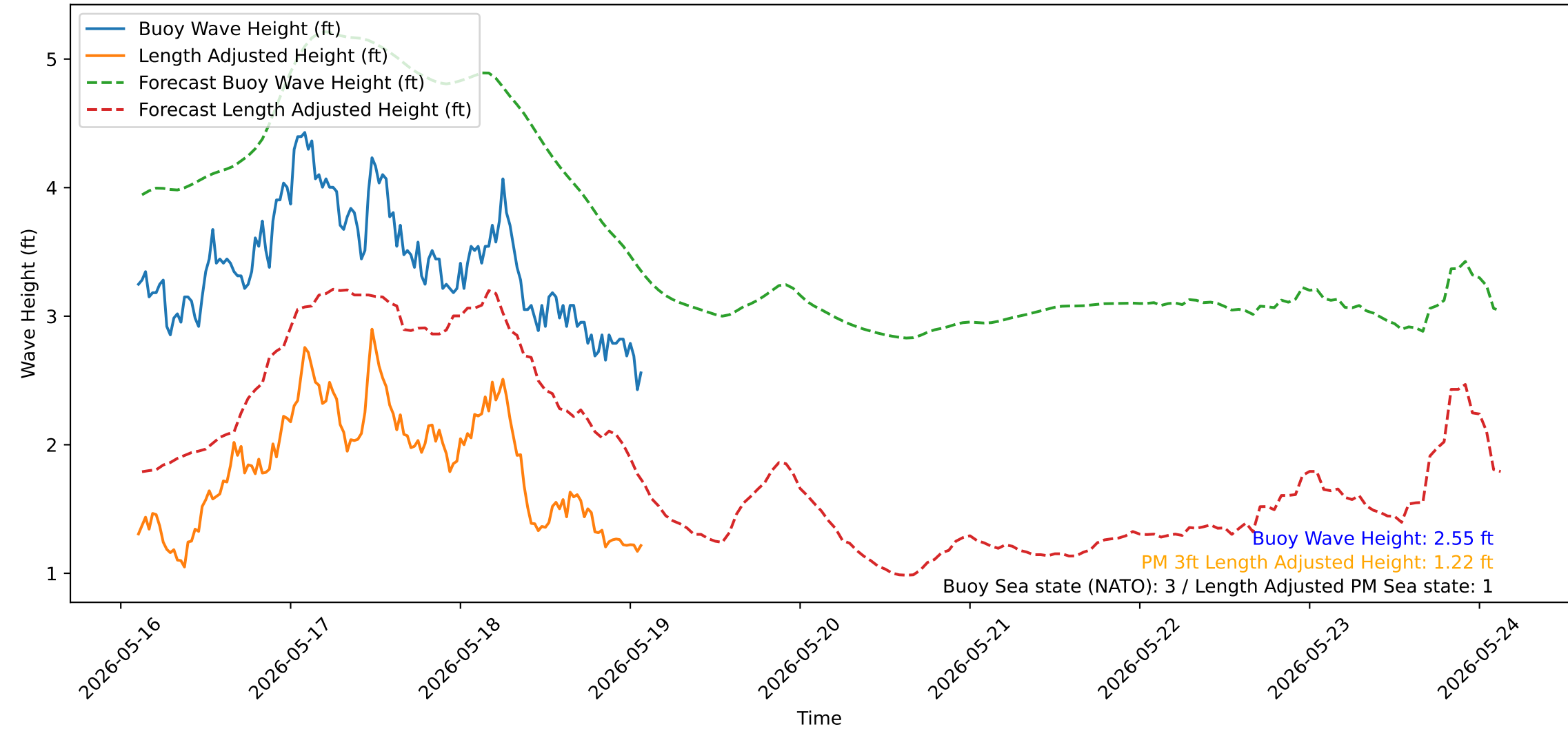
Wave Heights over Time for Green Beach at 2026-05-19 02:31:13
