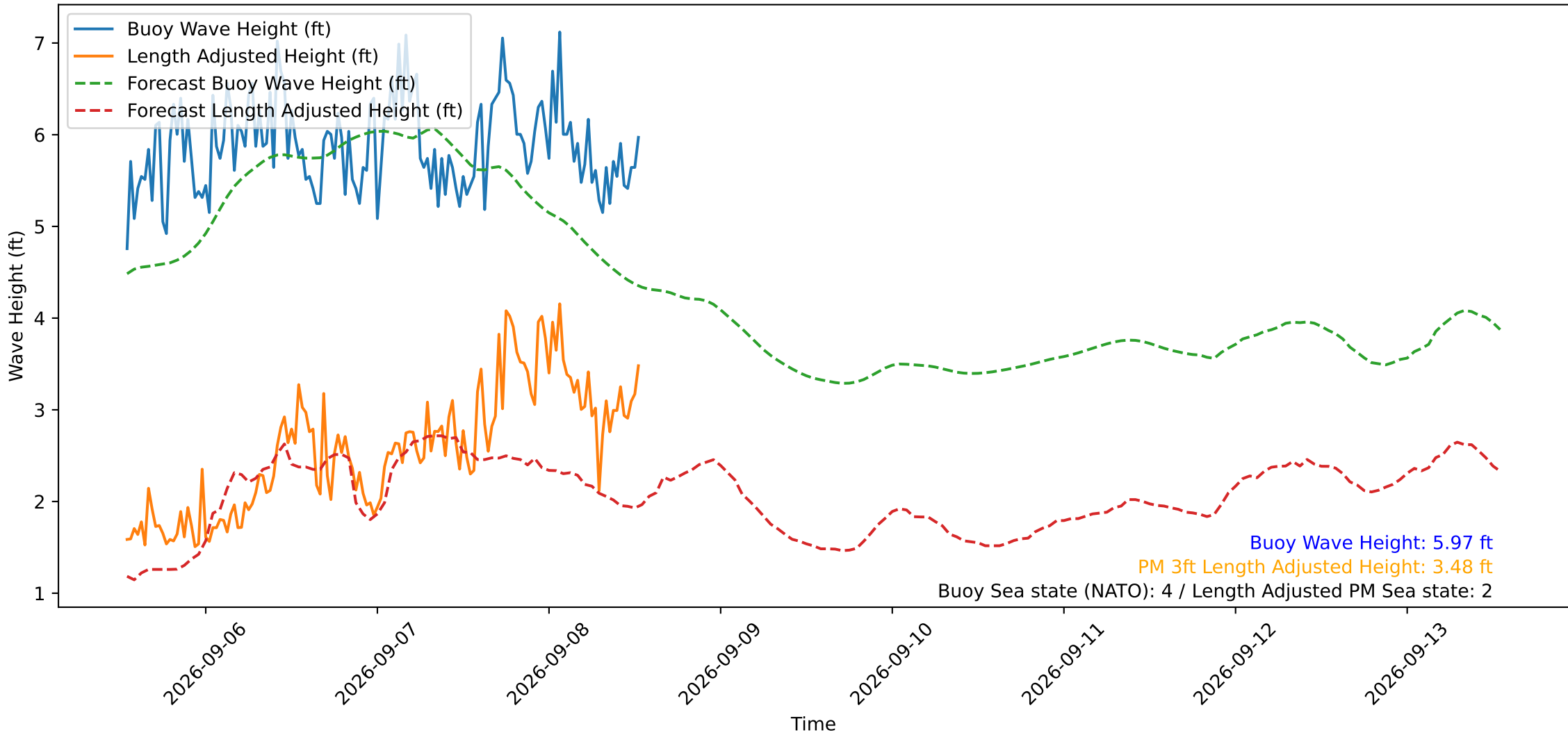
Wave Heights over Time for Oceanside Harbor at 2026-09-08 13:10:30
