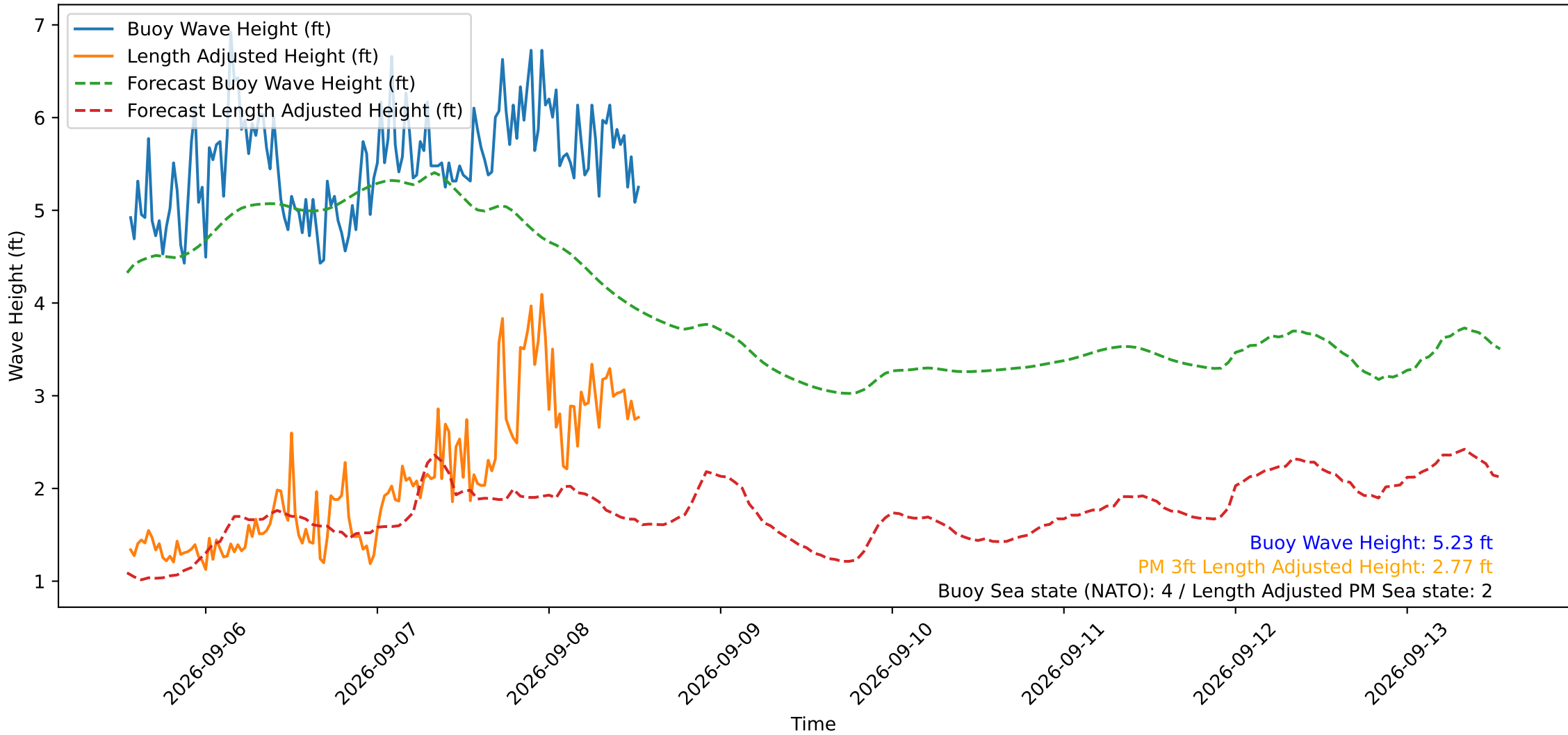
Wave Heights over Time for Red Beach at 2026-09-08 13:10:50
