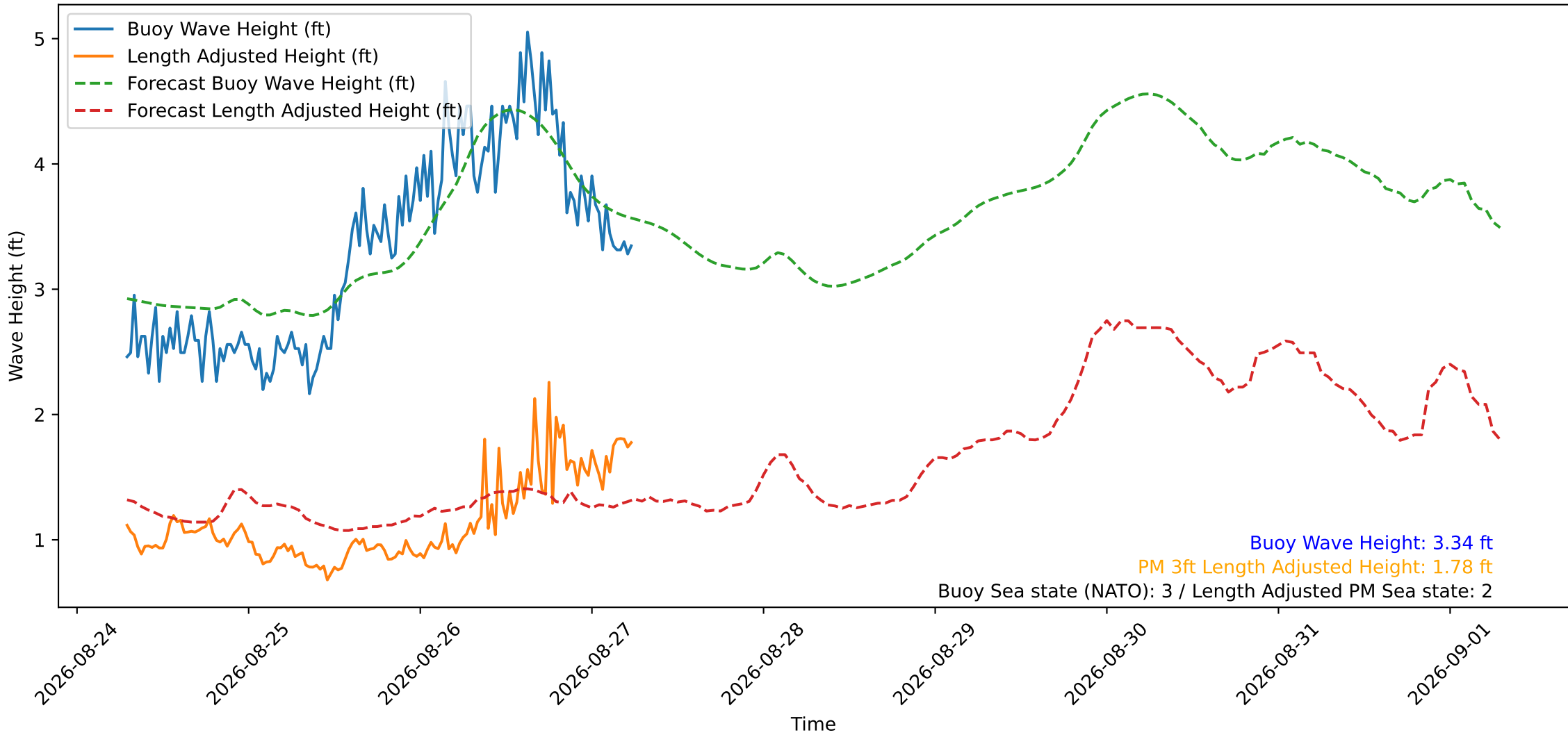
Wave Heights over Time for Red Beach at 2026-08-27 06:30:51
