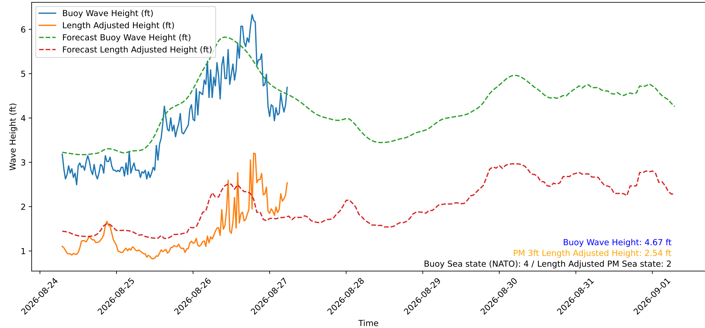
Wave Heights over Time for Green Beach at 2026-08-27 06:31:13
