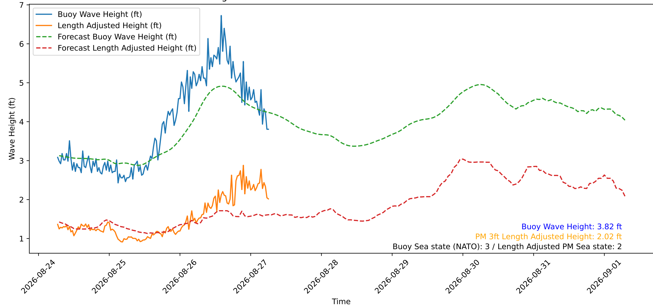
Wave Heights over Time for Oceanside Harbor at 2026-08-27 06:30:30
