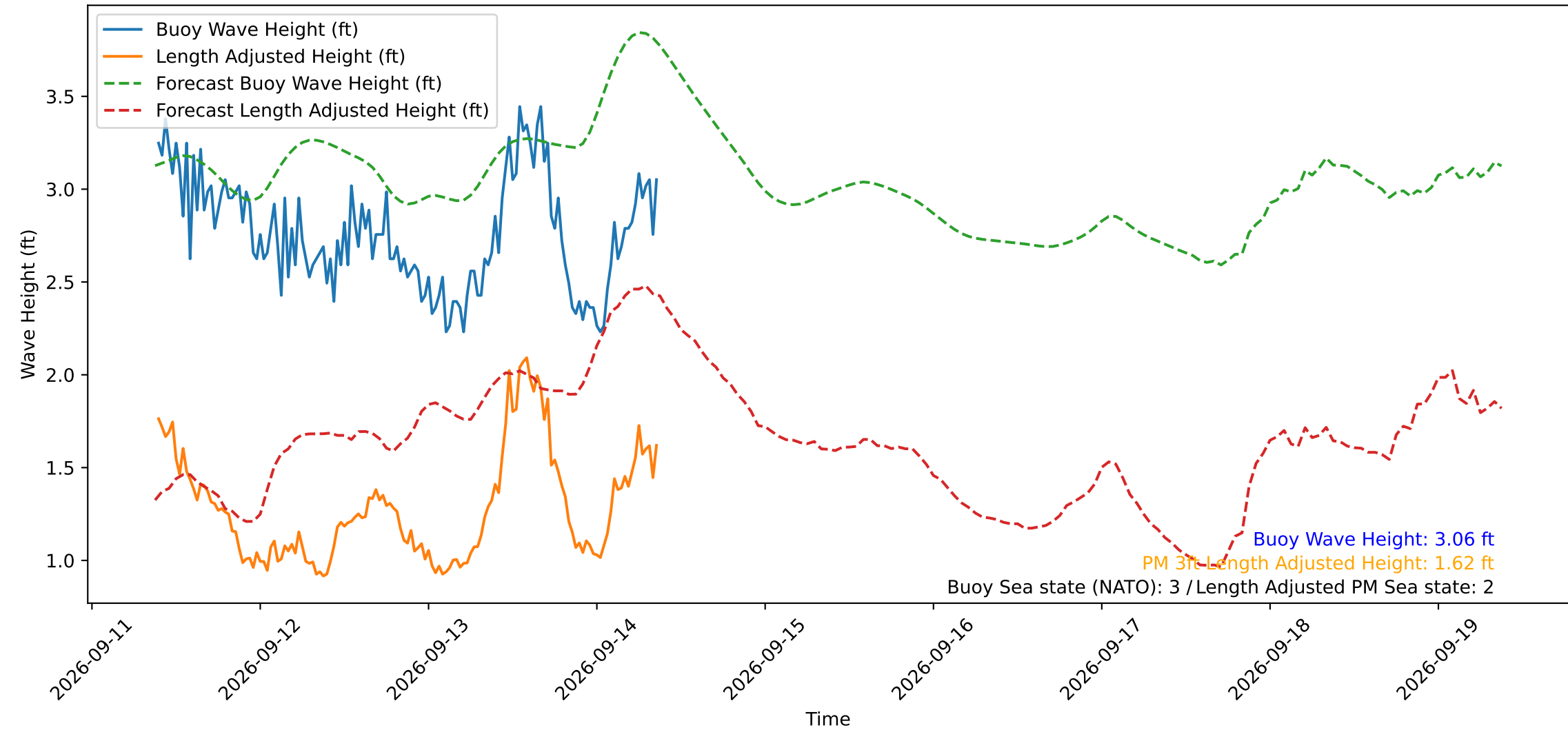
Wave Heights over Time for Red Beach at 2026-09-14 09:20:50
