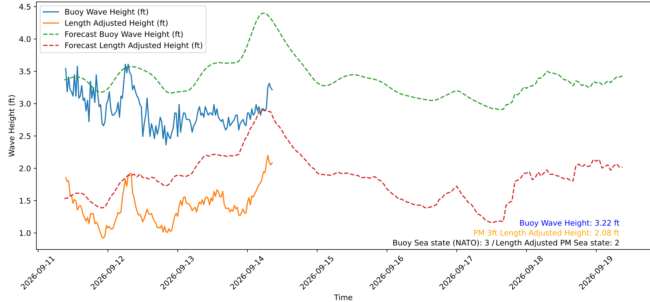
Wave Heights over Time for Green Beach at 2026-09-14 09:21:13
