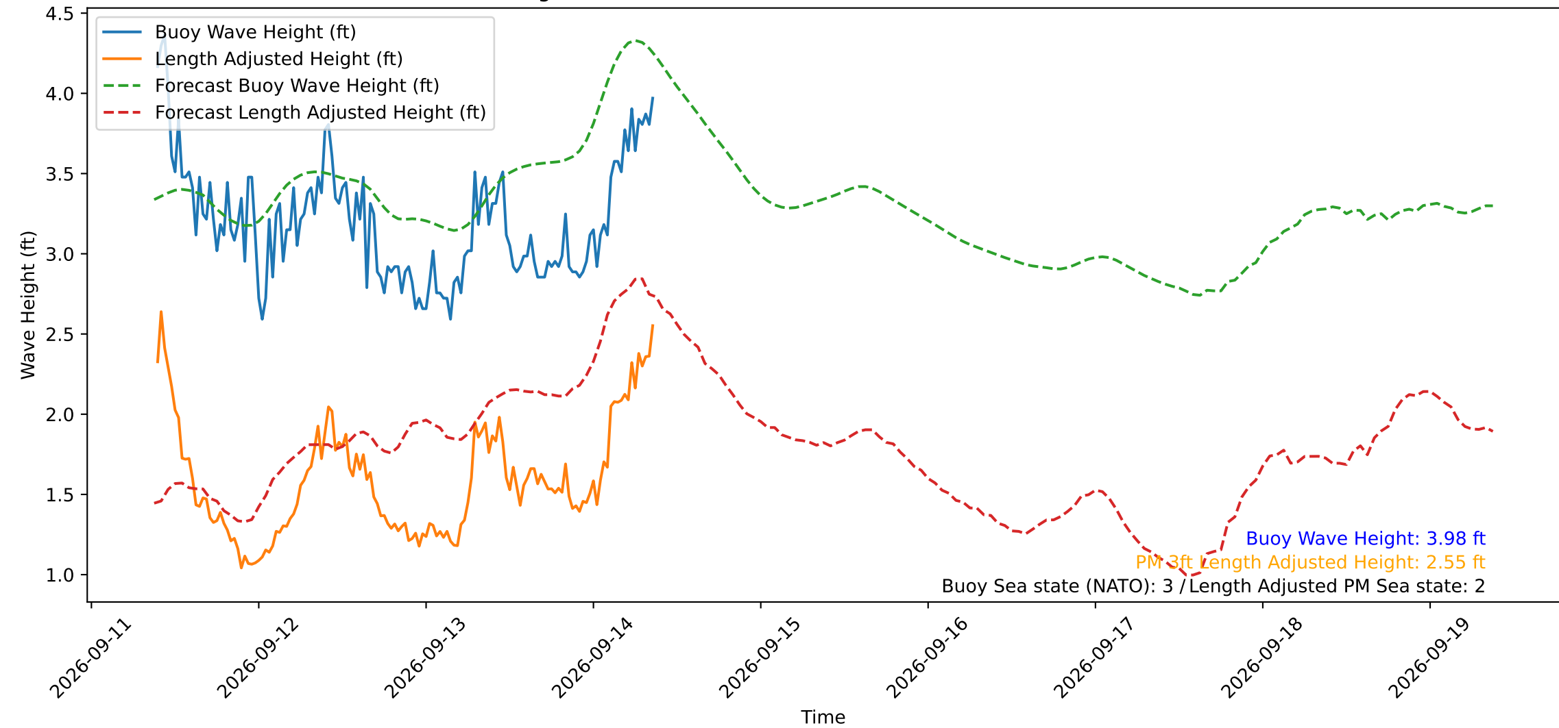
Wave Heights over Time for Oceanside Harbor at 2026-09-14 09:20:29
