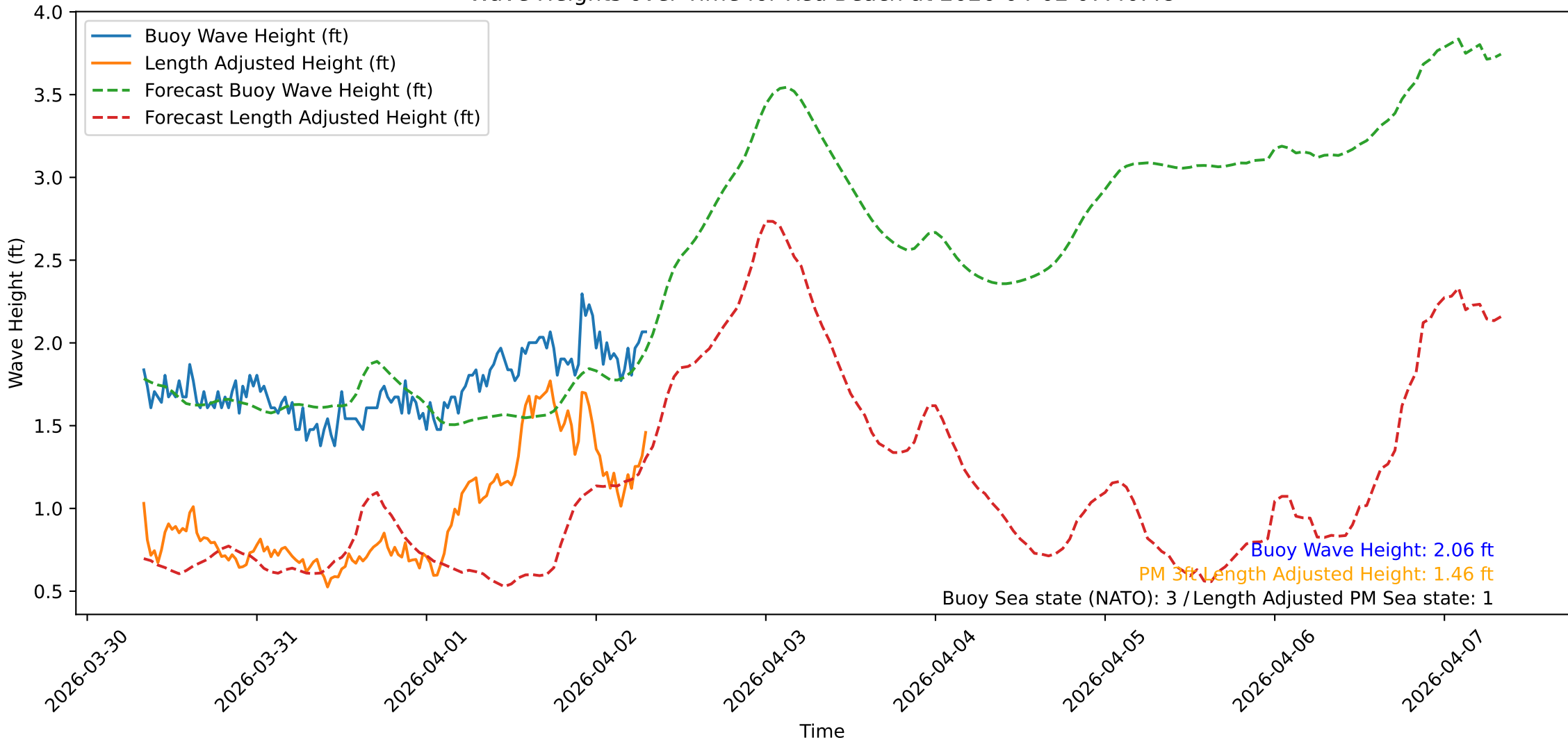
Wave Heights over Time for Red Beach at 2026-04-02 07:40:48
