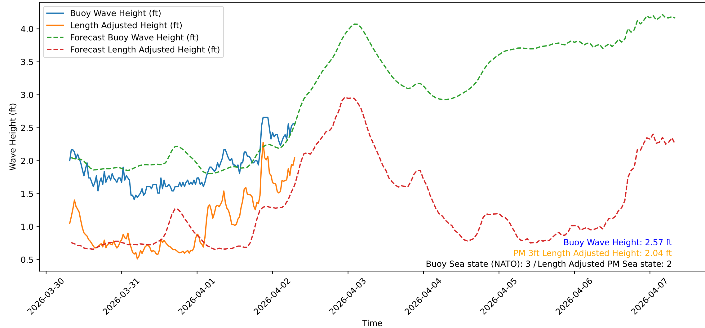
Wave Heights over Time for Green Beach at 2026-04-02 07:41:11
