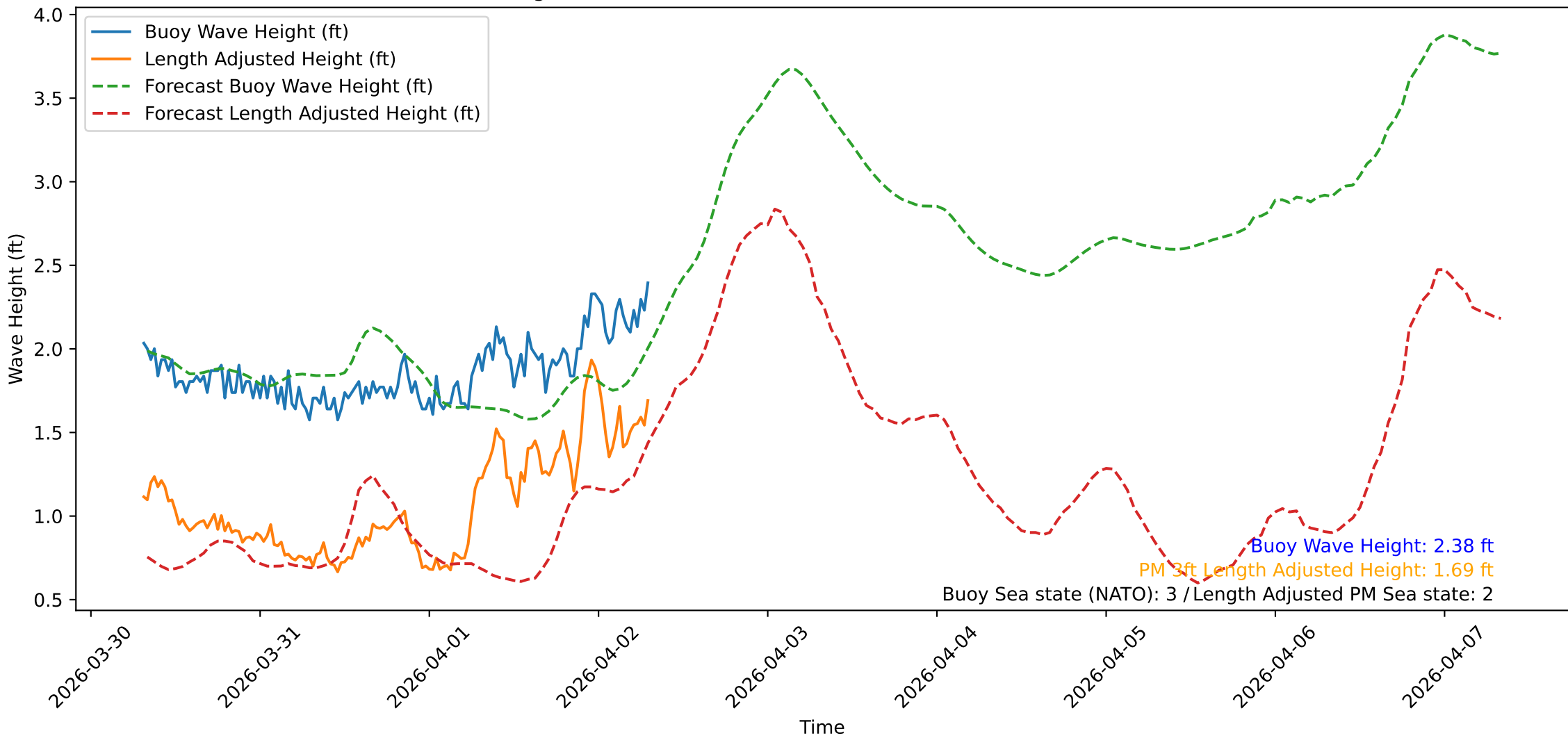
Wave Heights over Time for Oceanside Harbor at 2026-04-02 07:40:32
